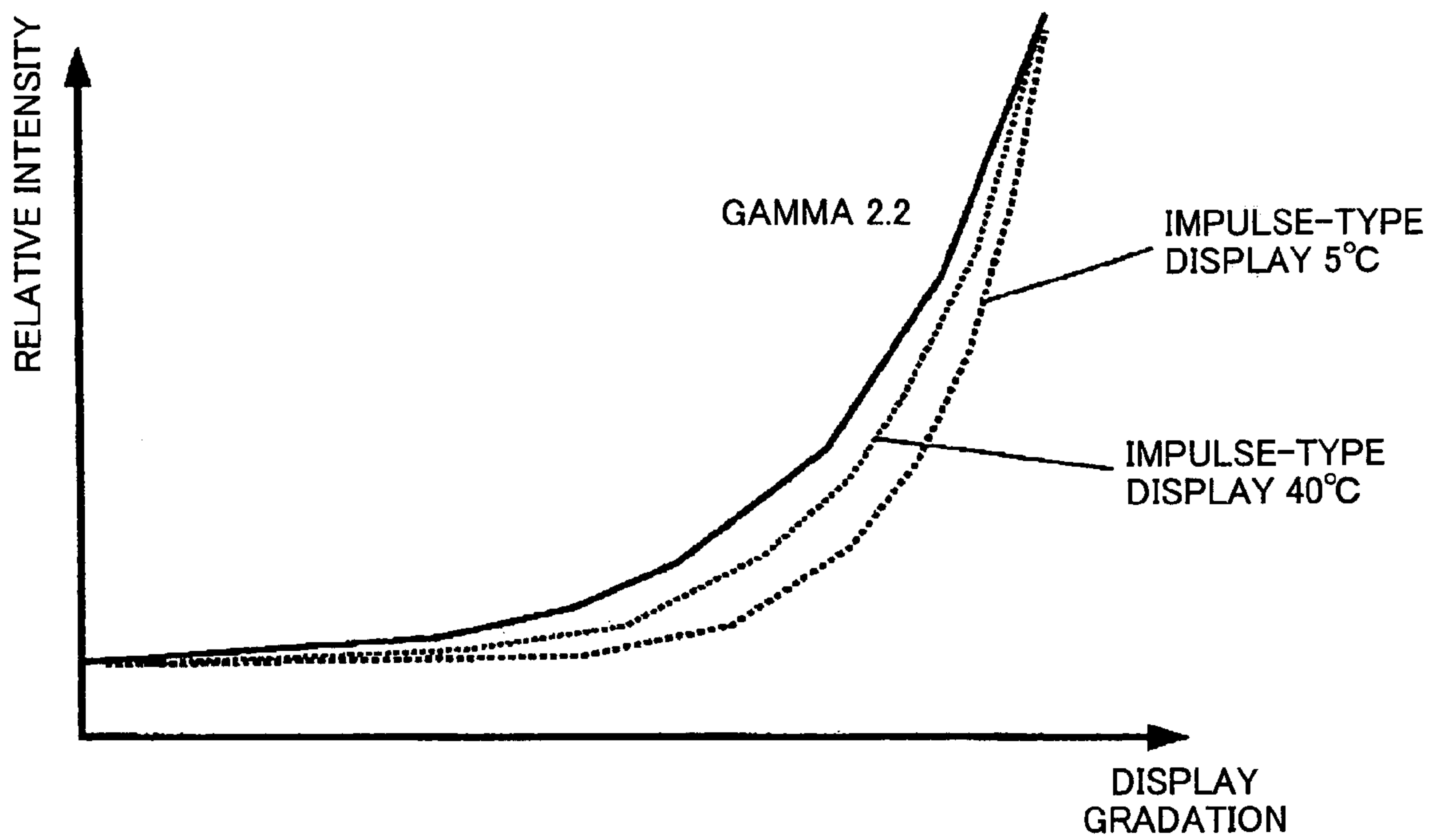
GAMMA CHARACTERISTICS OF LIQUID CRYSTAL DISPLAY
