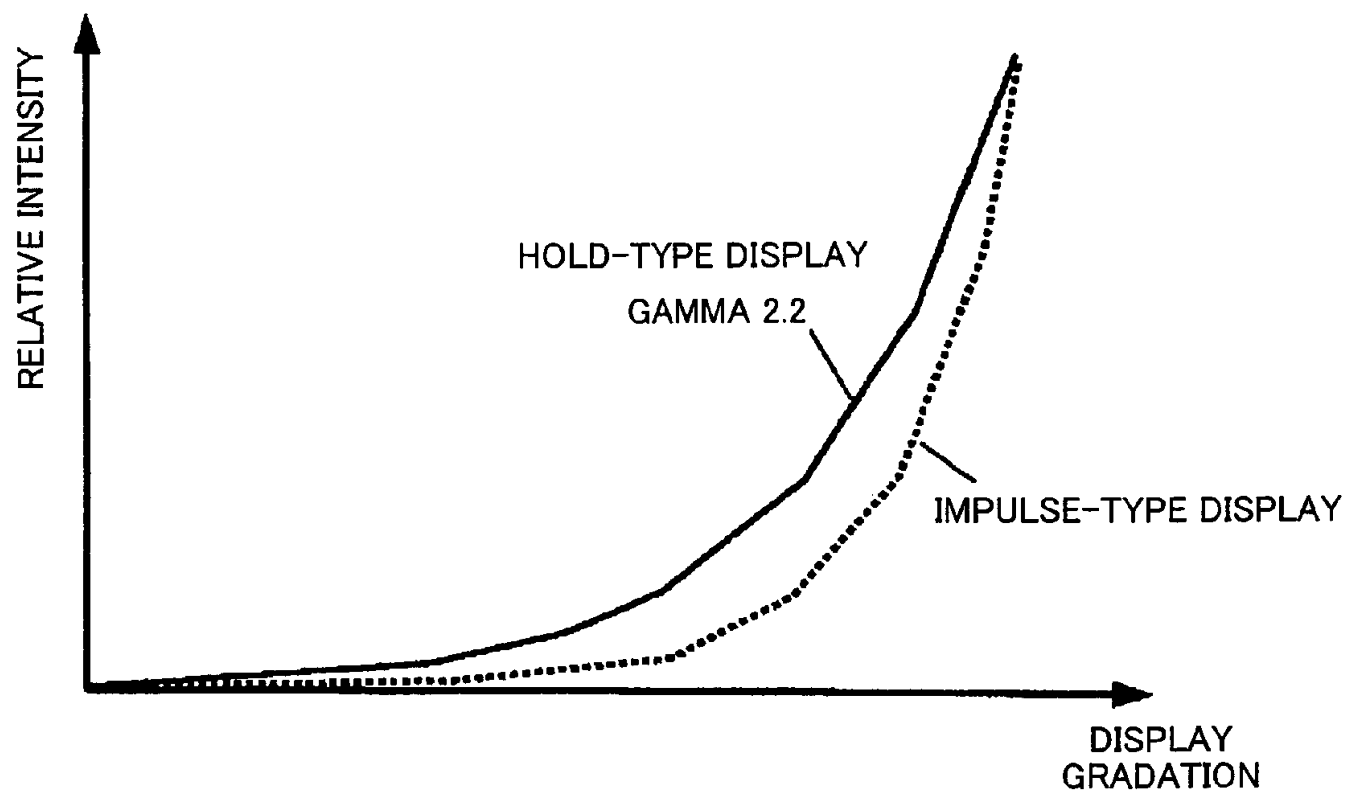
GAMMA CHARACTERISTICS OF LIQUID CRYSTAL DISPLAY
