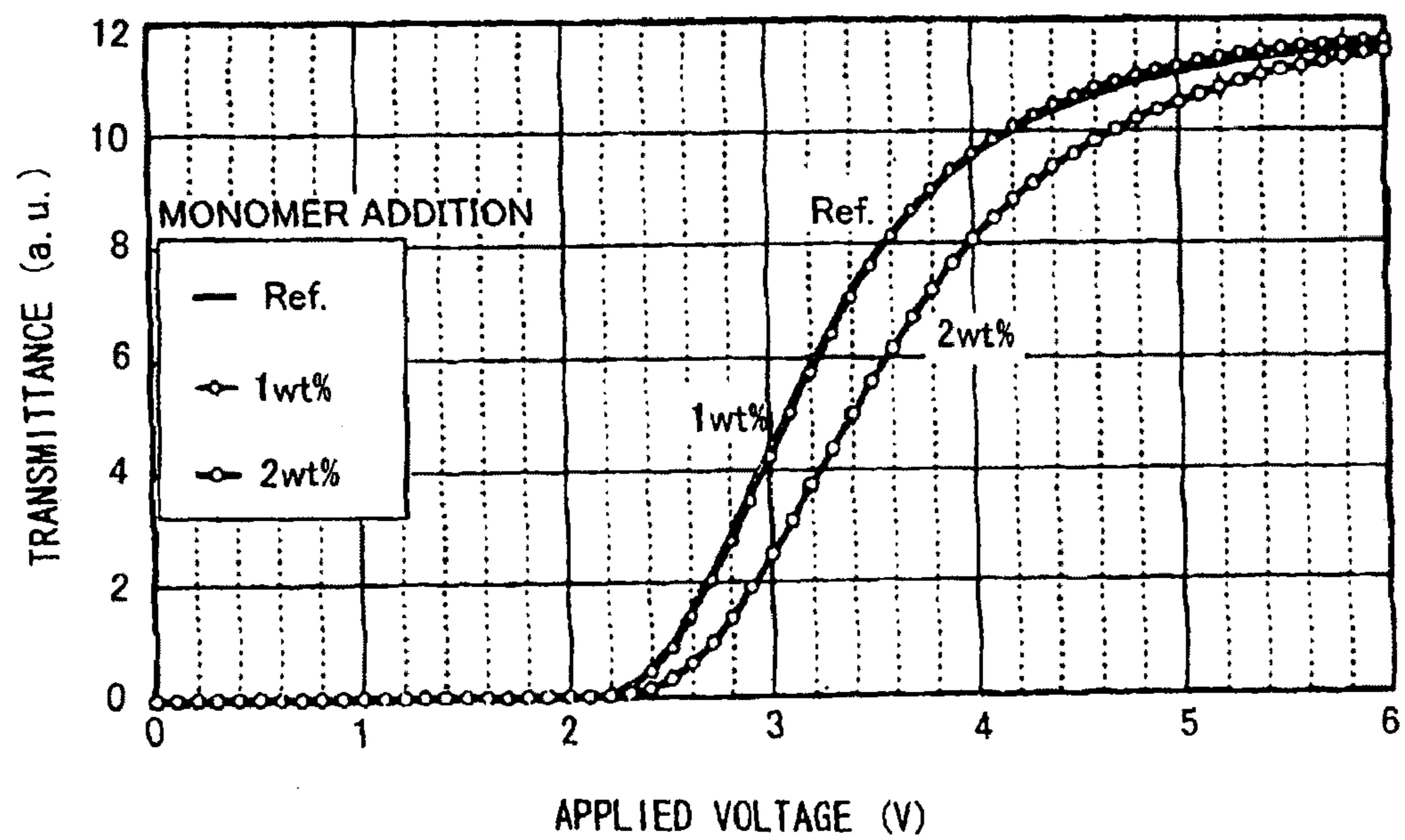
FIG. 37 ADDITION OF MONOFUNCTIONAL MONOMER
