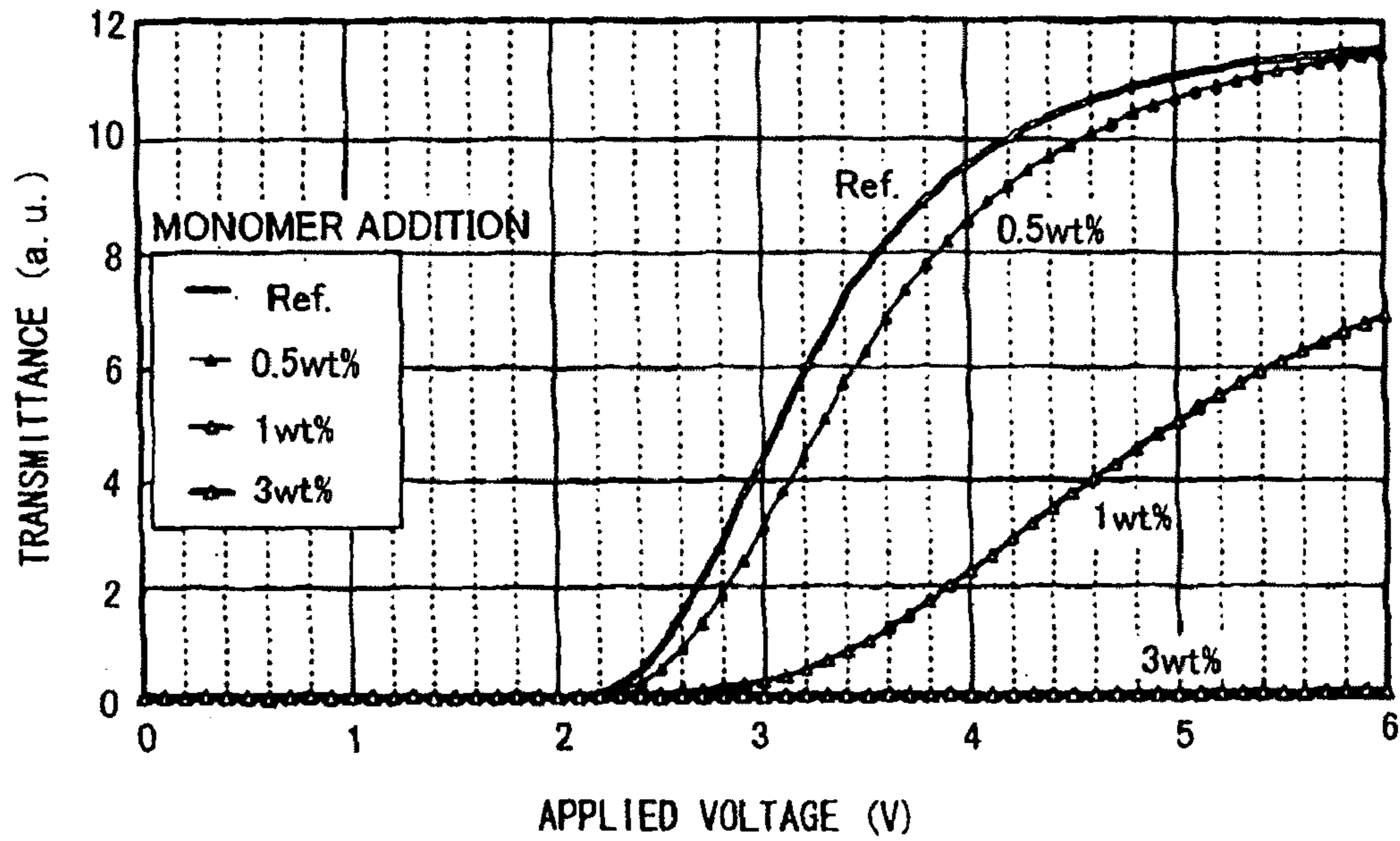
FIG. 36 ADDITION OF BIFUNCTIONAL MONOMER
