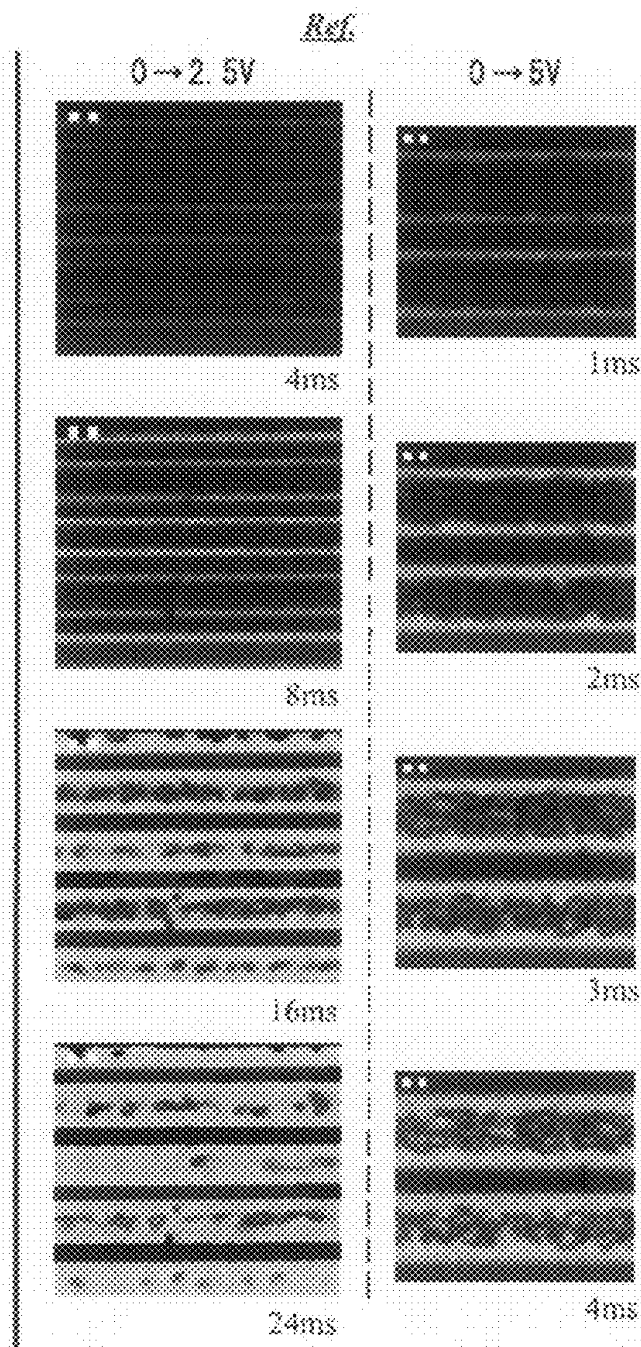
FIG. 39 COMPARATIVE EXAMPLE: LIQUID CRYSTAL DISPLAY APPARATUS WHEREIN NO POLYMERIZABLE COMPONENT IS ADDED TO THE LIQUID CRYSTAL
