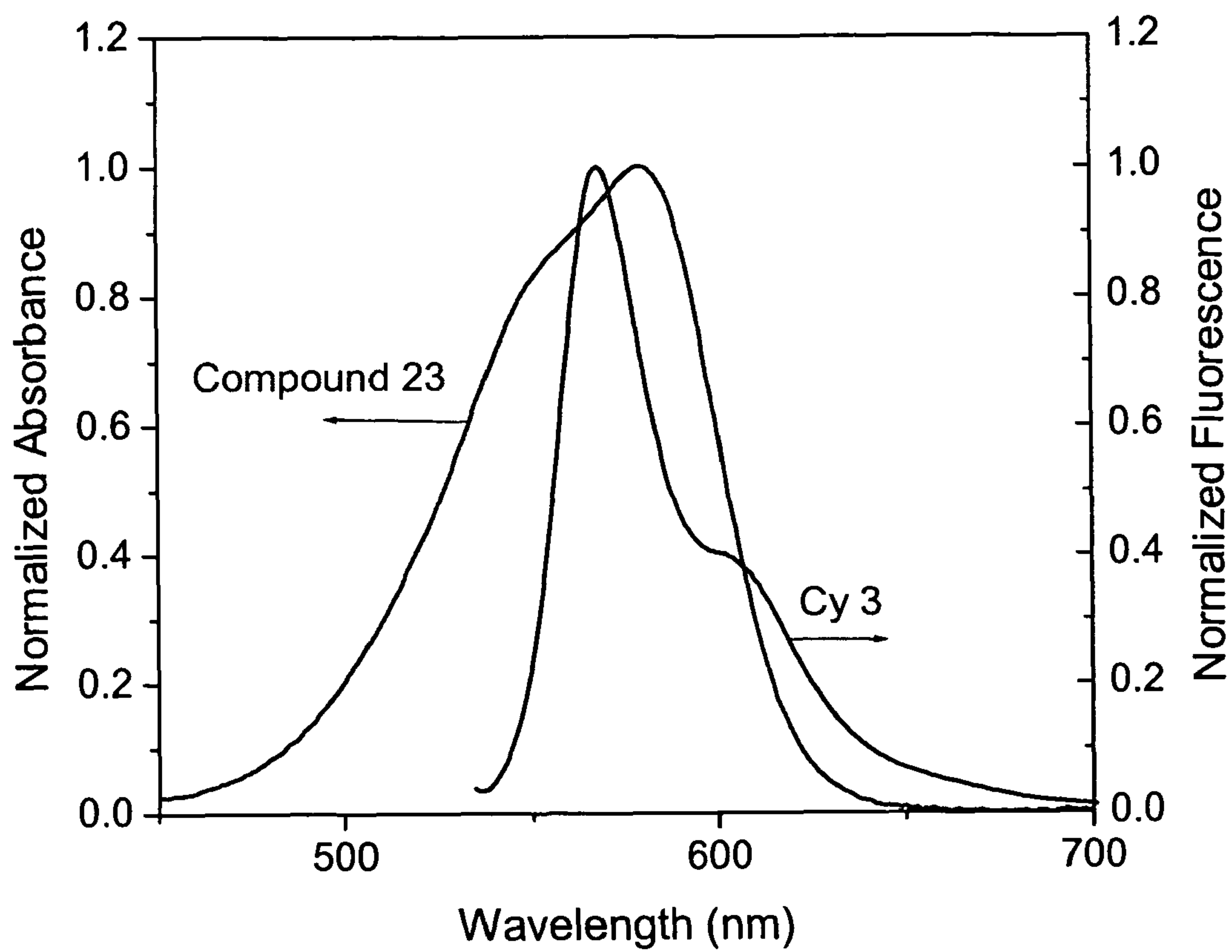
FIG. 9. Spectral overlap of compound 23 with Cy3
