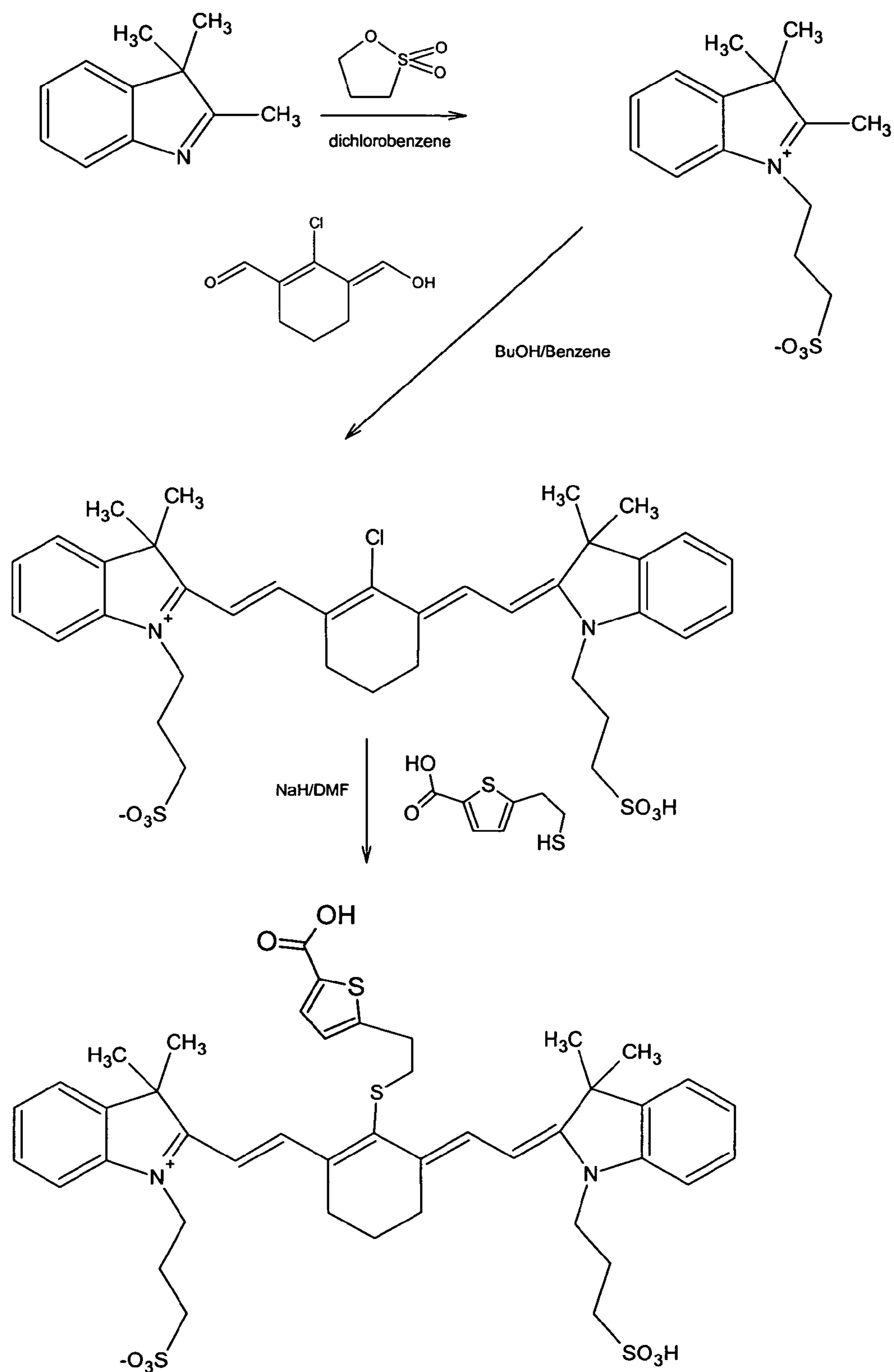
FIG. 6. Synthesis of a cyanine that has a LQM at the BRIDGE atoms
