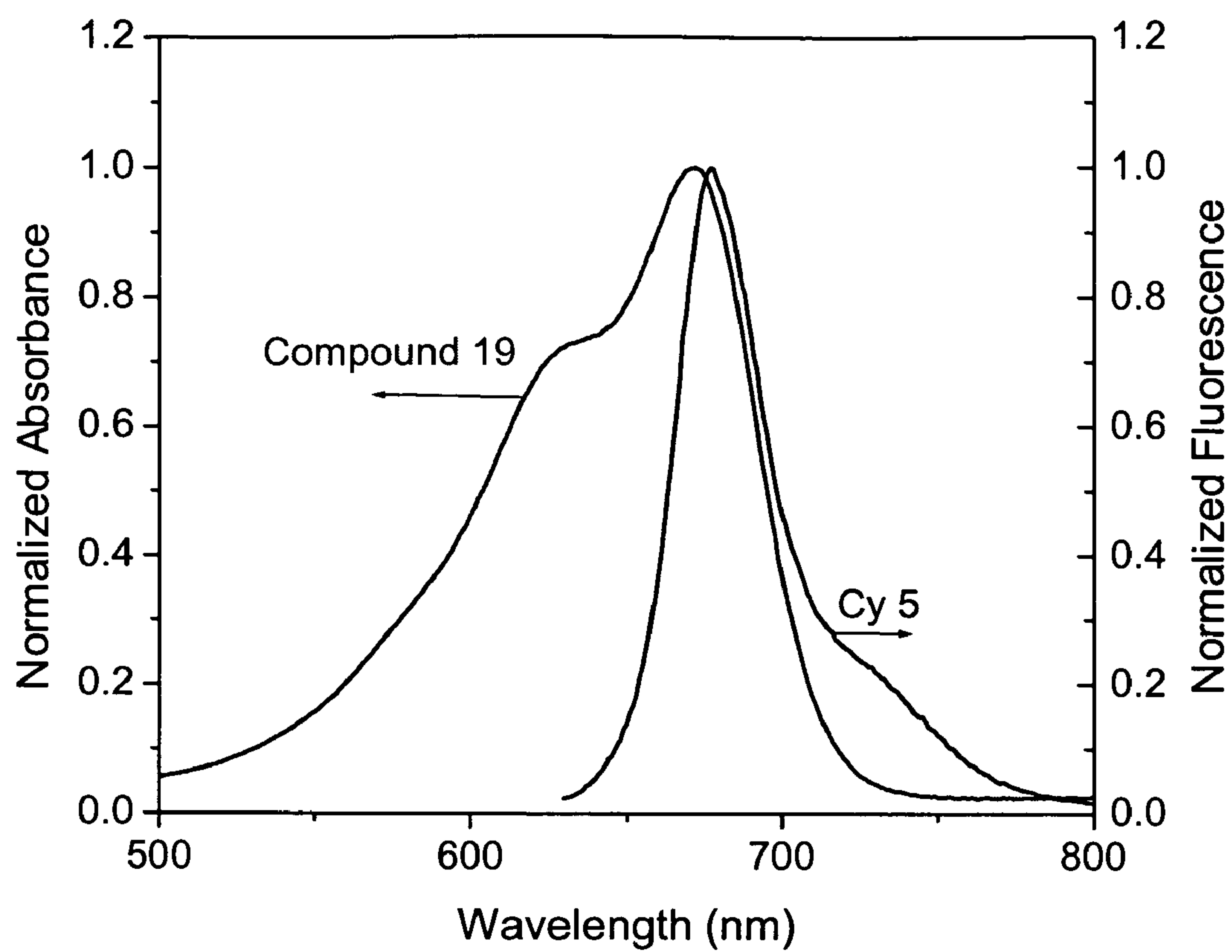
FIG. 10. Spectral overlap of compound 19 with Cy5.
