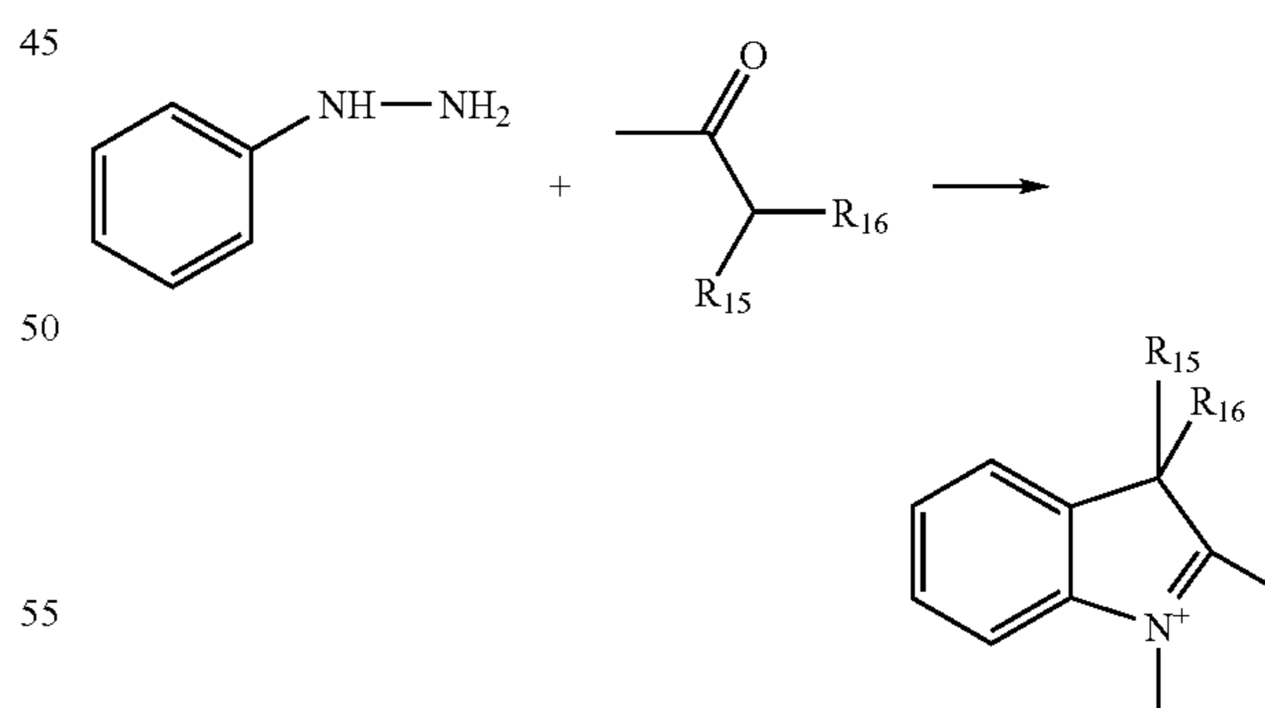
Scheme 1. Typical synthesis of indolium intermediates
