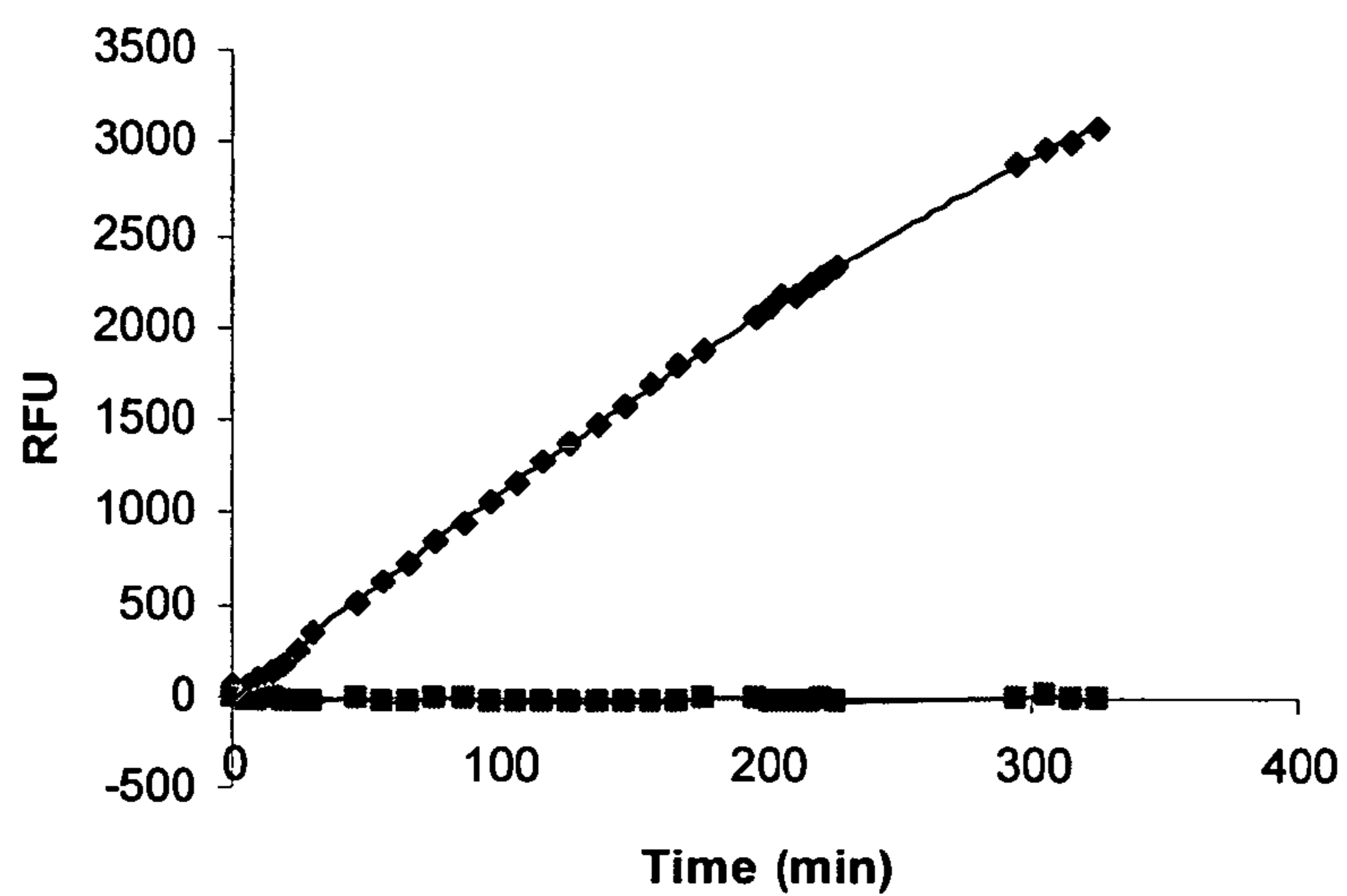
FIG. 11. MMP-2 cleavage of Compound 19-Lys-Pro-Leu-Ala-Nva-Asp(Cy5)-Ala-Arg-NH 2 .
