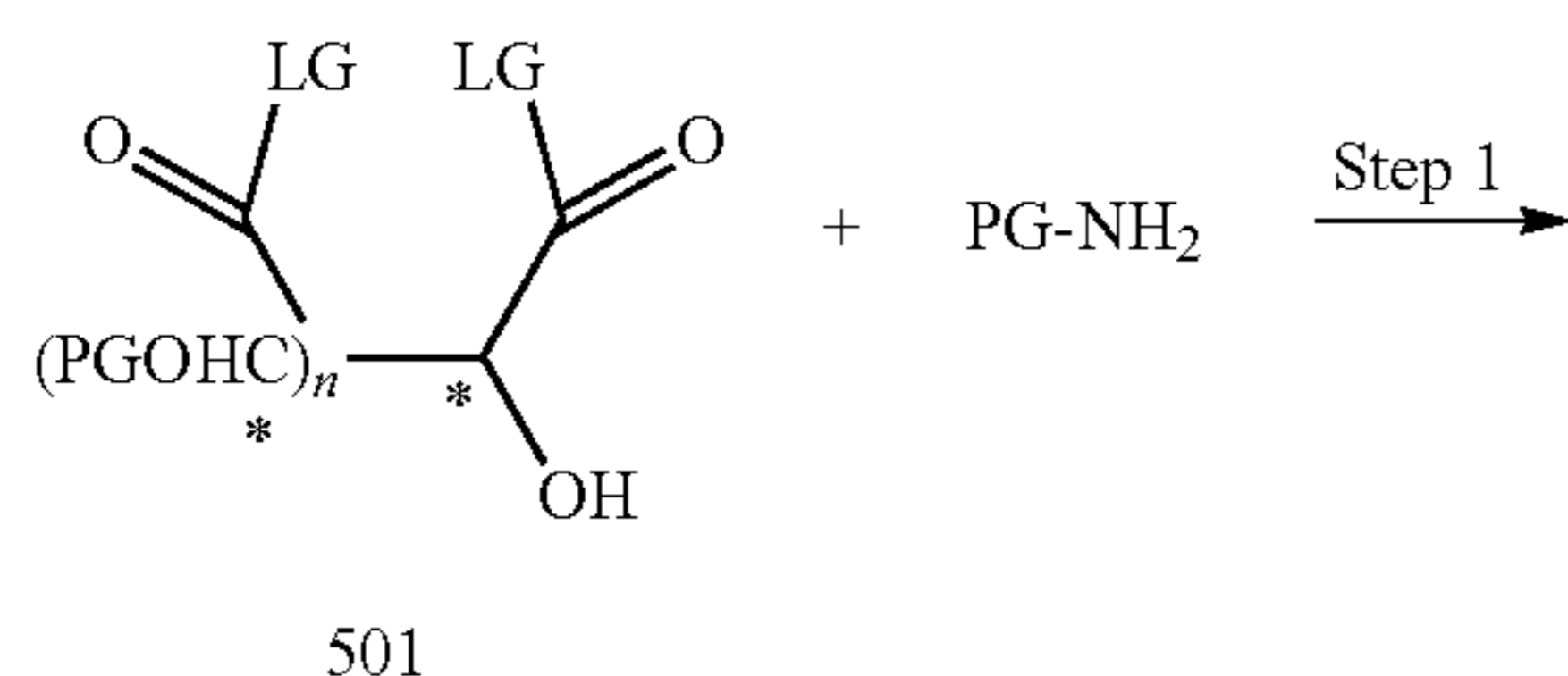
REACTION SCHEME 5
