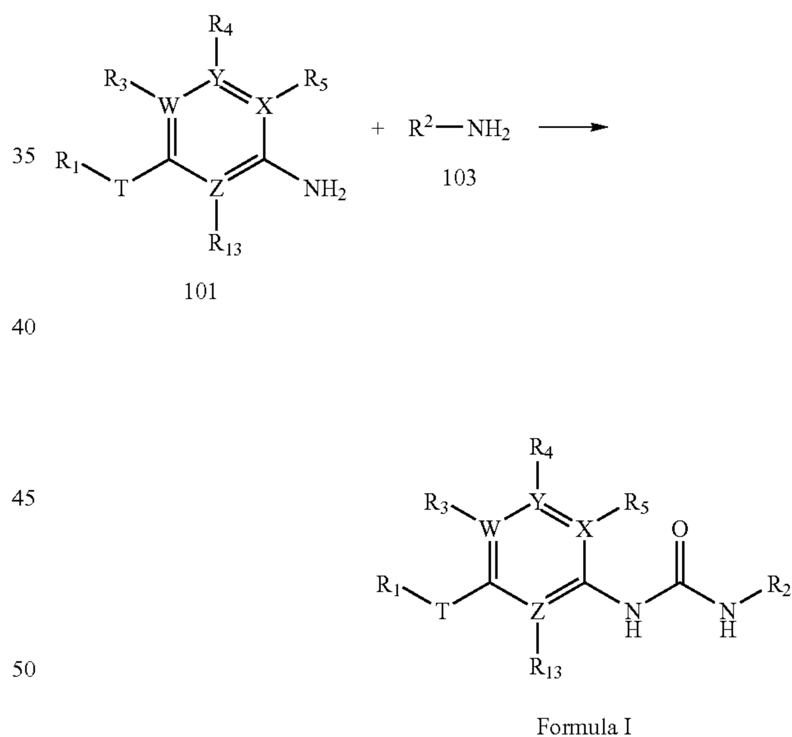
REACTION SCHEME 1
