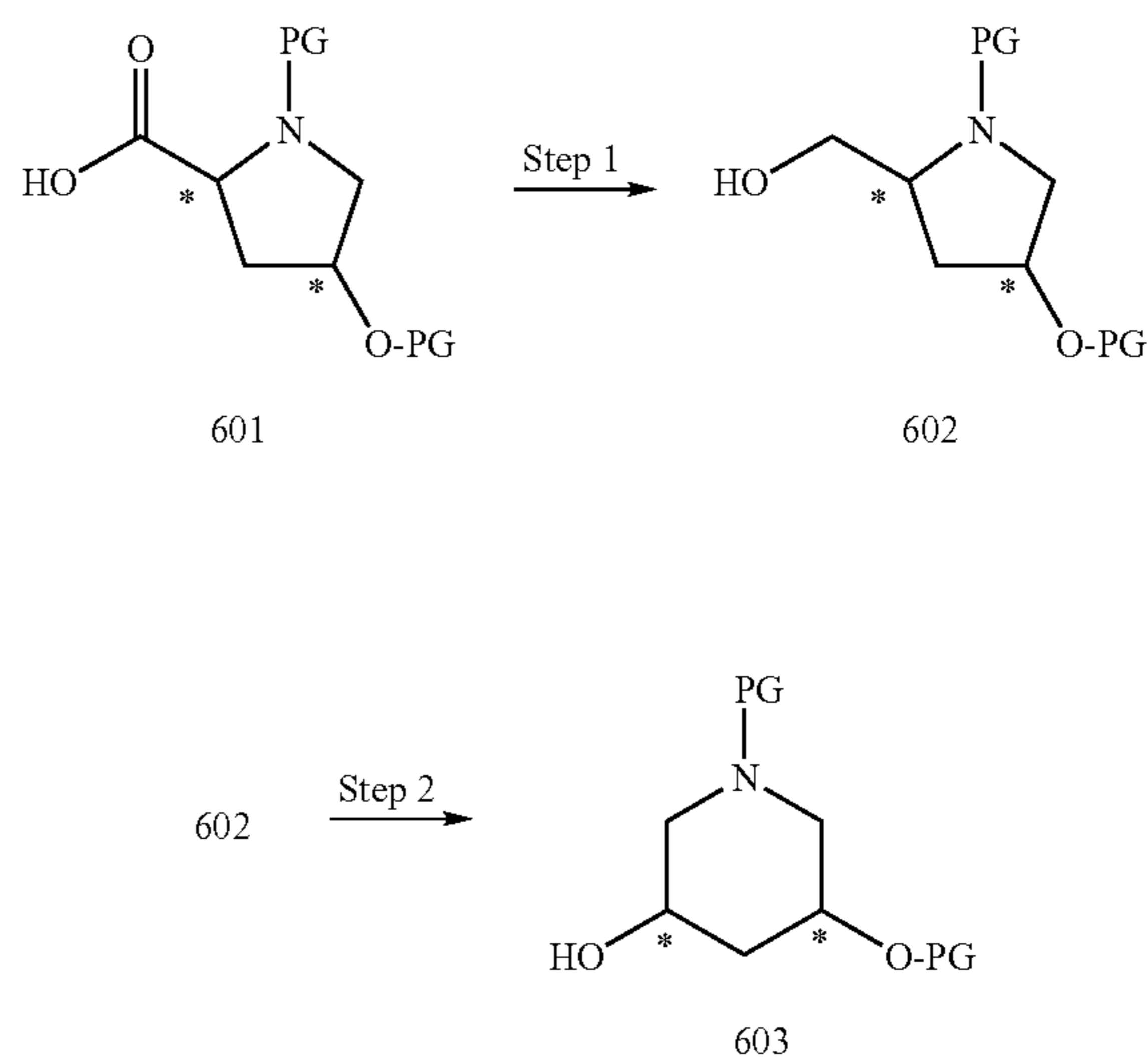
REACTION SCHEME 6
