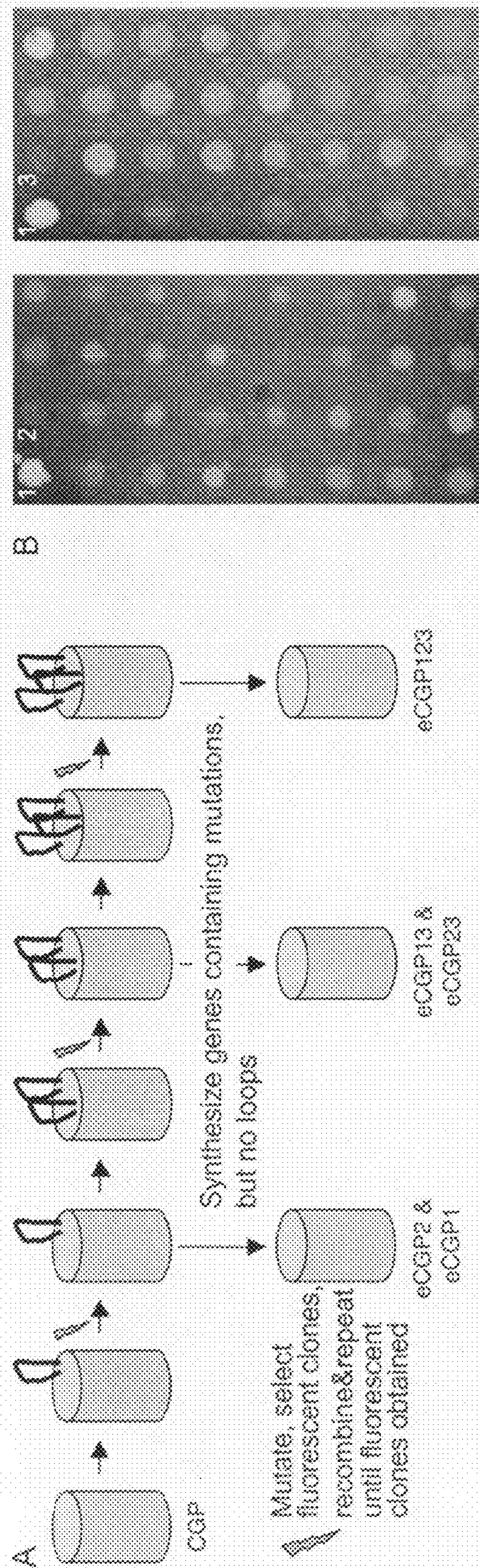
Figure 1: evolutionary strategy
