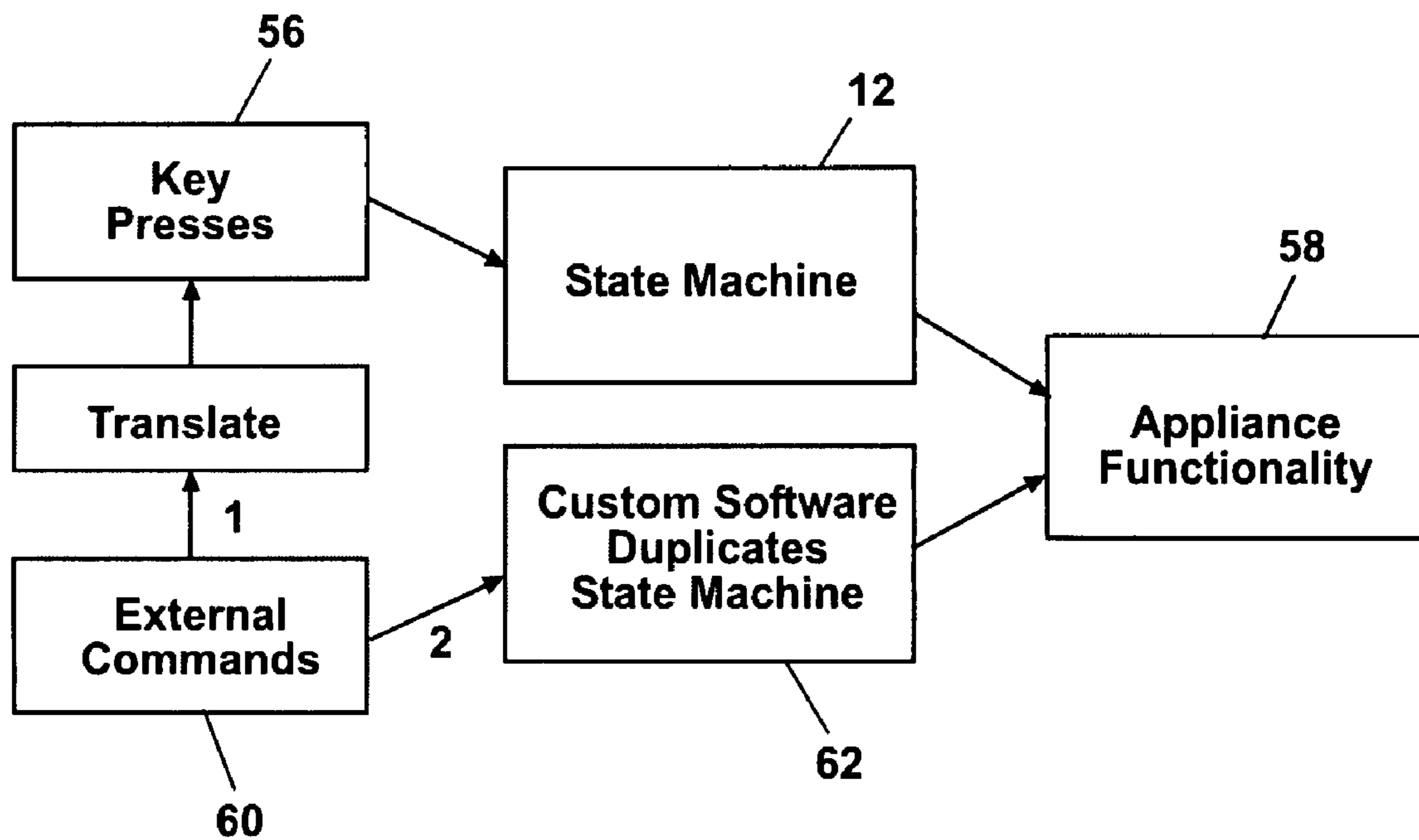
Fig. 16 (PRIOR ART)
