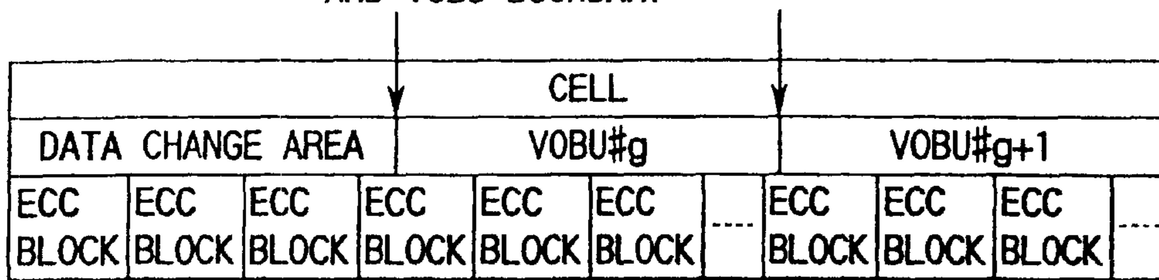
POSITIONS OF SHIFT PRODUCED BETWEEN ECC BLOCK BOUNDARY AND VOBU BOUNDARY
