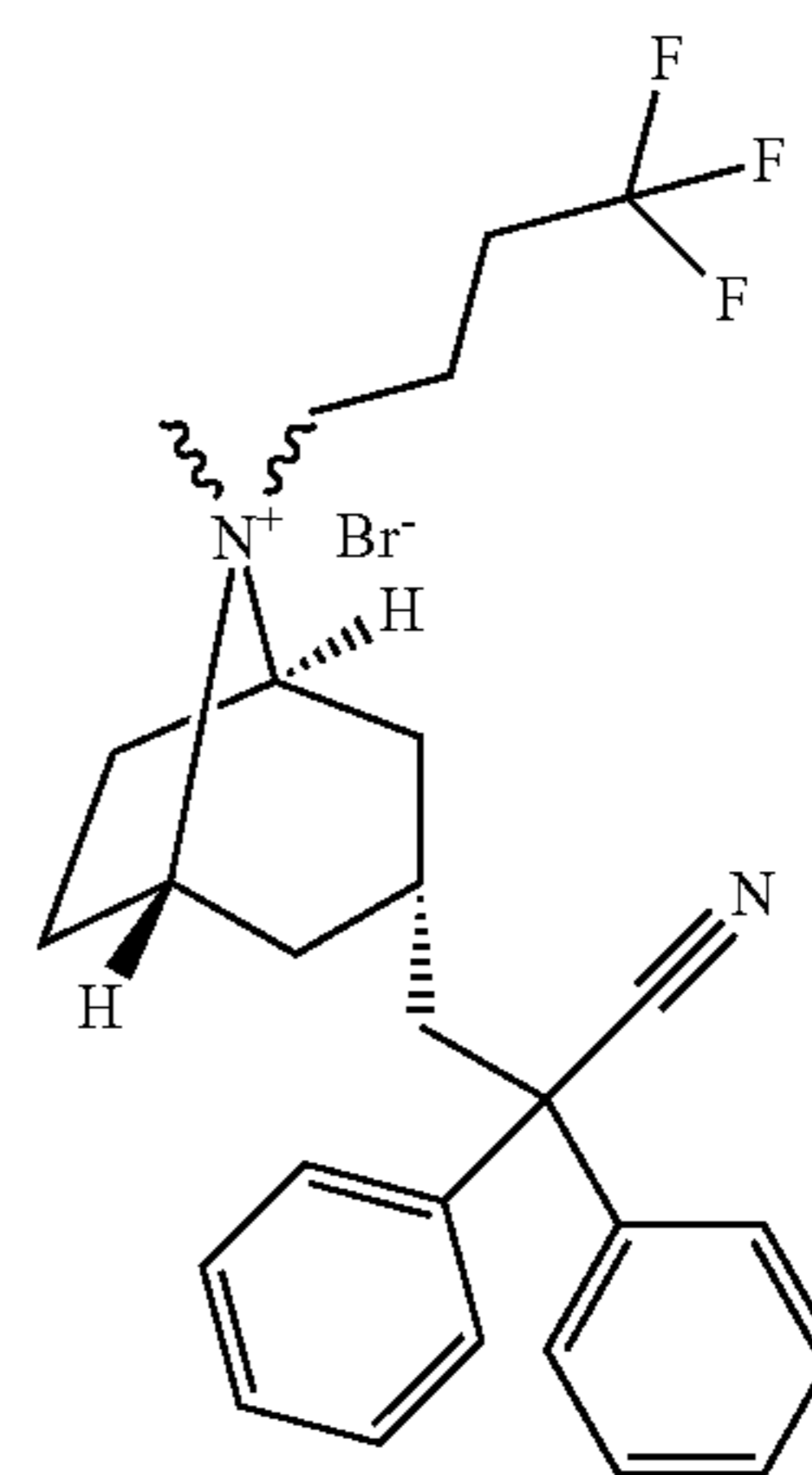
(3-endo)-3-(2-cyano-2,2-diphenylethyl)-8-methyl-8-(4,4,4-trifluorobutyl)-8-azoniabicyclo[3.2.1]octane bromide
