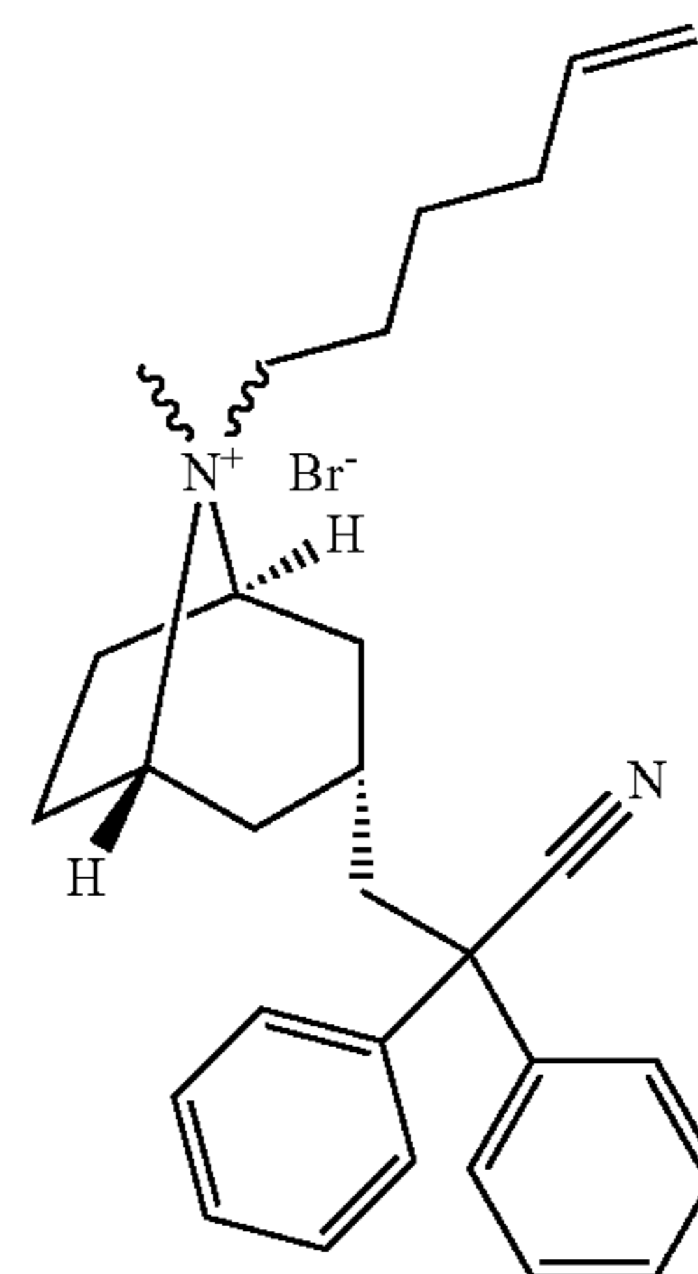
(3-endo)-3-(2-cyano-2,2-diphenylethyl)-8-(5-hexen-1-yl)-8-methyl-8-azoniabicyclo[3.2.1]octane bromide
