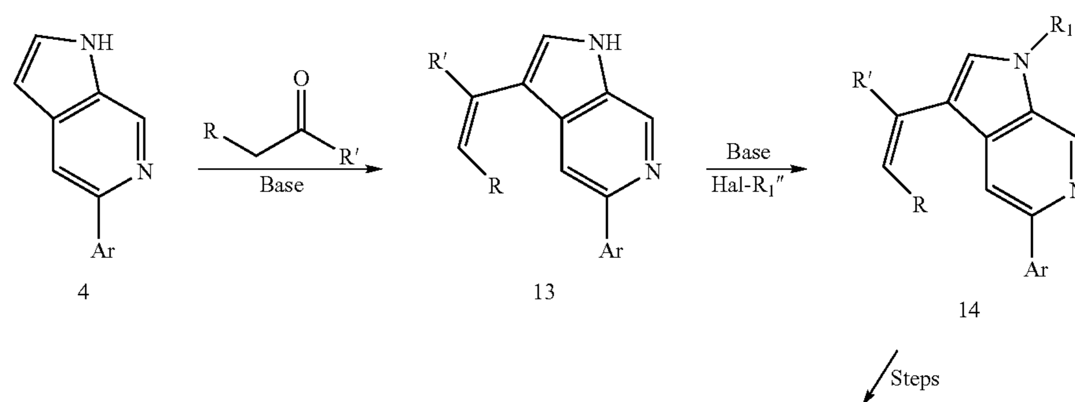
Scheme 6 Preparation of compounds of Formula I or Formula II.
