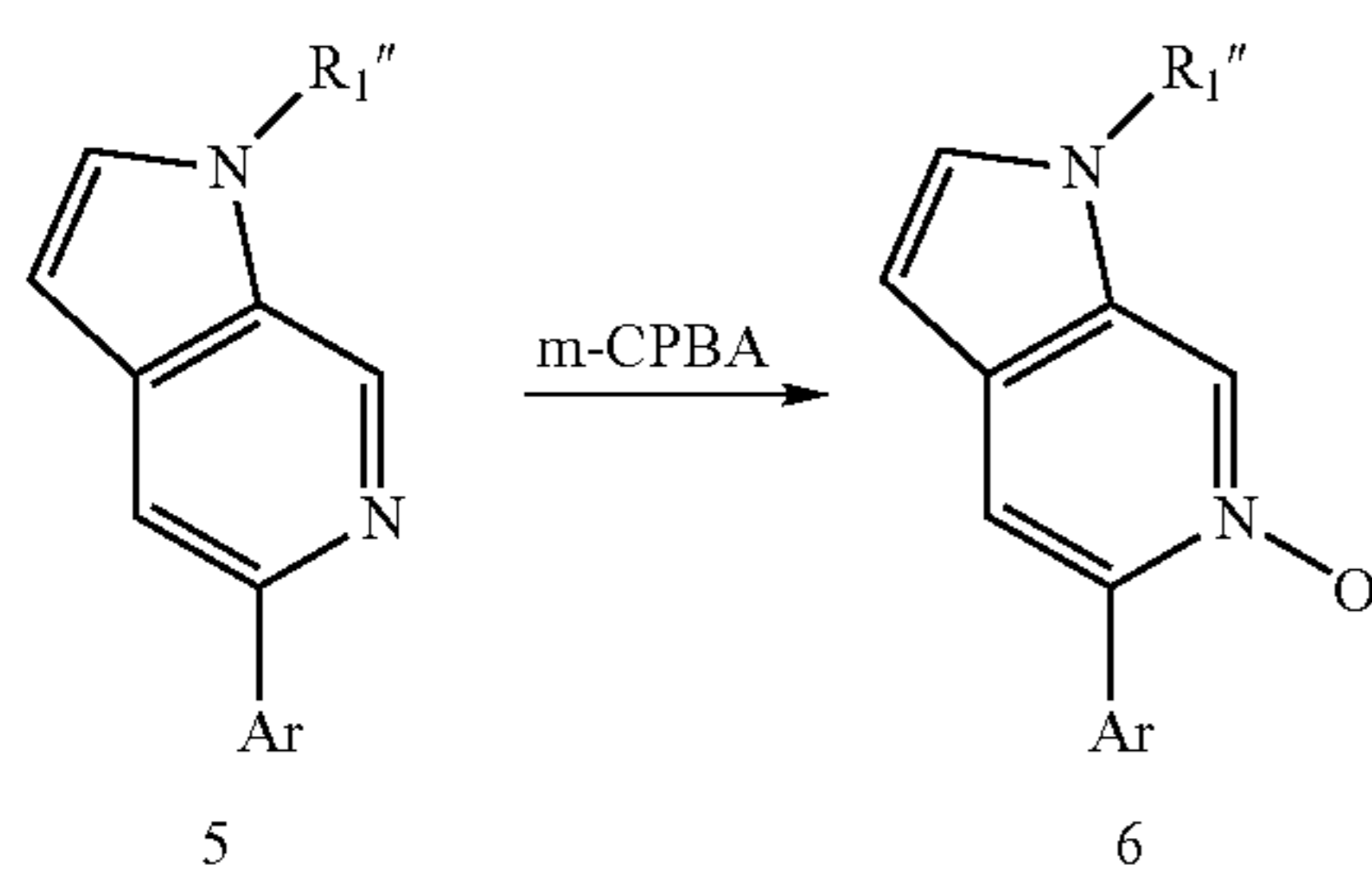
Scheme 3. Preparation of Compounds of Formula Ia wherein R 5 is attached to Compound 5.
