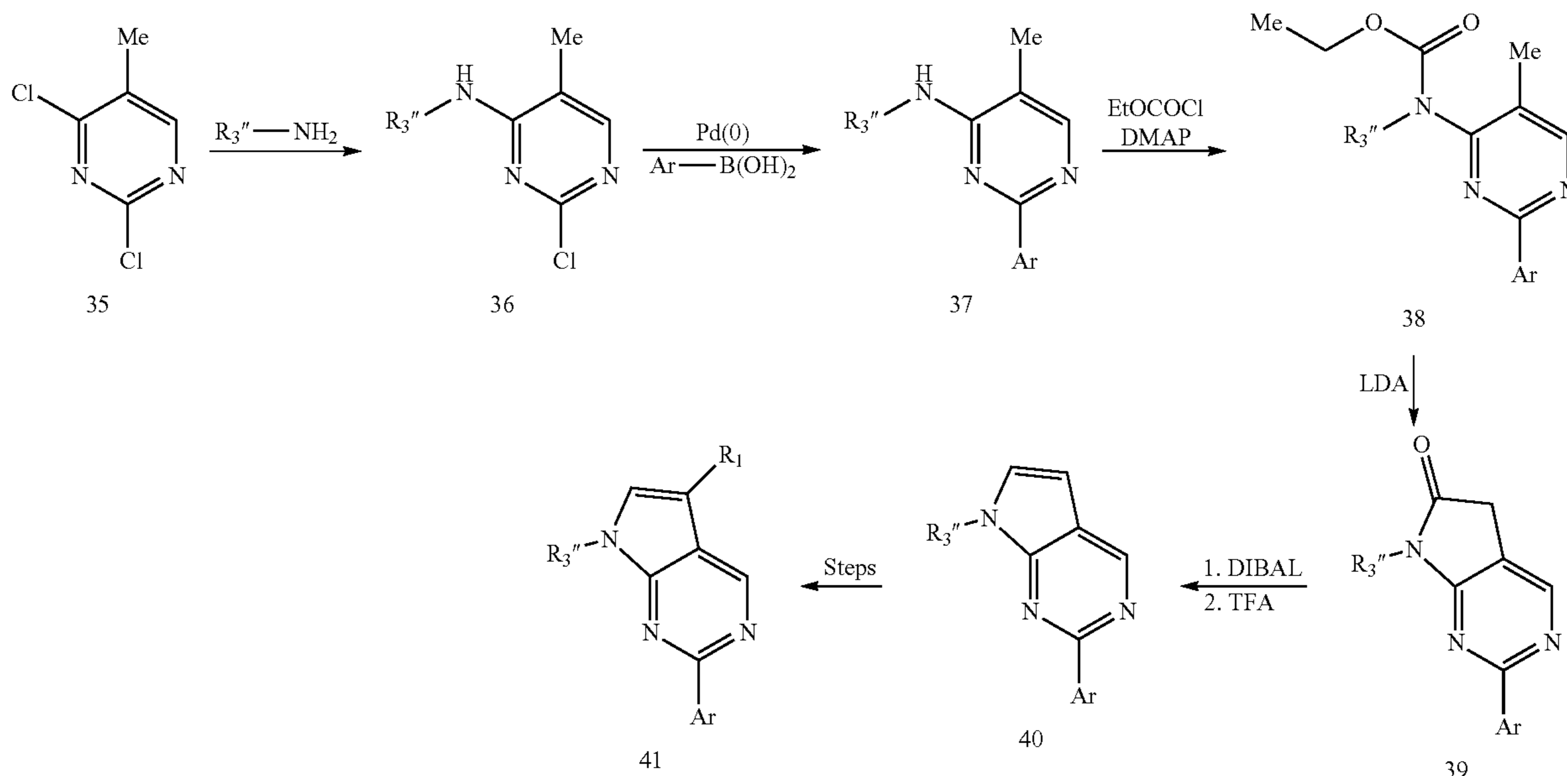
Scheme 10 Preparation of compounds of Formula I or Formula II in which Z 1 is CR 1 and Z 3 is NR 3 '' and Z 4 is N.
