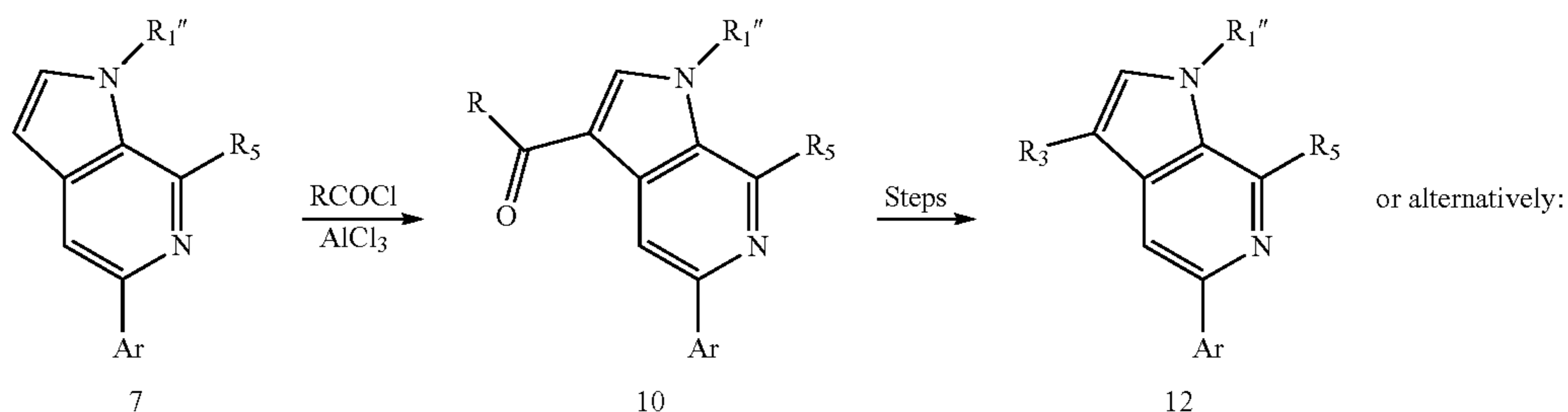
Scheme 5. Preparation of compounds of Formula I or Formula II.
