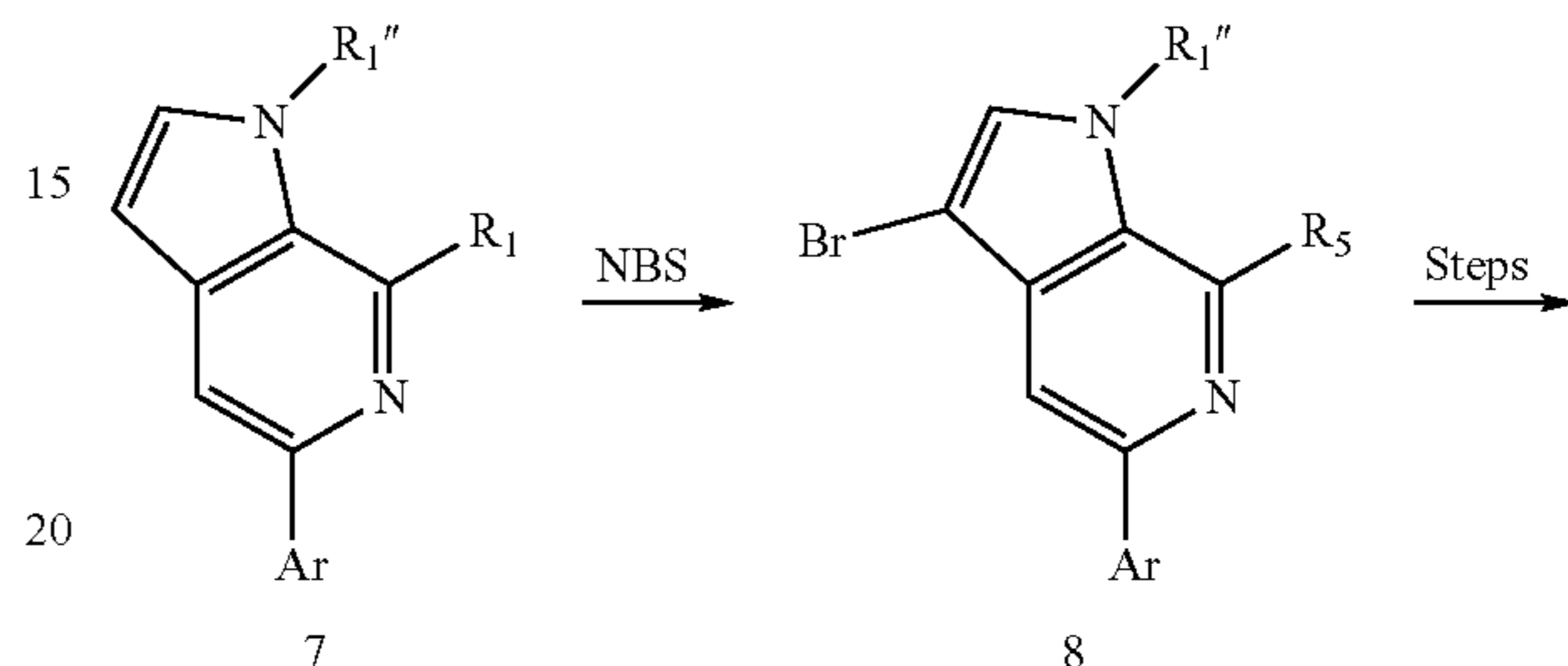
Scheme 4. Preparation of compounds of Formula I or Formula II where R 3 is introduced.
