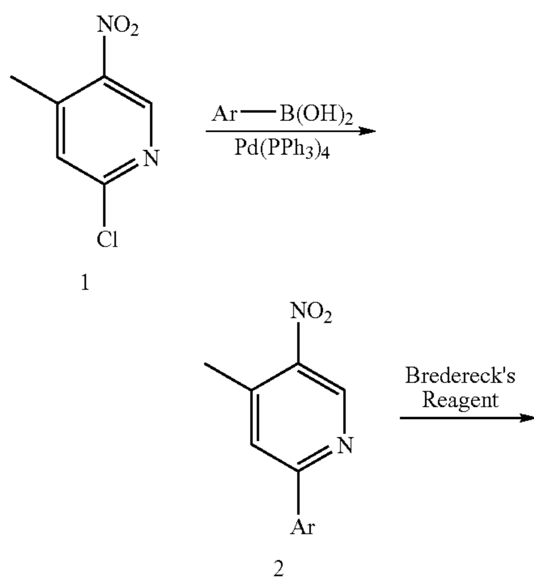
Scheme 1. Preparation of Intermediate for synthesis of compounds of Formula Ia.
