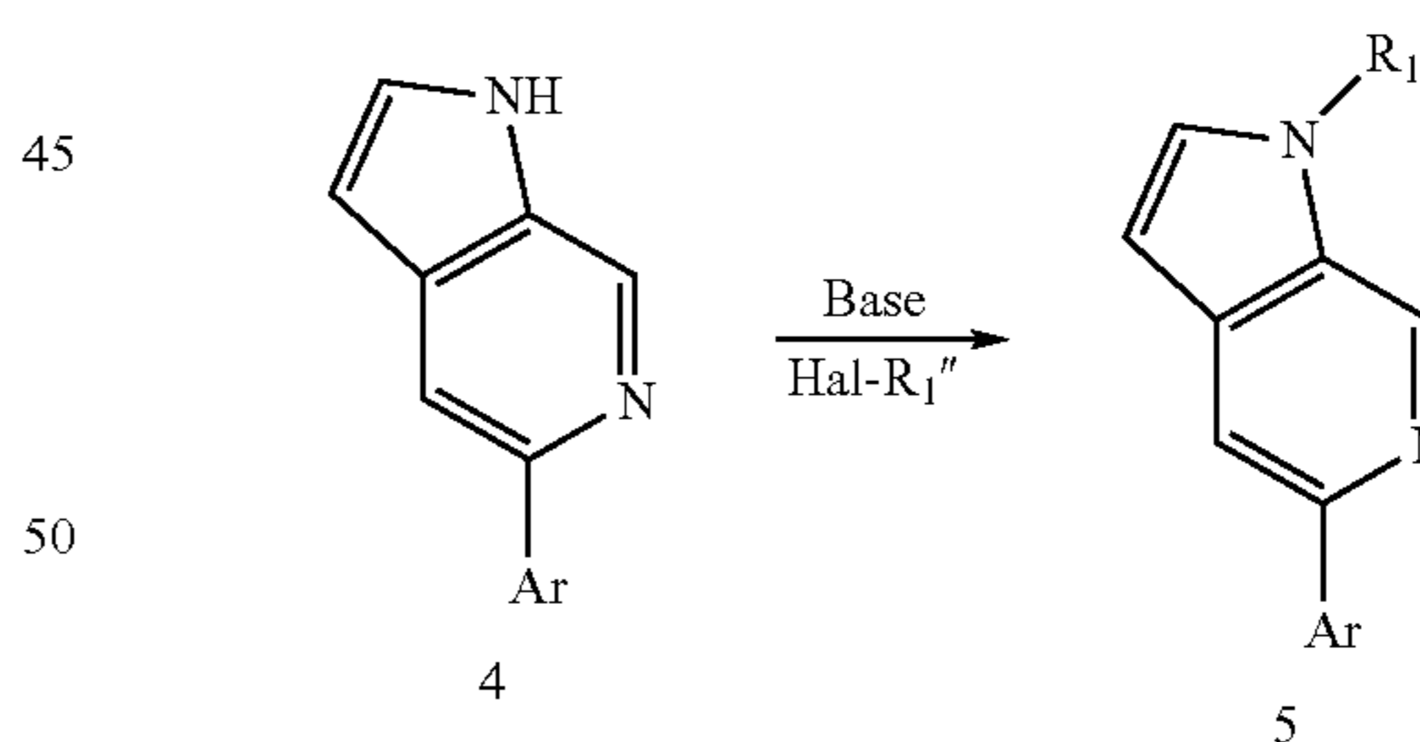
Scheme 2. Preparation of compounds of Formula Ia wherein R 1 " is attached to intermediate 4.
