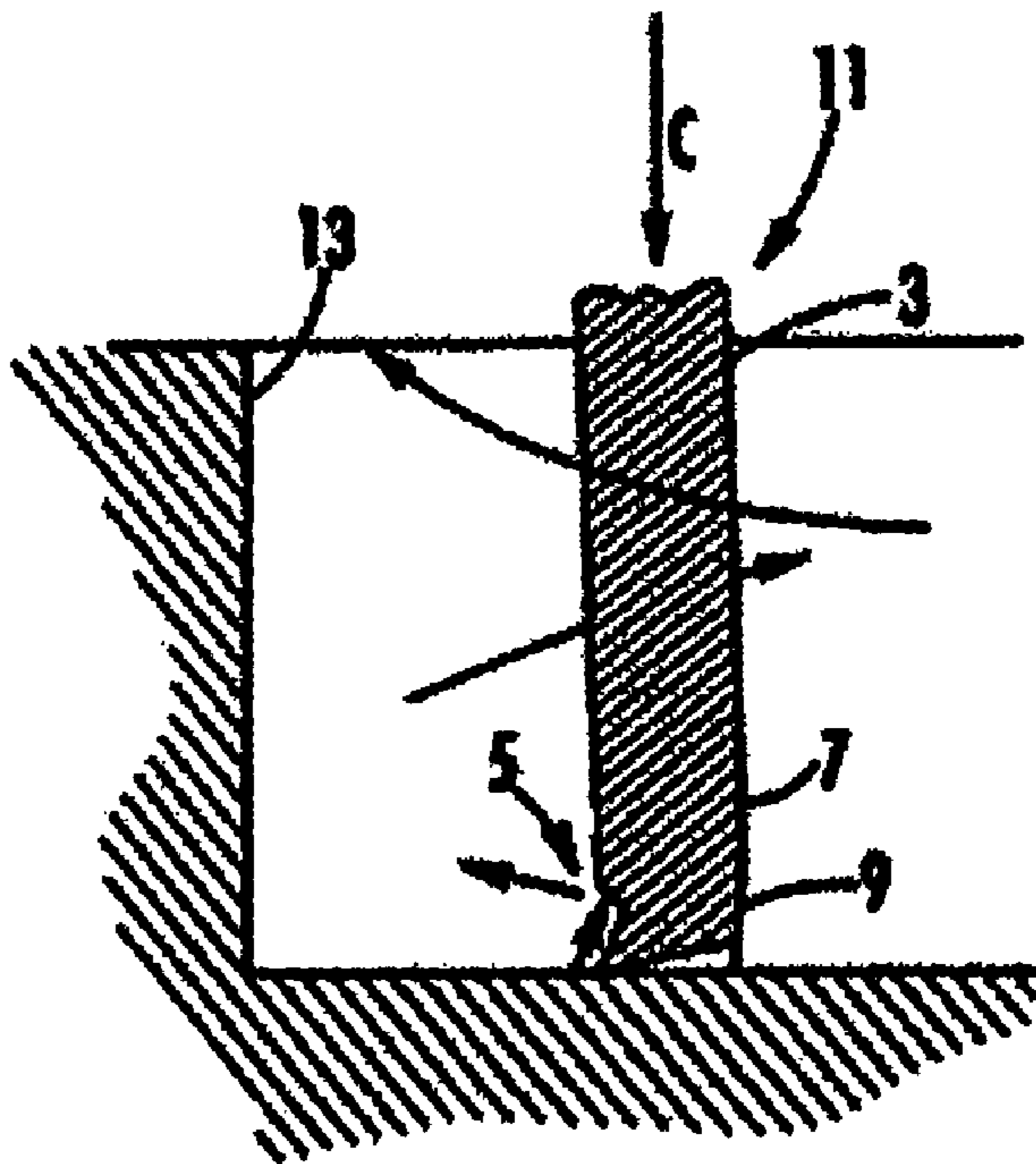
FIG. 8 (PRIOR ART)
