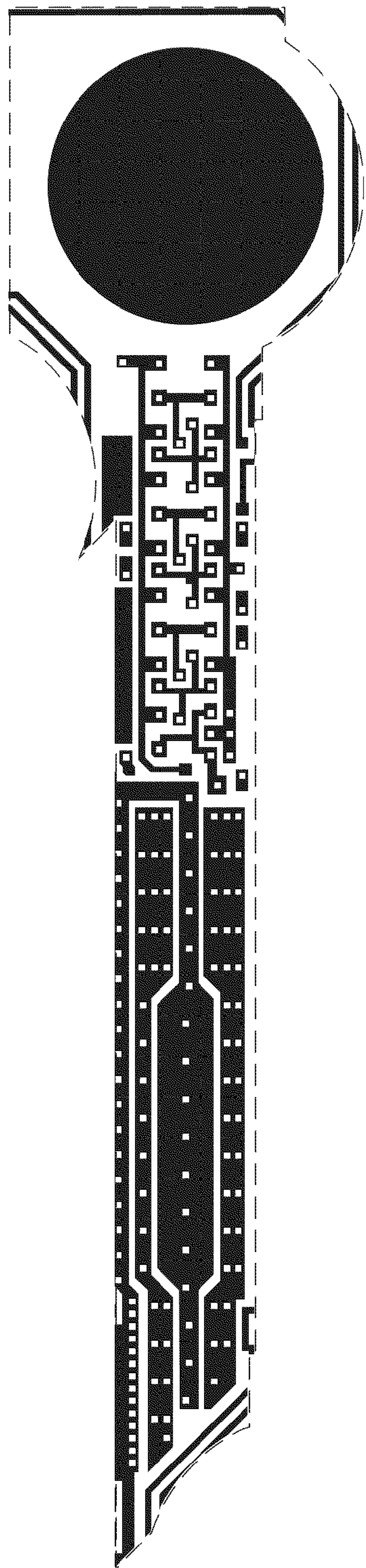
Metal 1 mask
