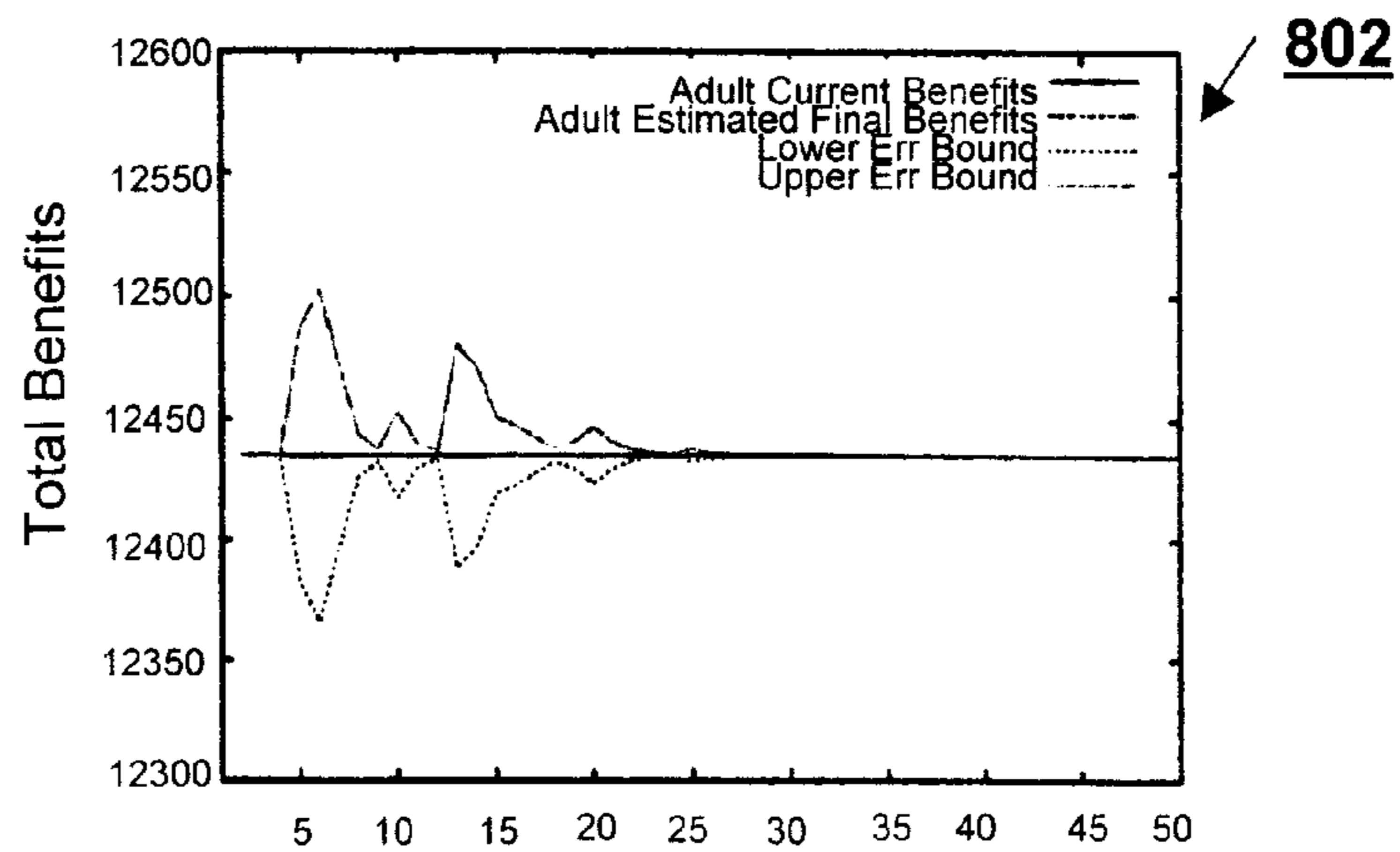
FIG.8C Sampling Size (Number of Classifiers)
