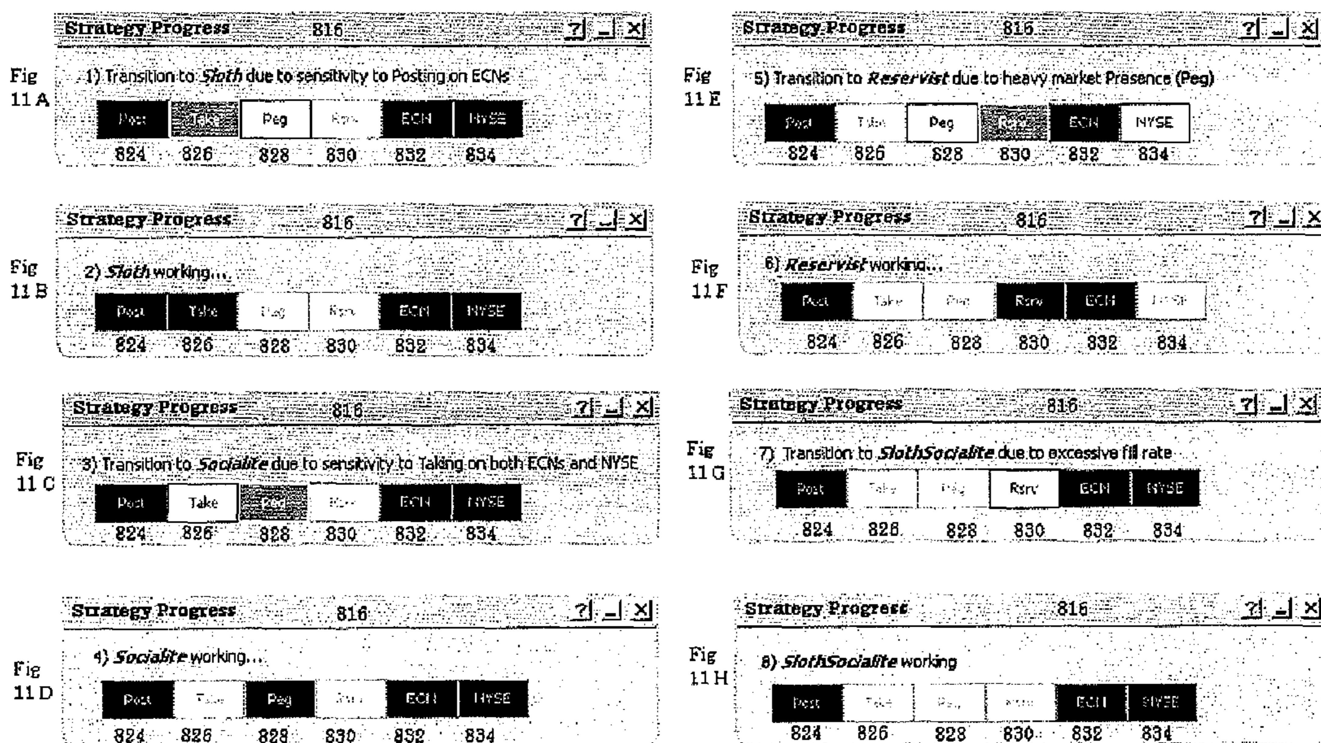
Figure 11: Examples of tactic update messages in Strategy Progress area
