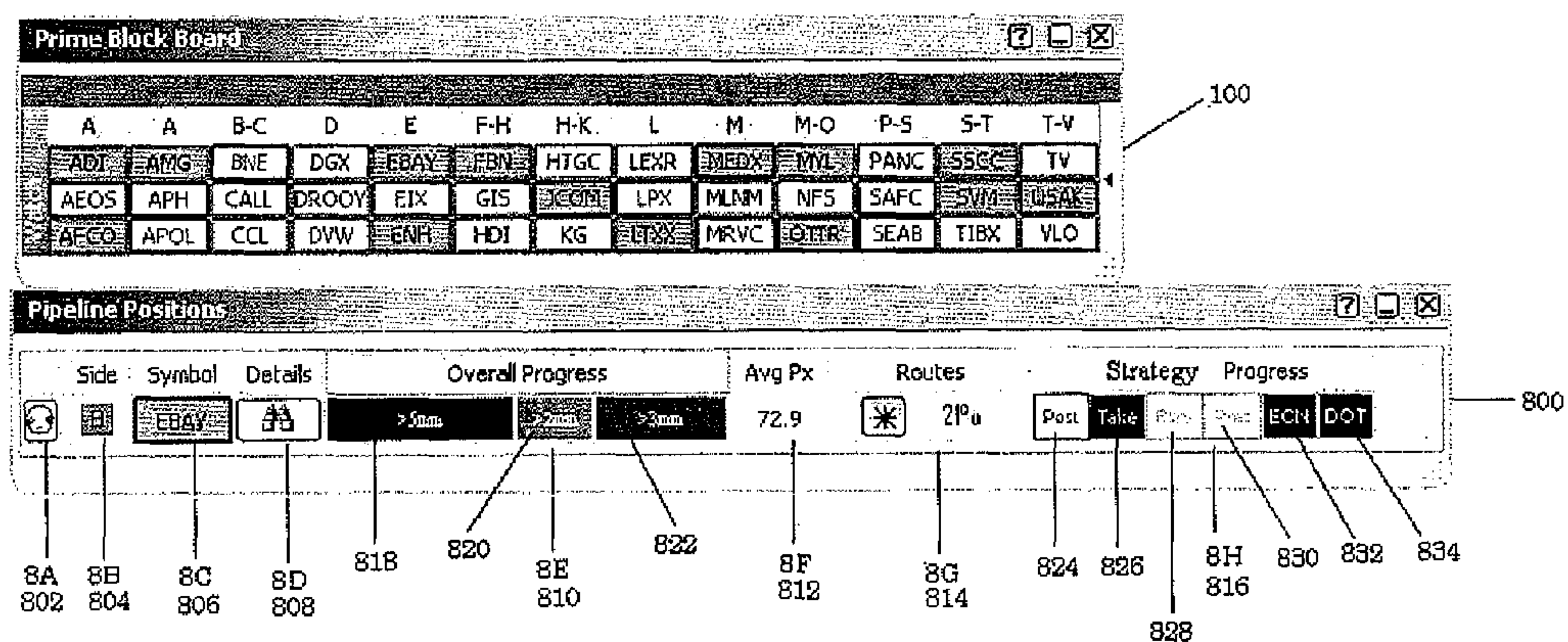
Figure 8: Positions Window
