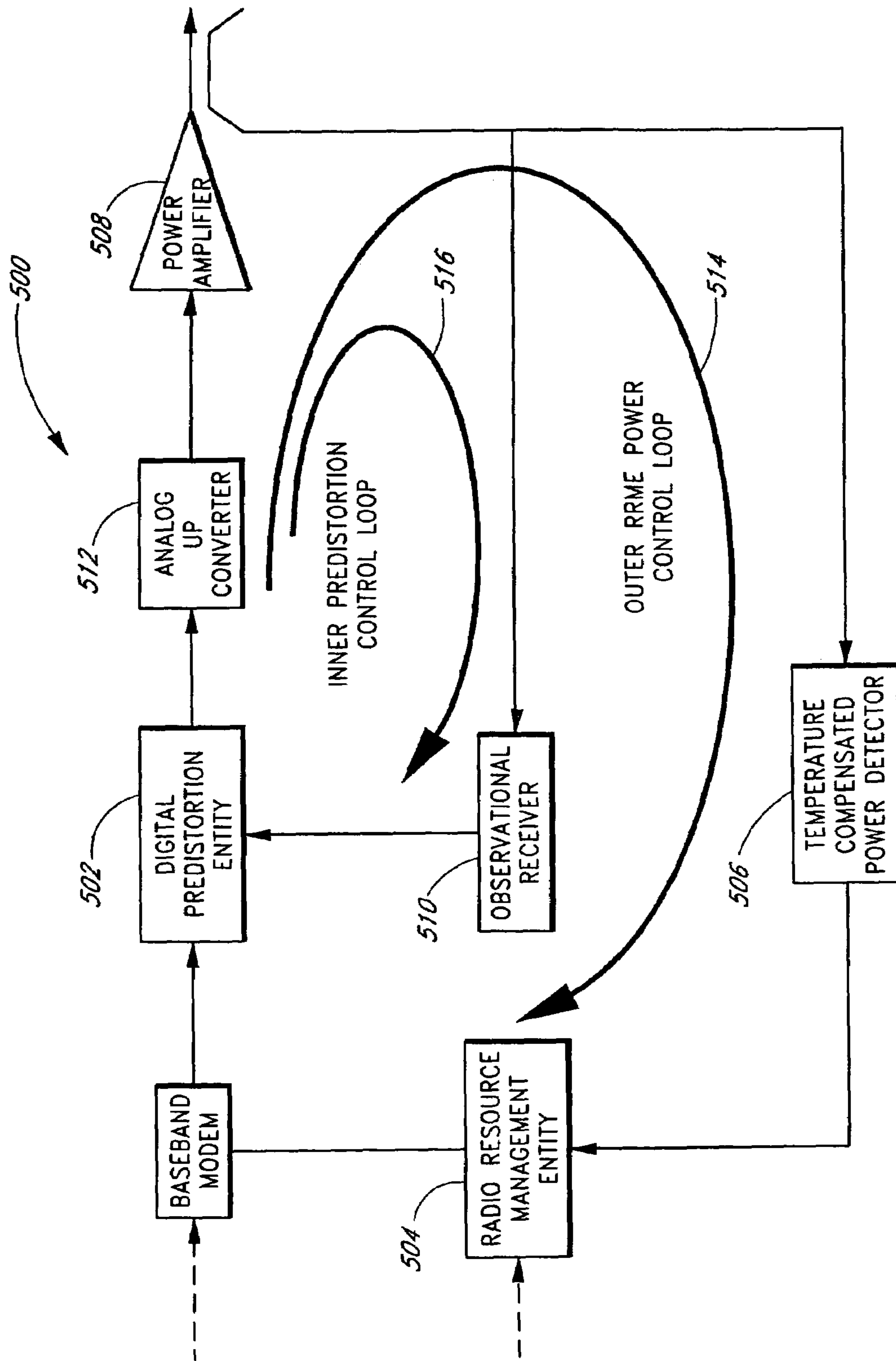
FIG. 5 (PRIOR ART)
