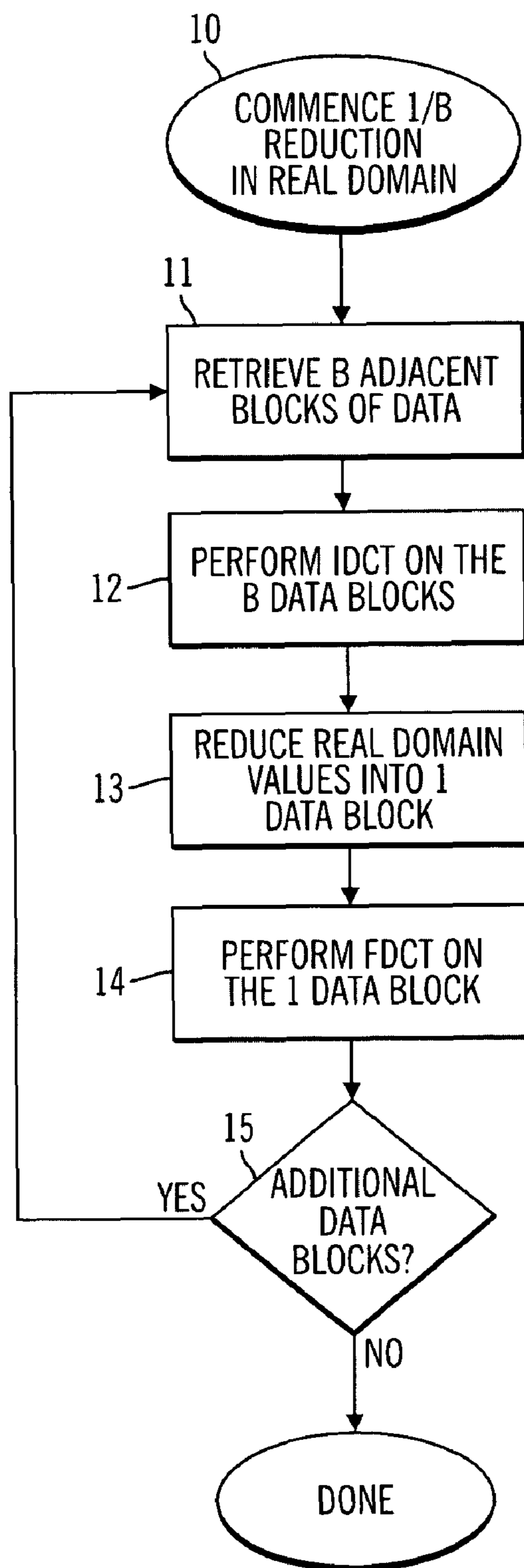
FIG. 1 (PRIOR ART)
