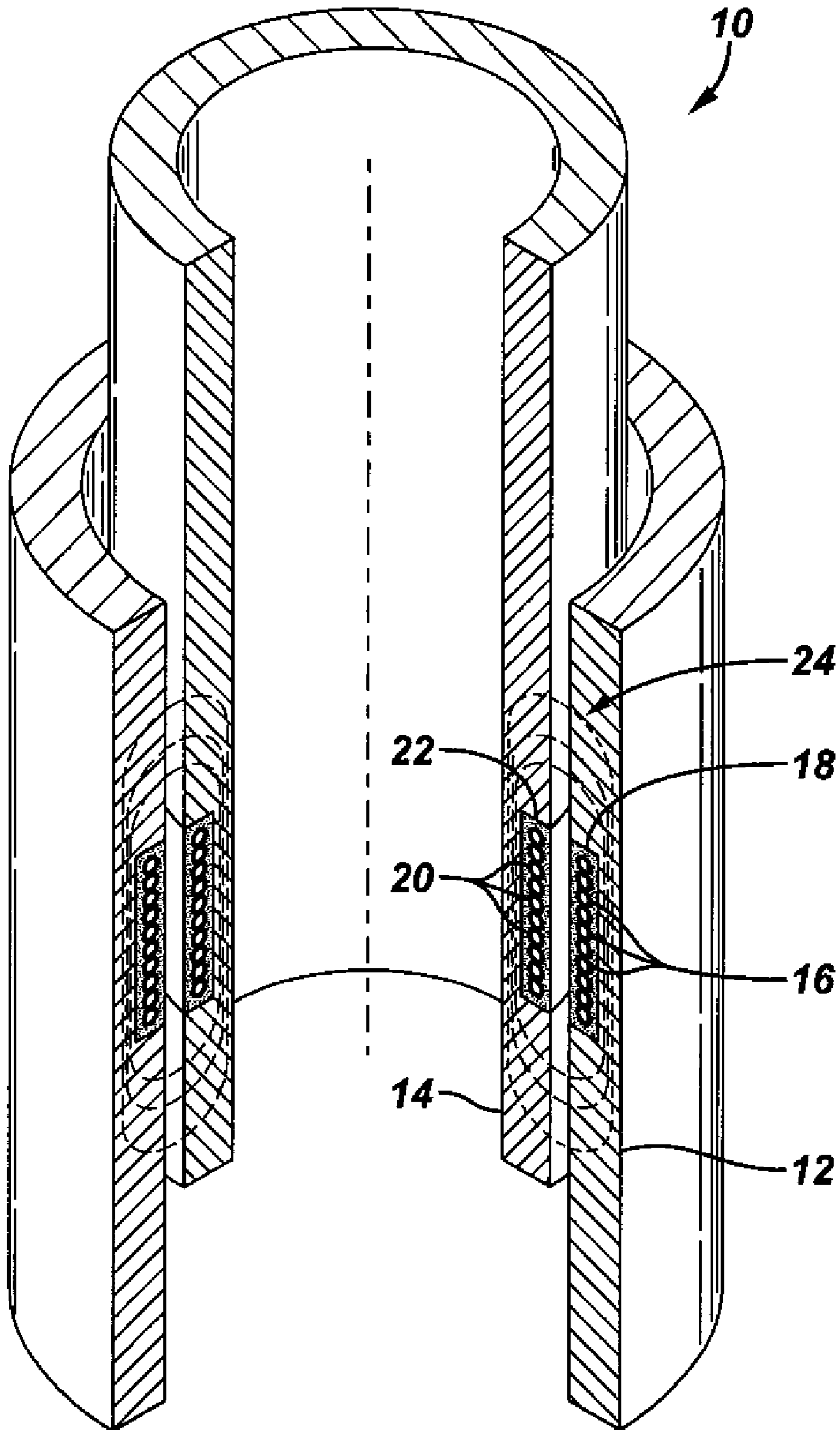
FIG. 1 (Prior Art)
