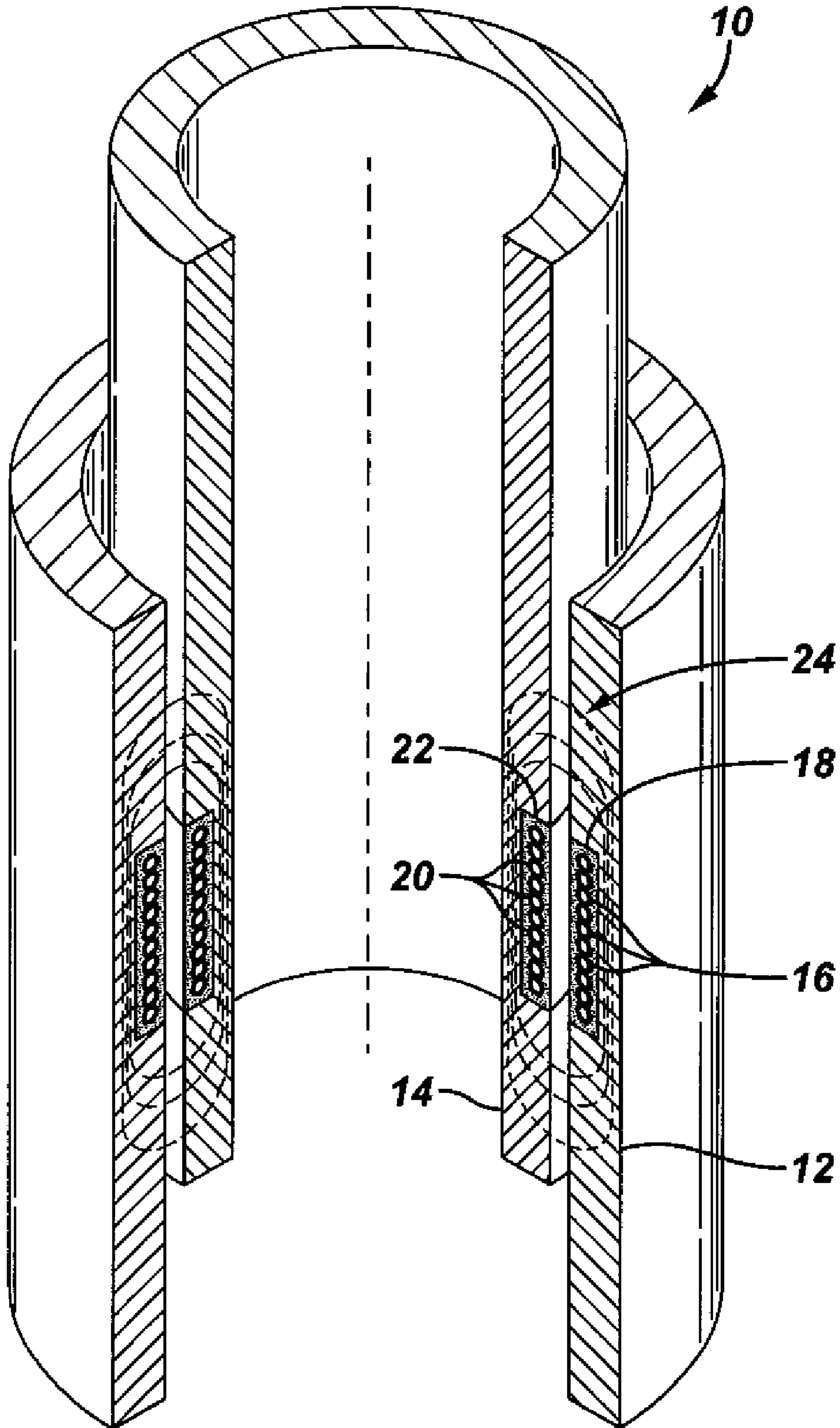
FIG. 1 (Prior Art)
