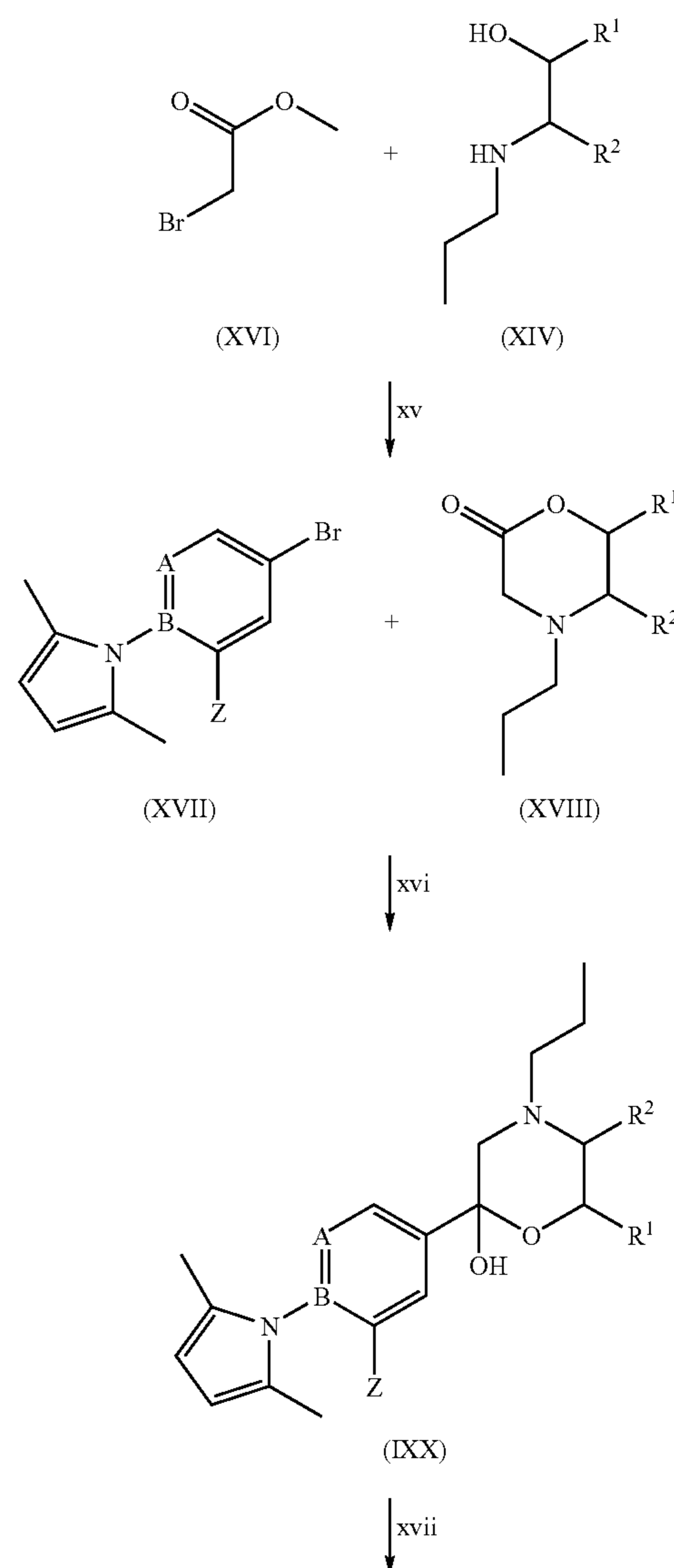
Scheme 4
