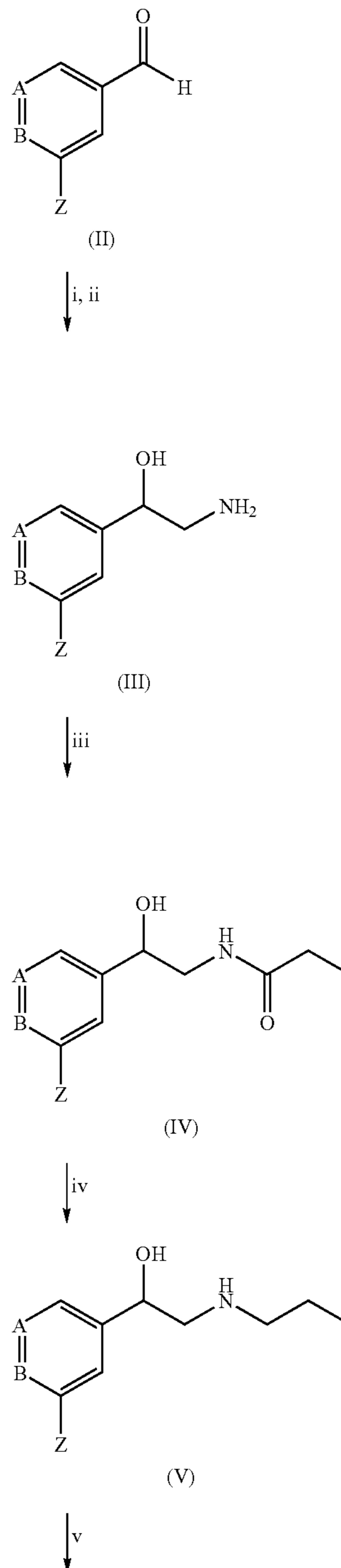
Scheme 1
