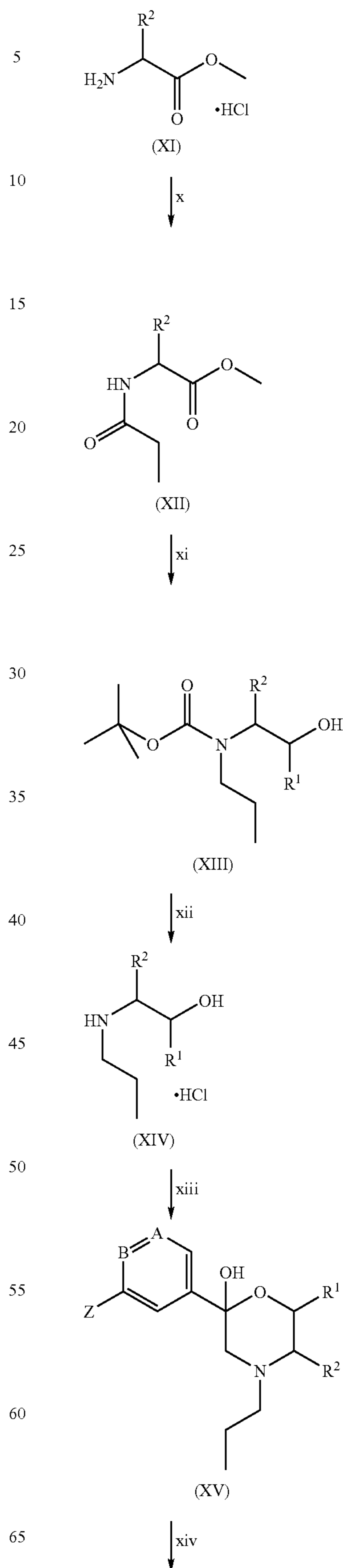
Scheme 3
