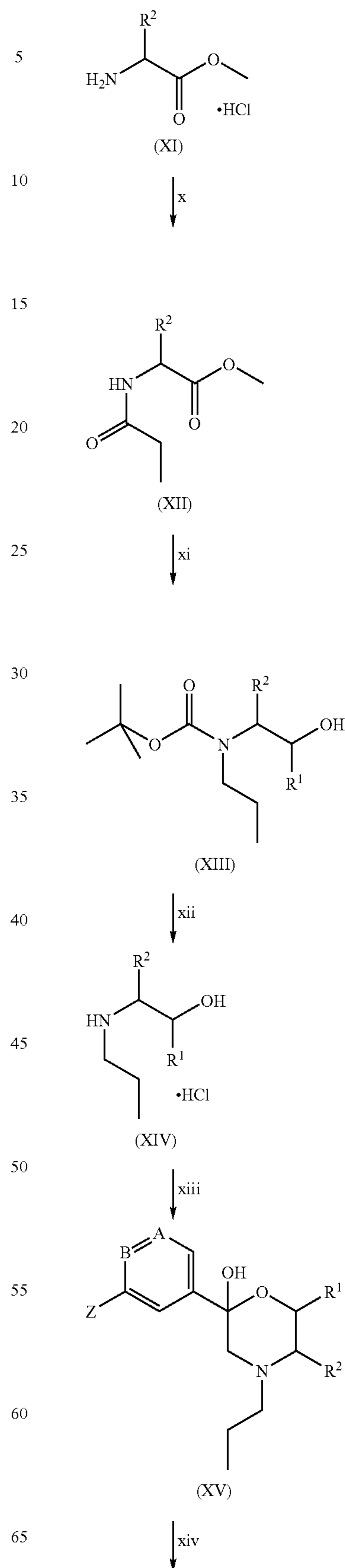
Scheme 3
