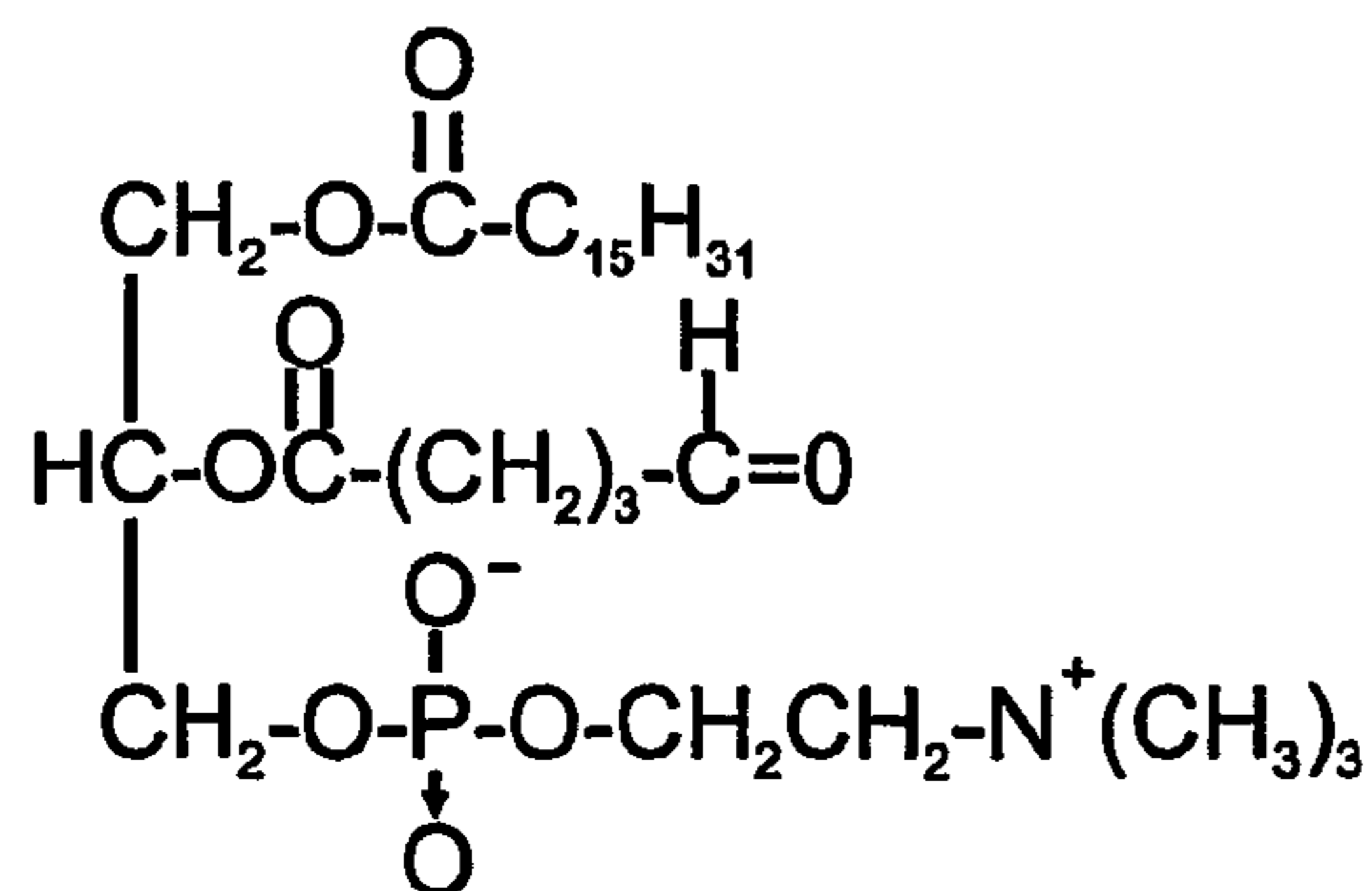
POVPC 1-Hexadecanoyl-2-(5'-oxopentanoyl)-sn-3-glycerophosphocholine
