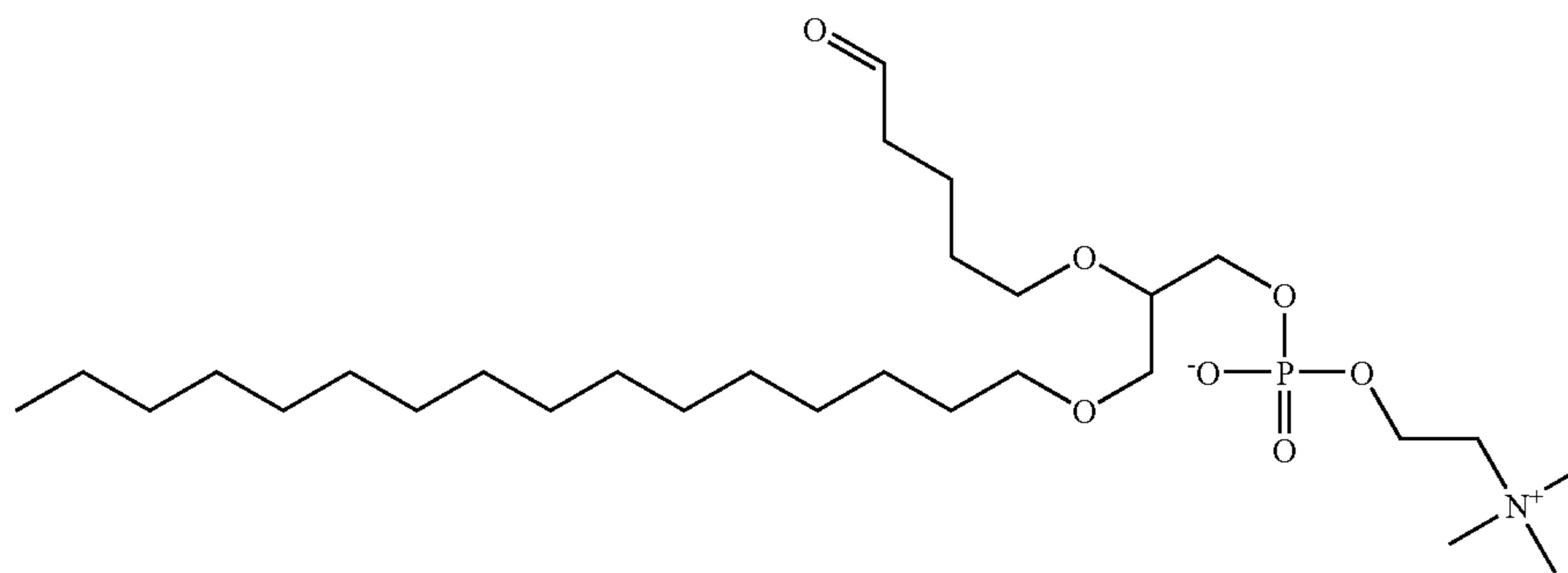
1-hexadecyl-2-(5'-oxo-pentanyl)-sn-glycero-3-phosphocholine
