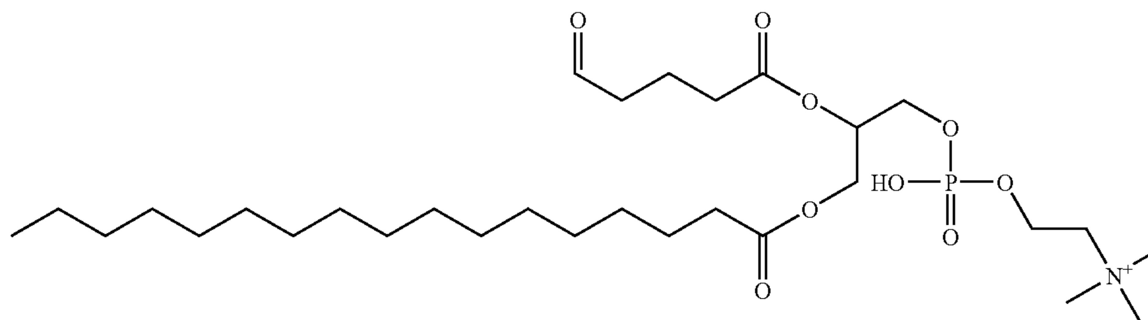
1-hexadecanoyl-2-(5'-oxo-valeroyl)-sn-3-phosphocholine
