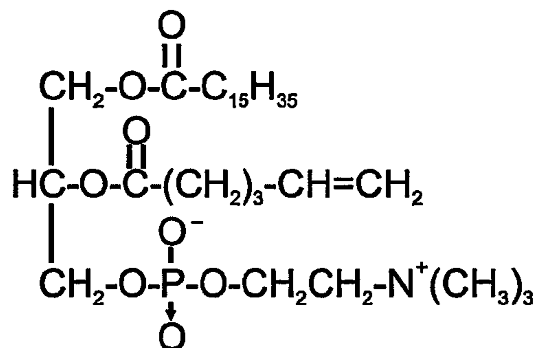
1-Hexadecanoyl-2-(5'-hexenoyl)sn-3-glycerophosphocholine
