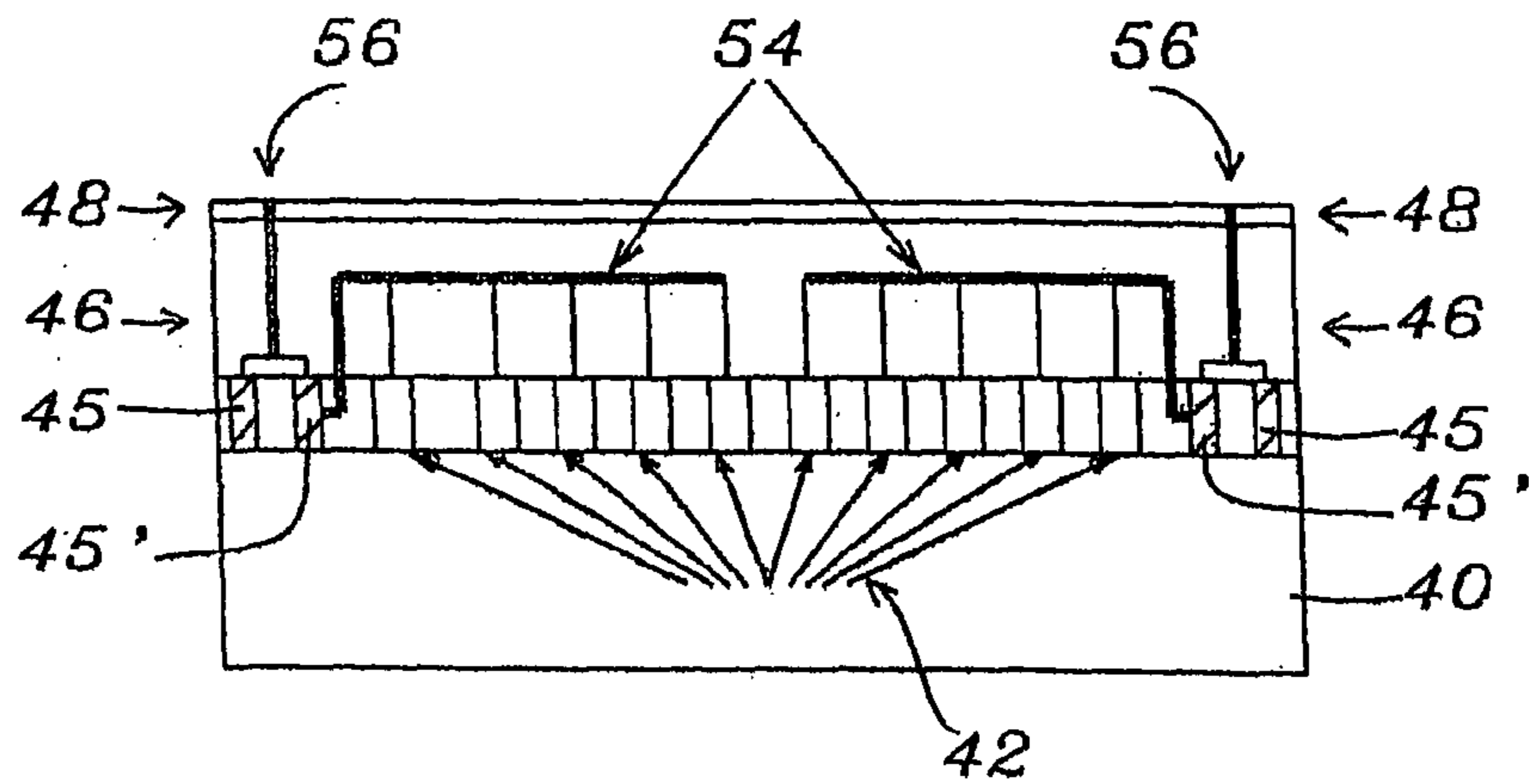
FIG. 2 - Prior Art
