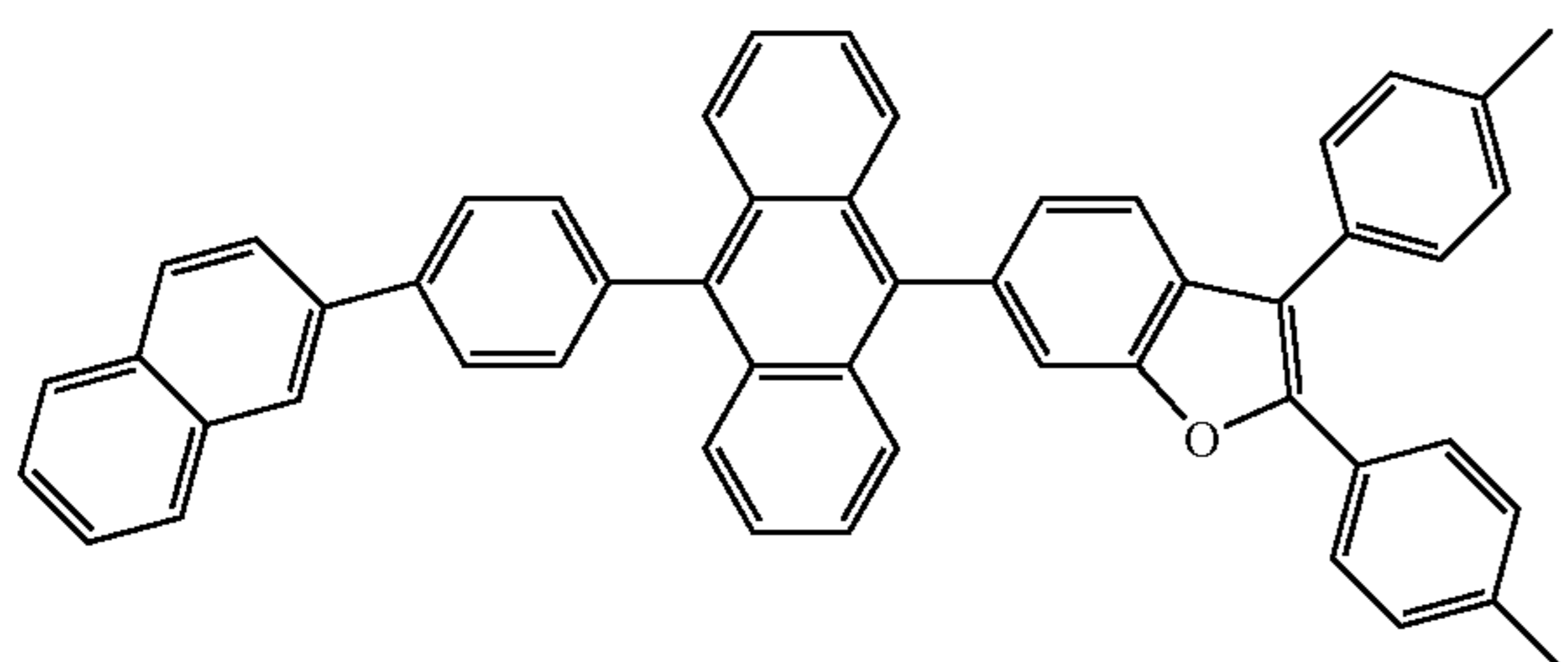
<Formula 31>
