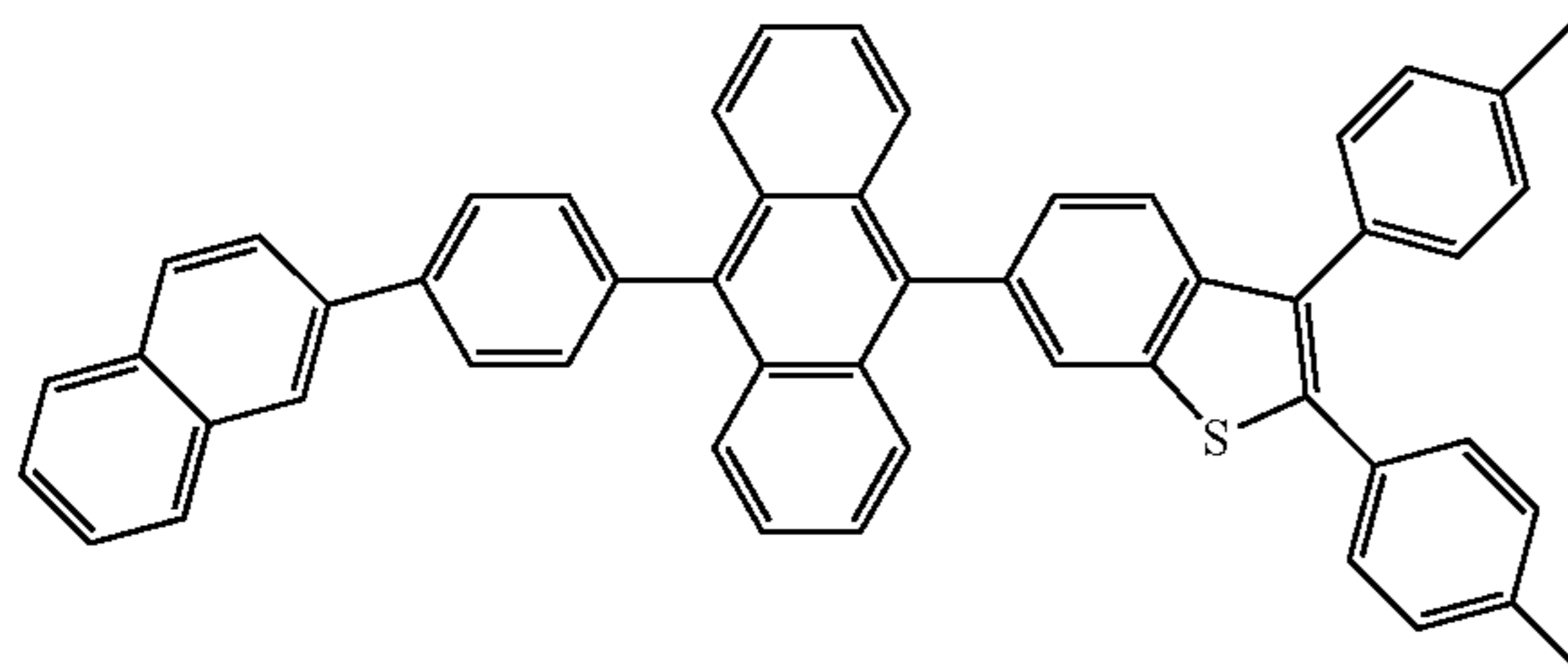
&lt;Formula 6&gt;
