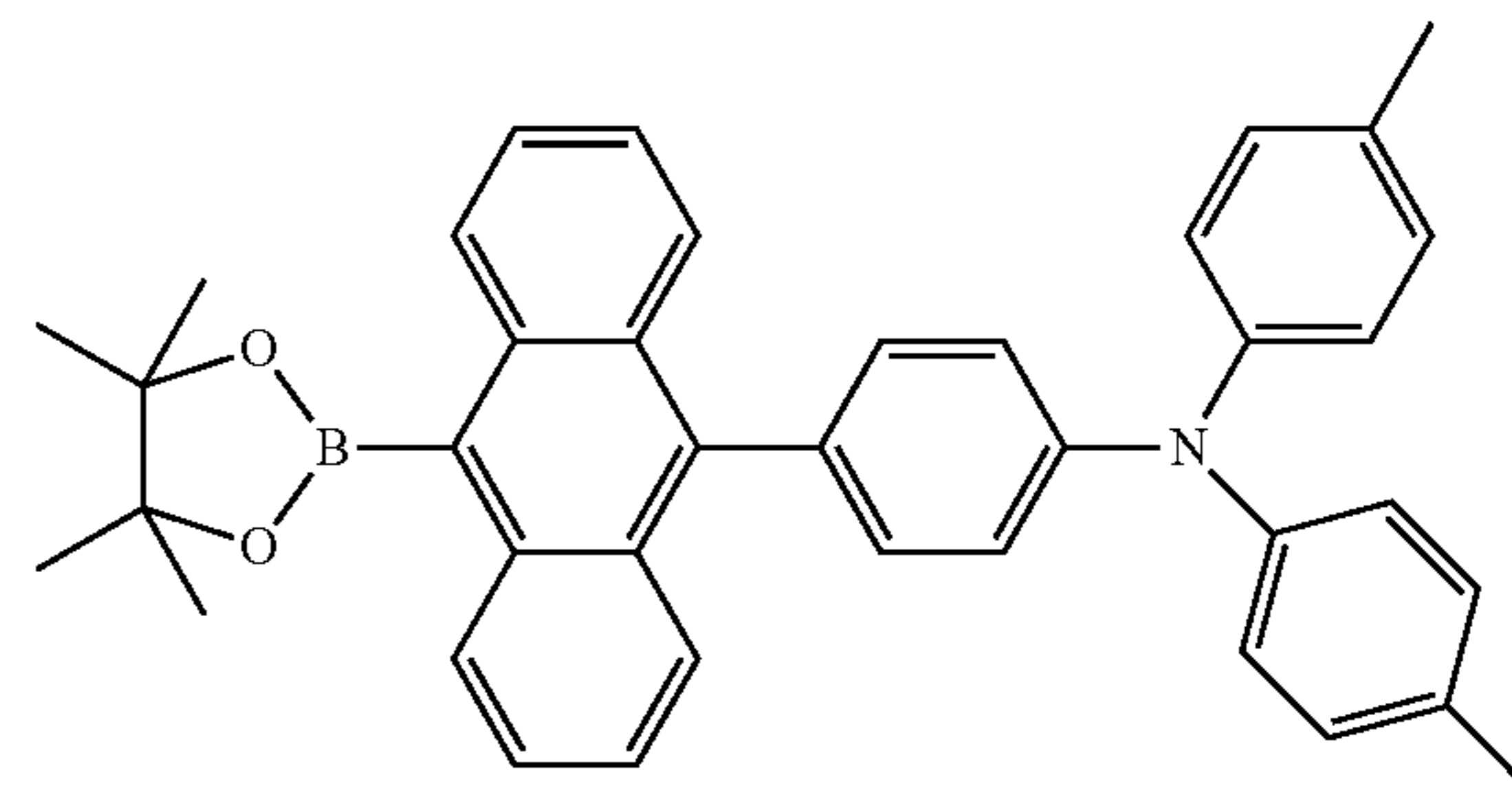
INTERMEDIATE D
