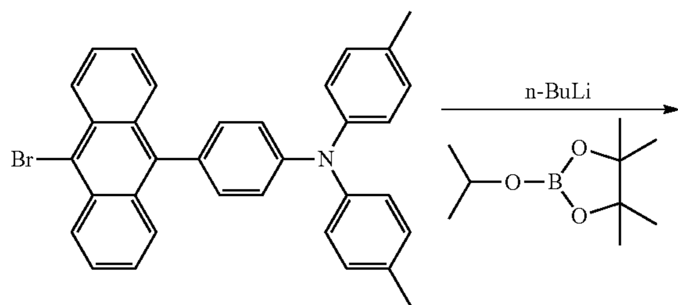
[Reaction Scheme 7]
