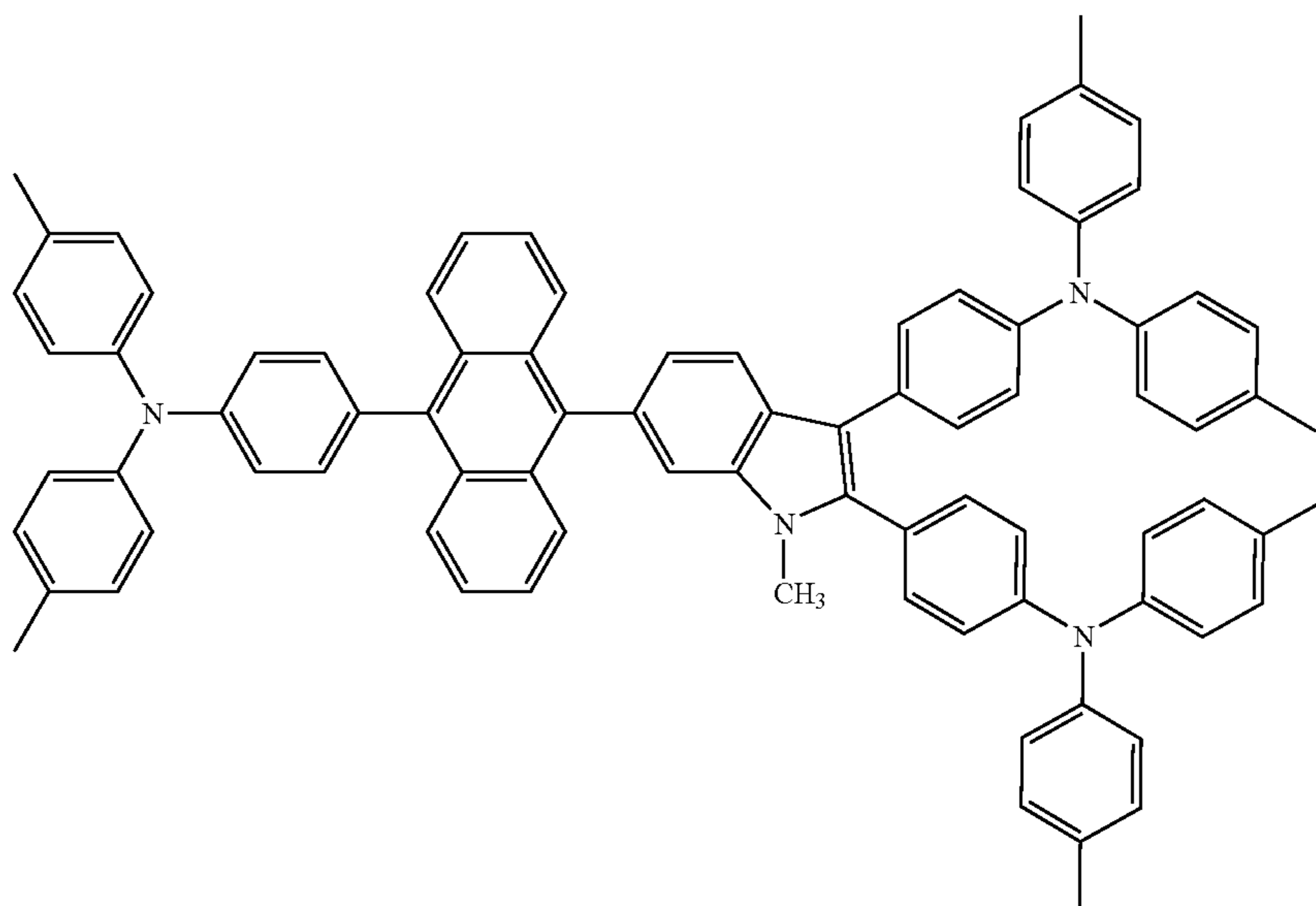
<Formula 70>
