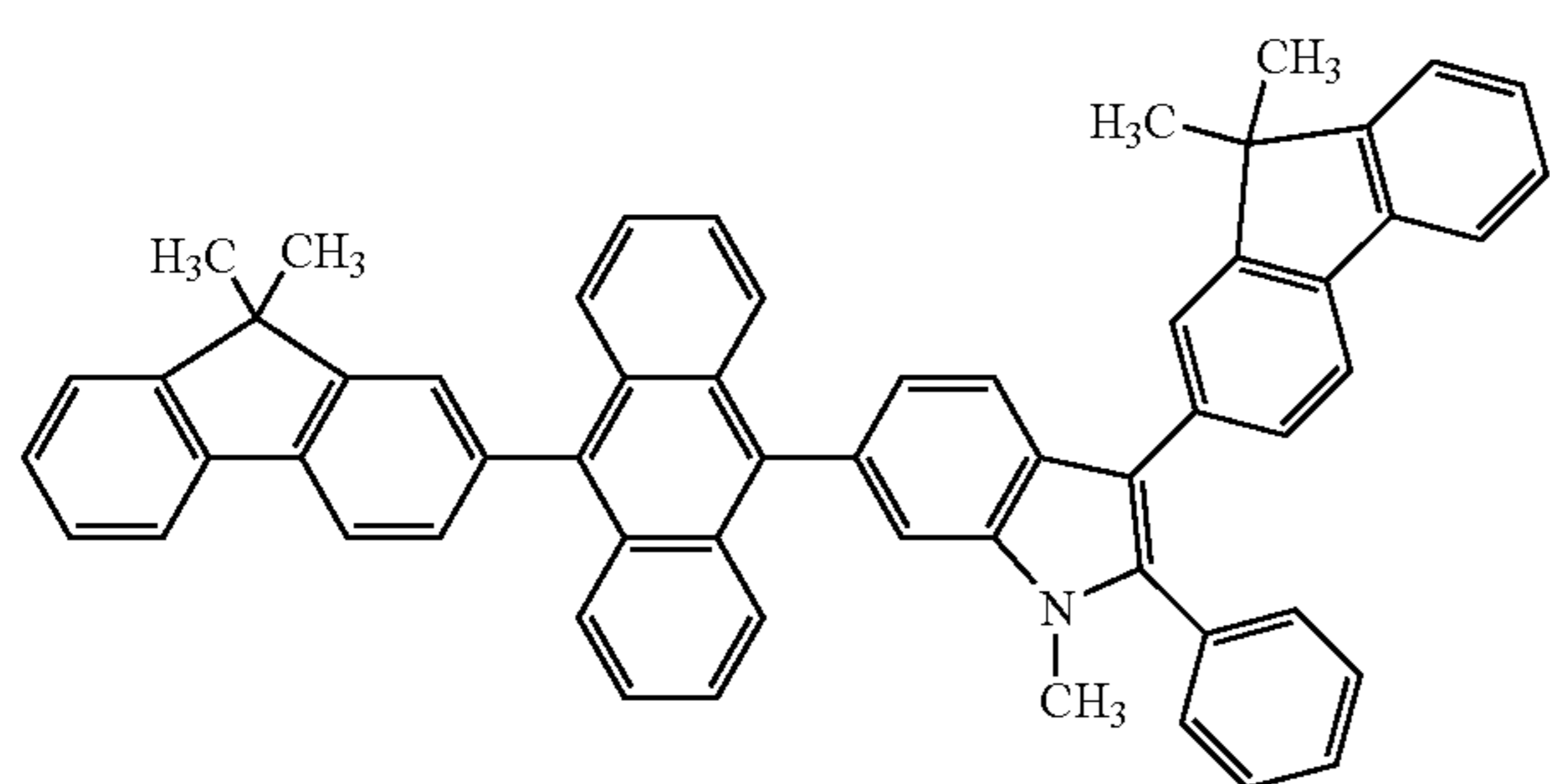
<Formula 67>
