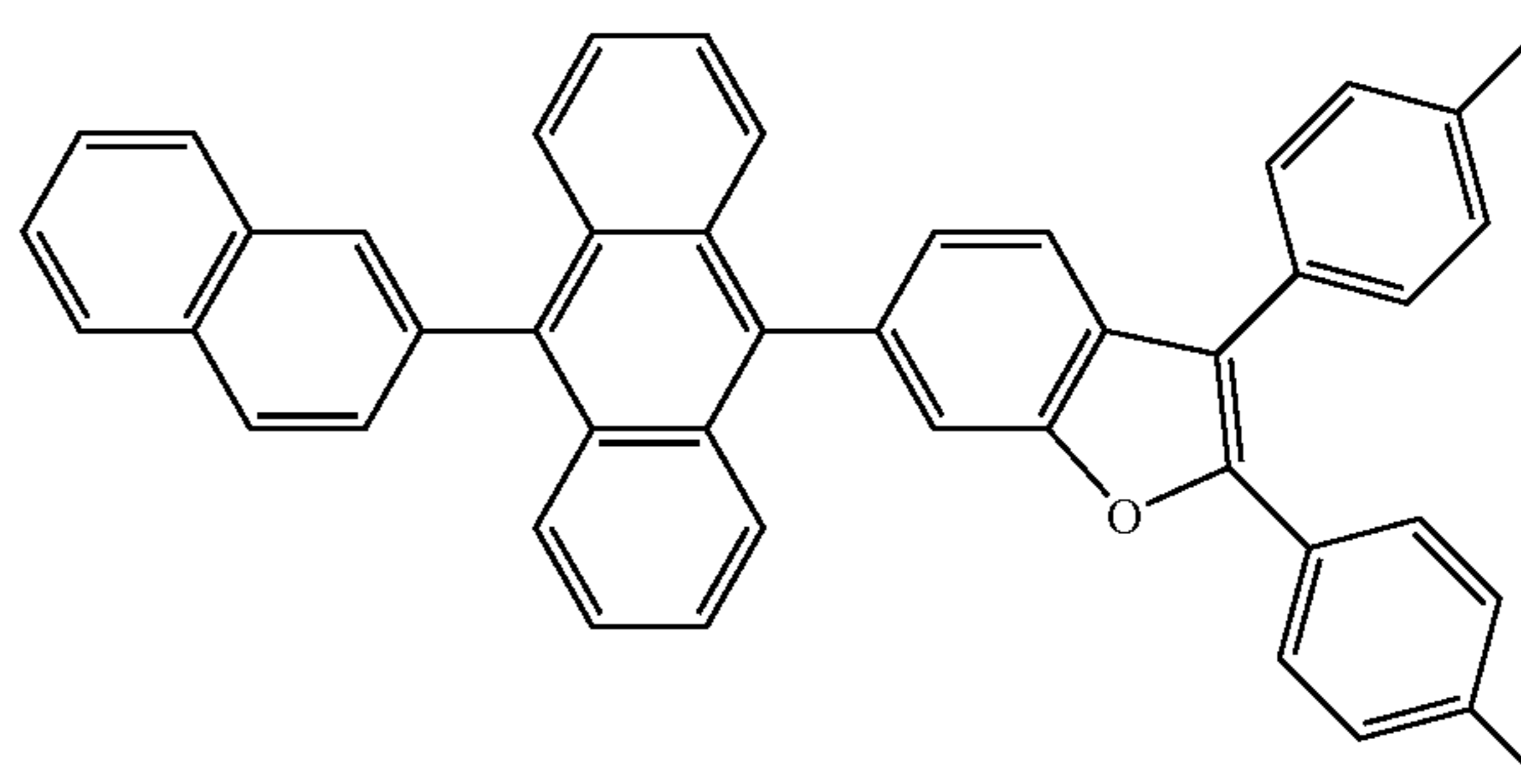
<Formula 30>
