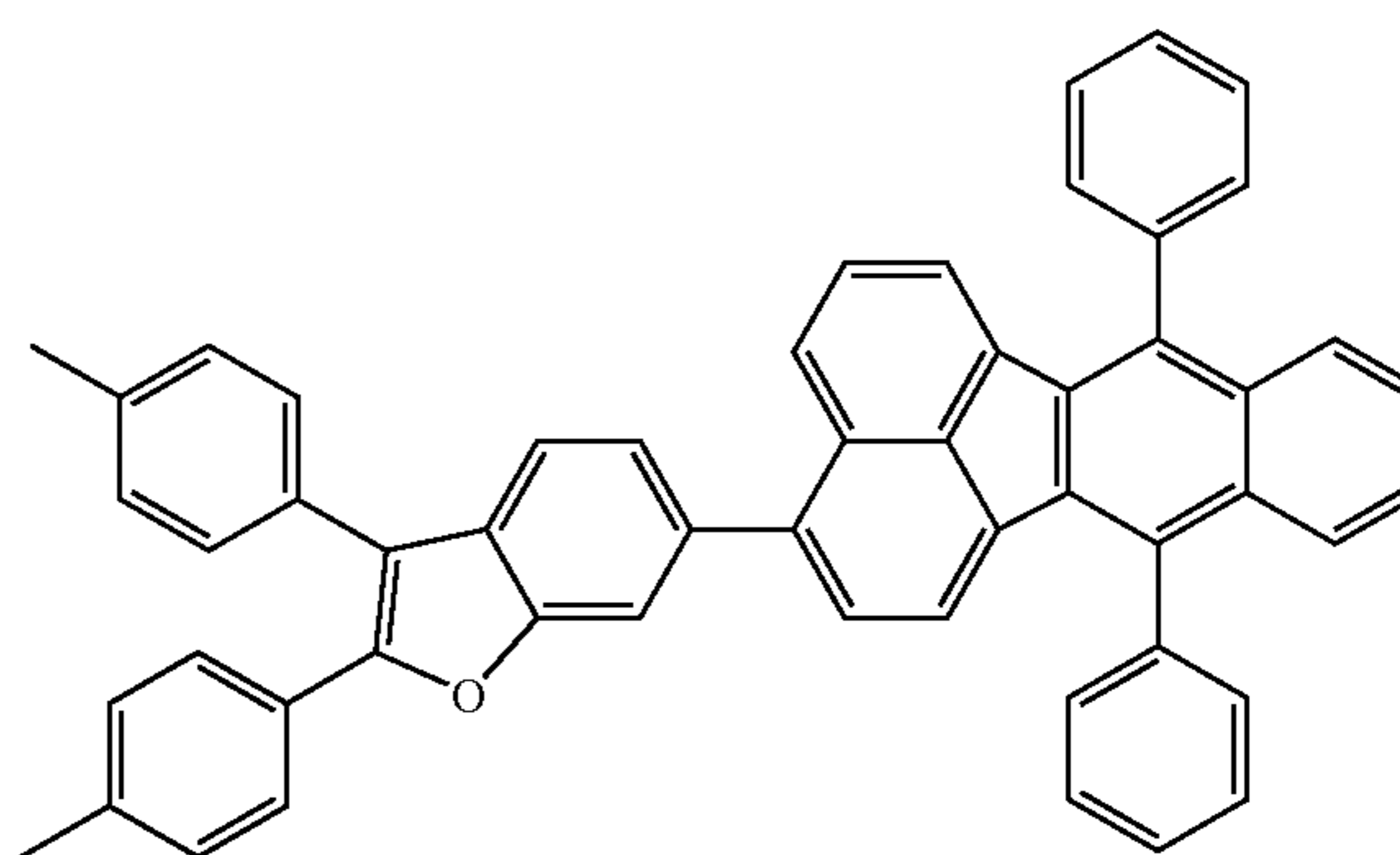
<Formula 48>
