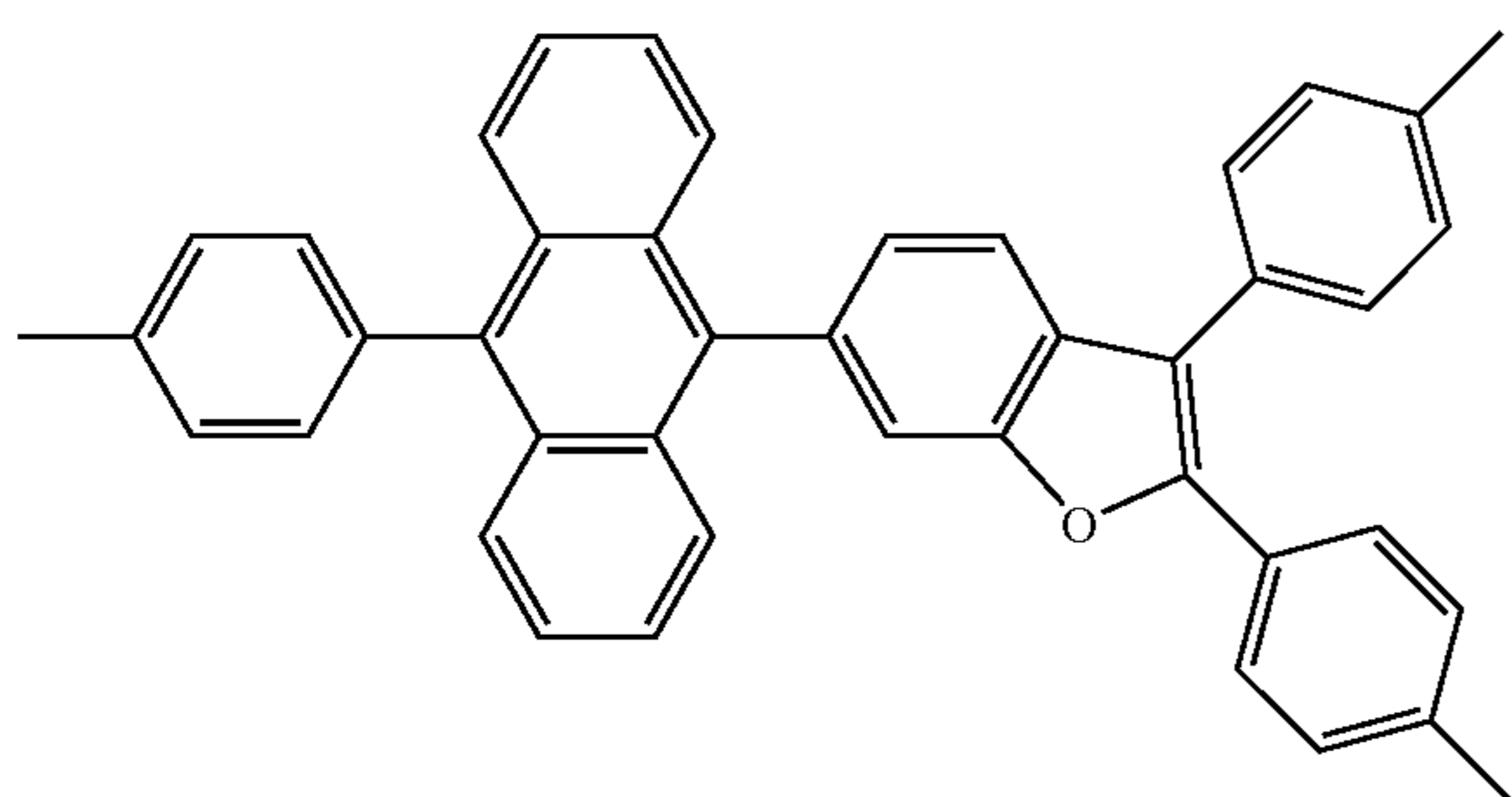
<Formula 29>
