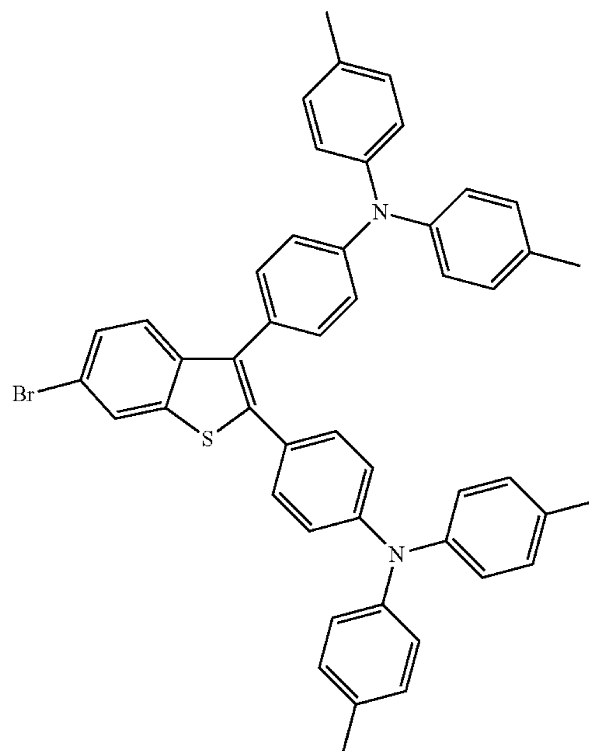
INTERMEDIATE C
