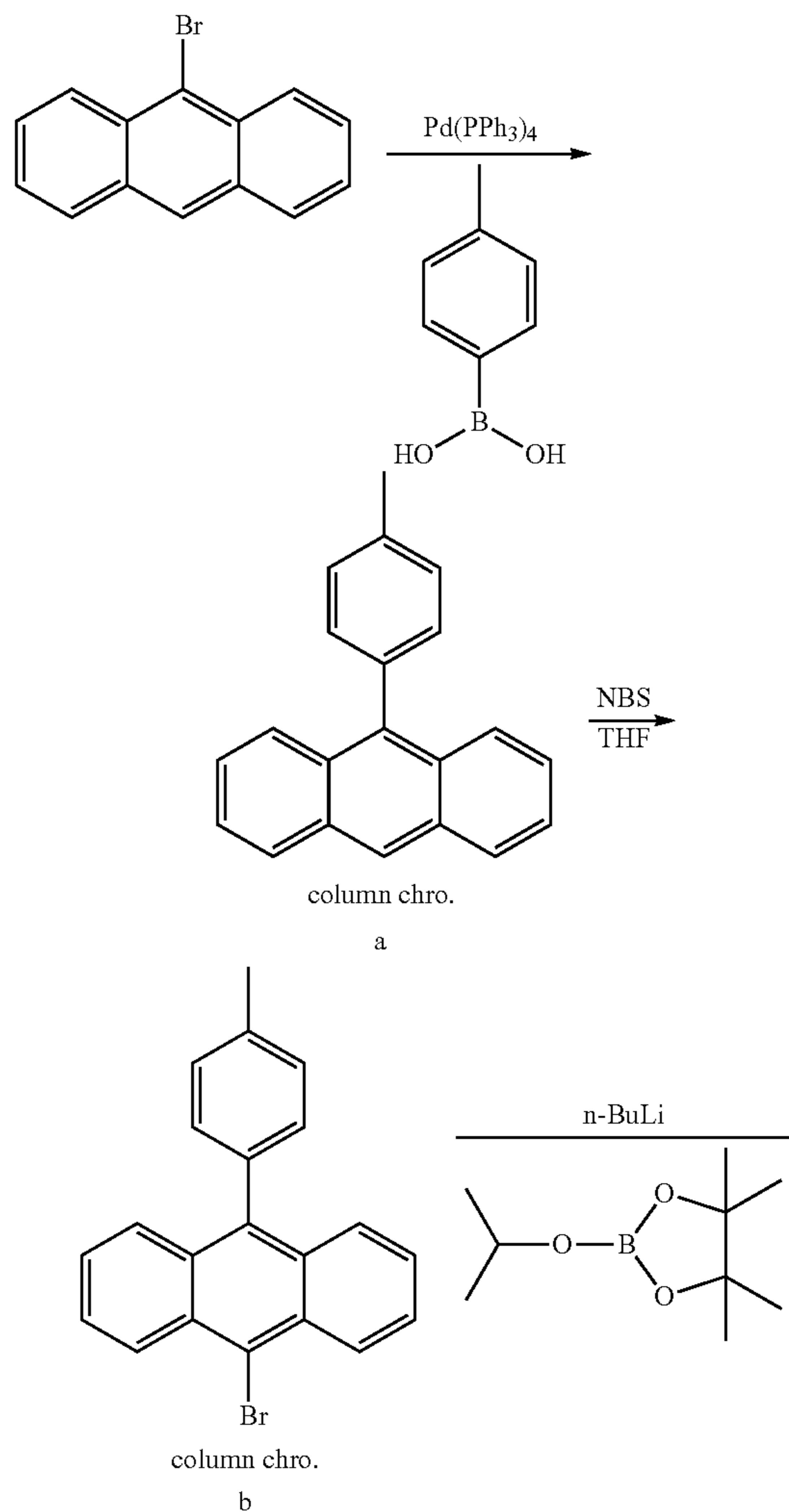
[Reaction Scheme 1]
