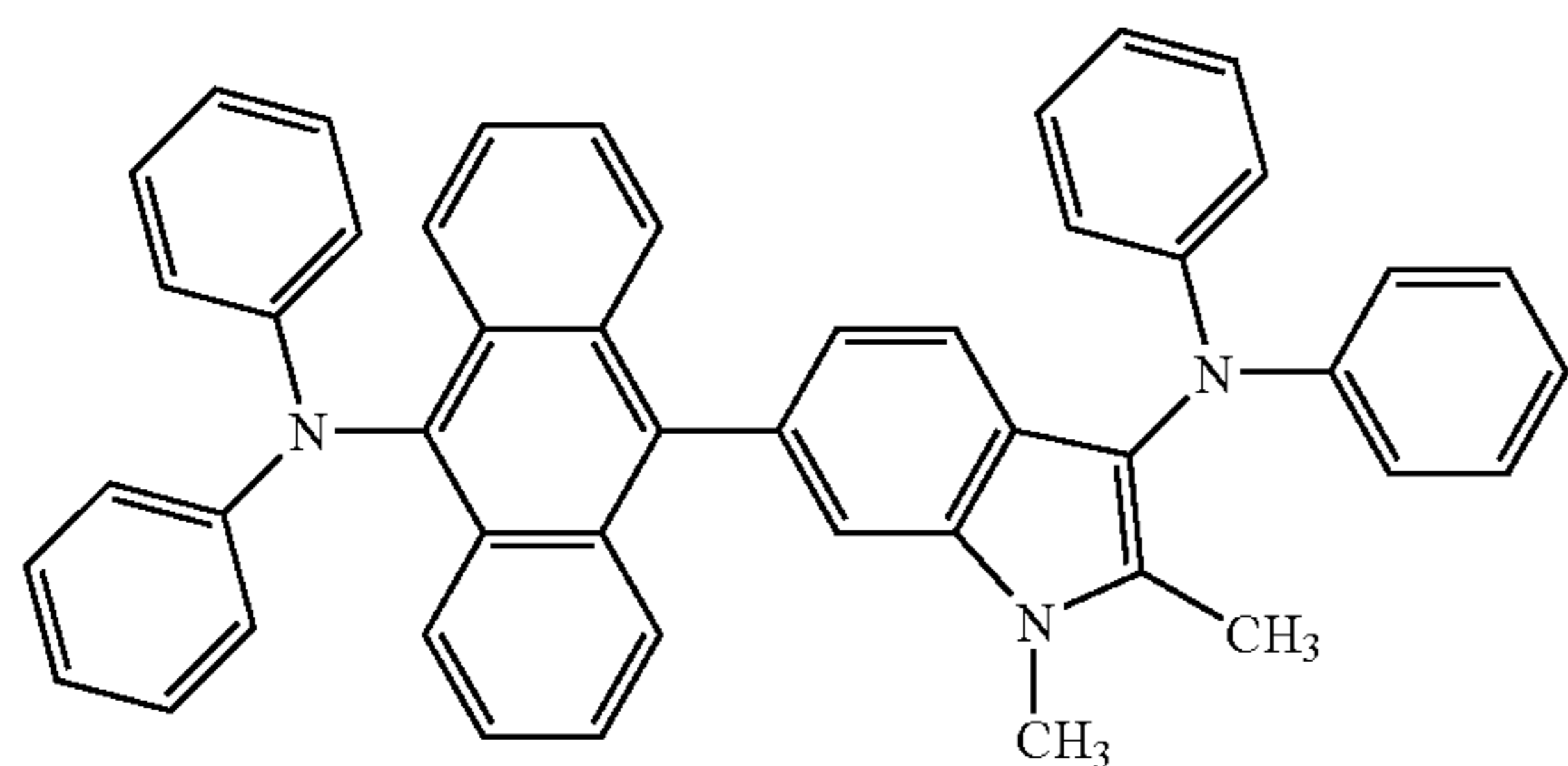
<Formula 65>
