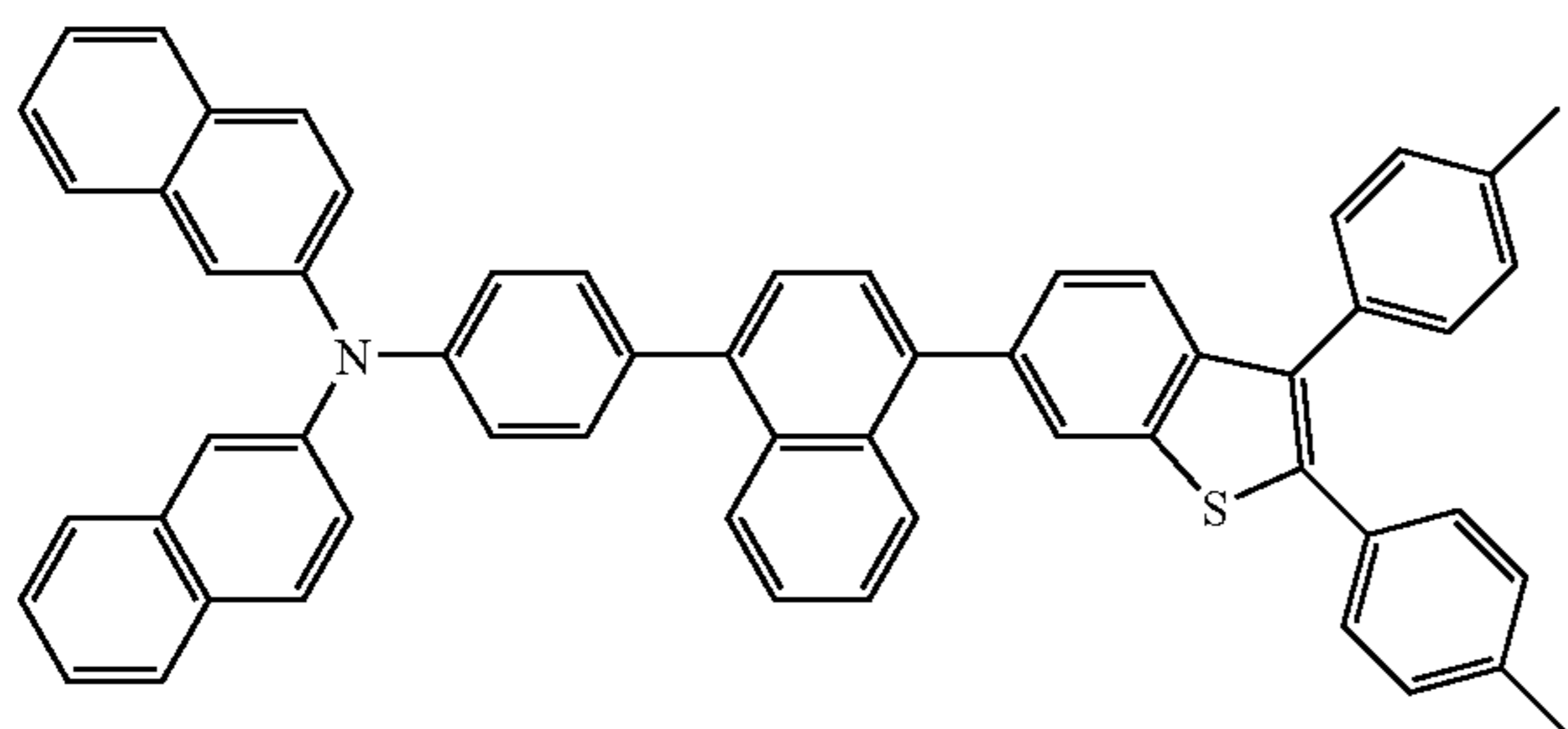
<Formula 27>
