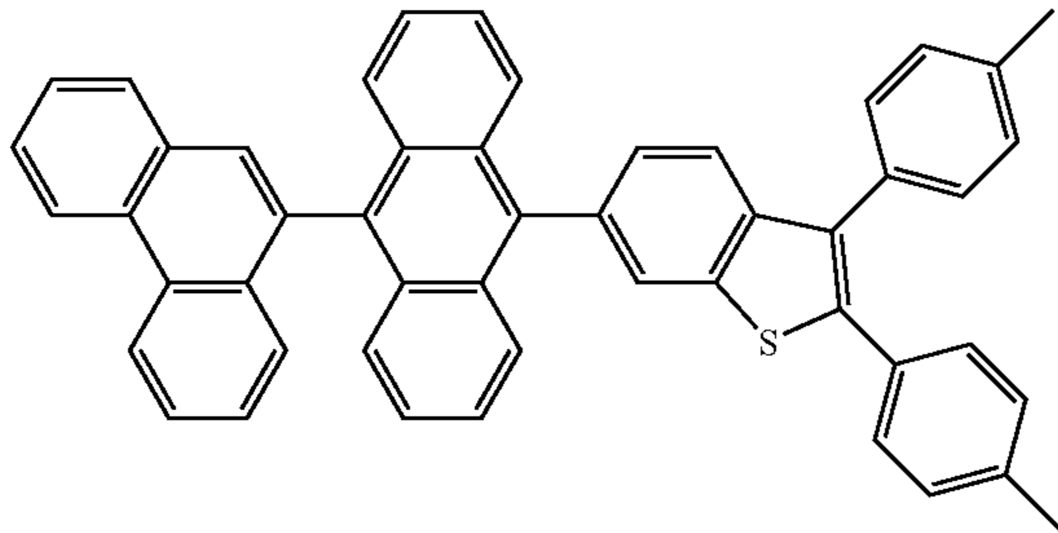
<Formula 8>
