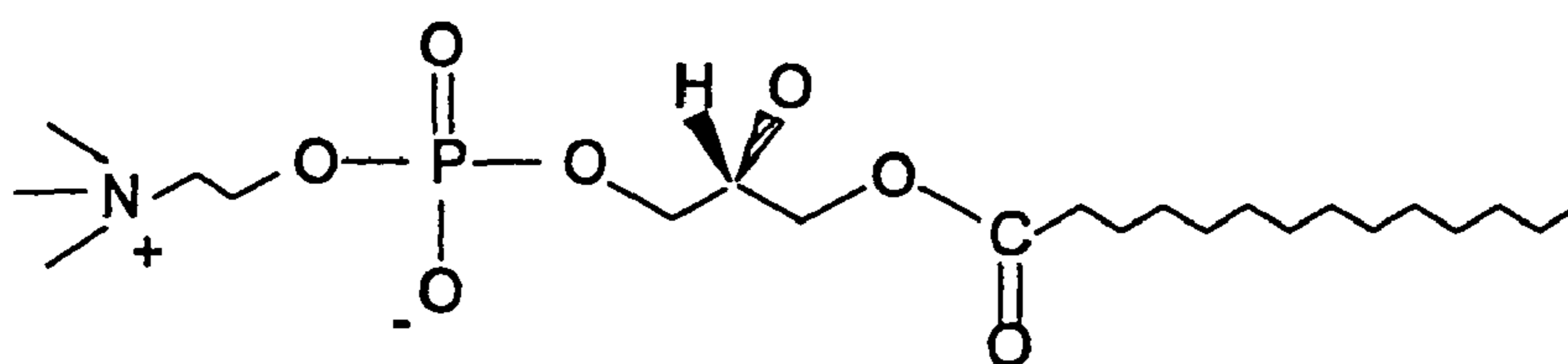
1-Palmitoyl-2-Hydroxy-sn-Glycero-3-Phosphocholine (MPPC)
