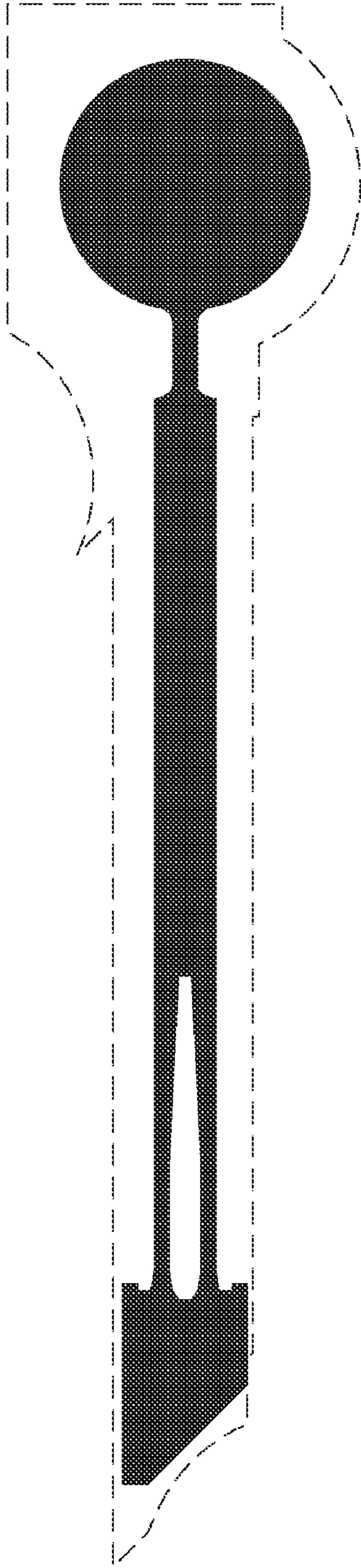
Actuator / bend compensator mask
