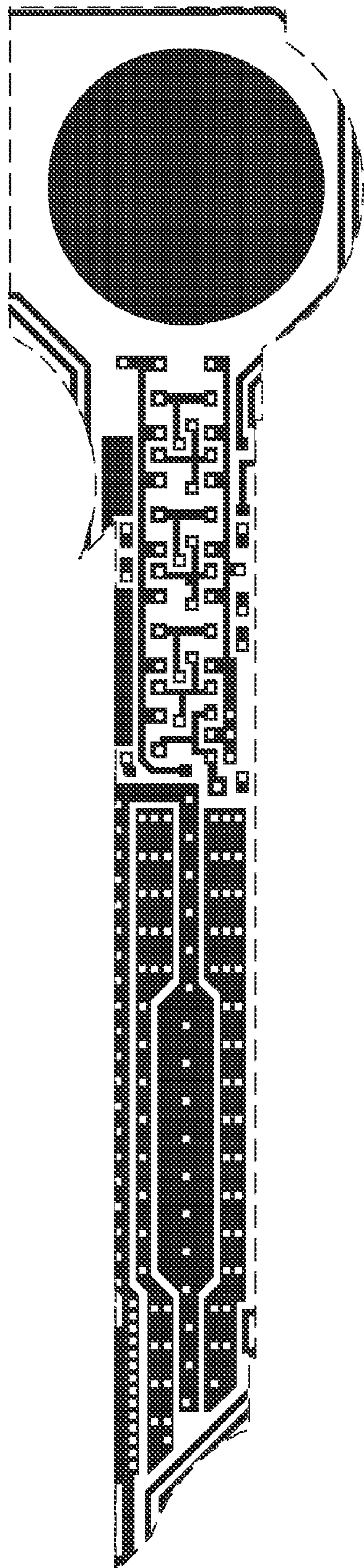
Metal 1 mask
