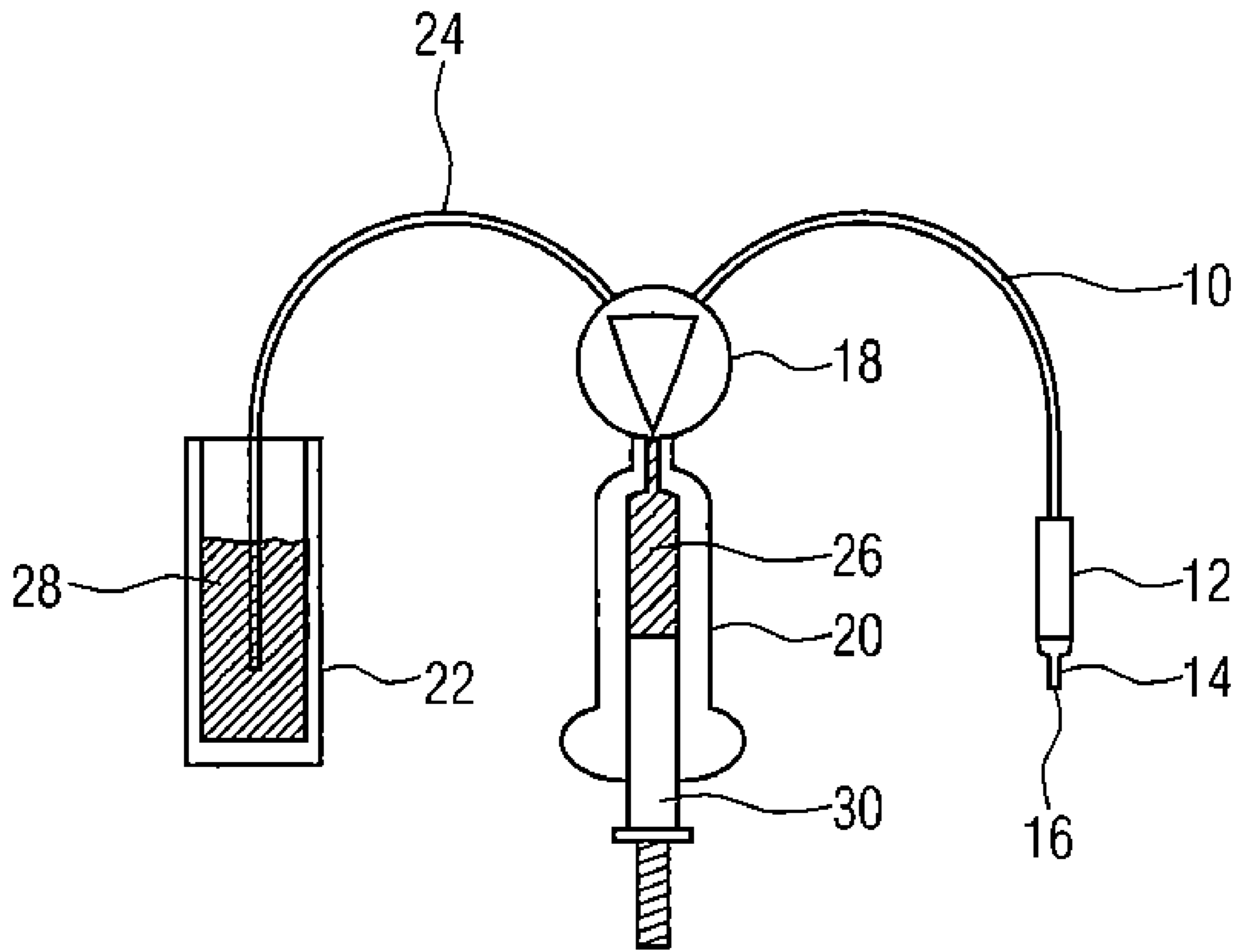
FIG. 8 PRIOR ART
