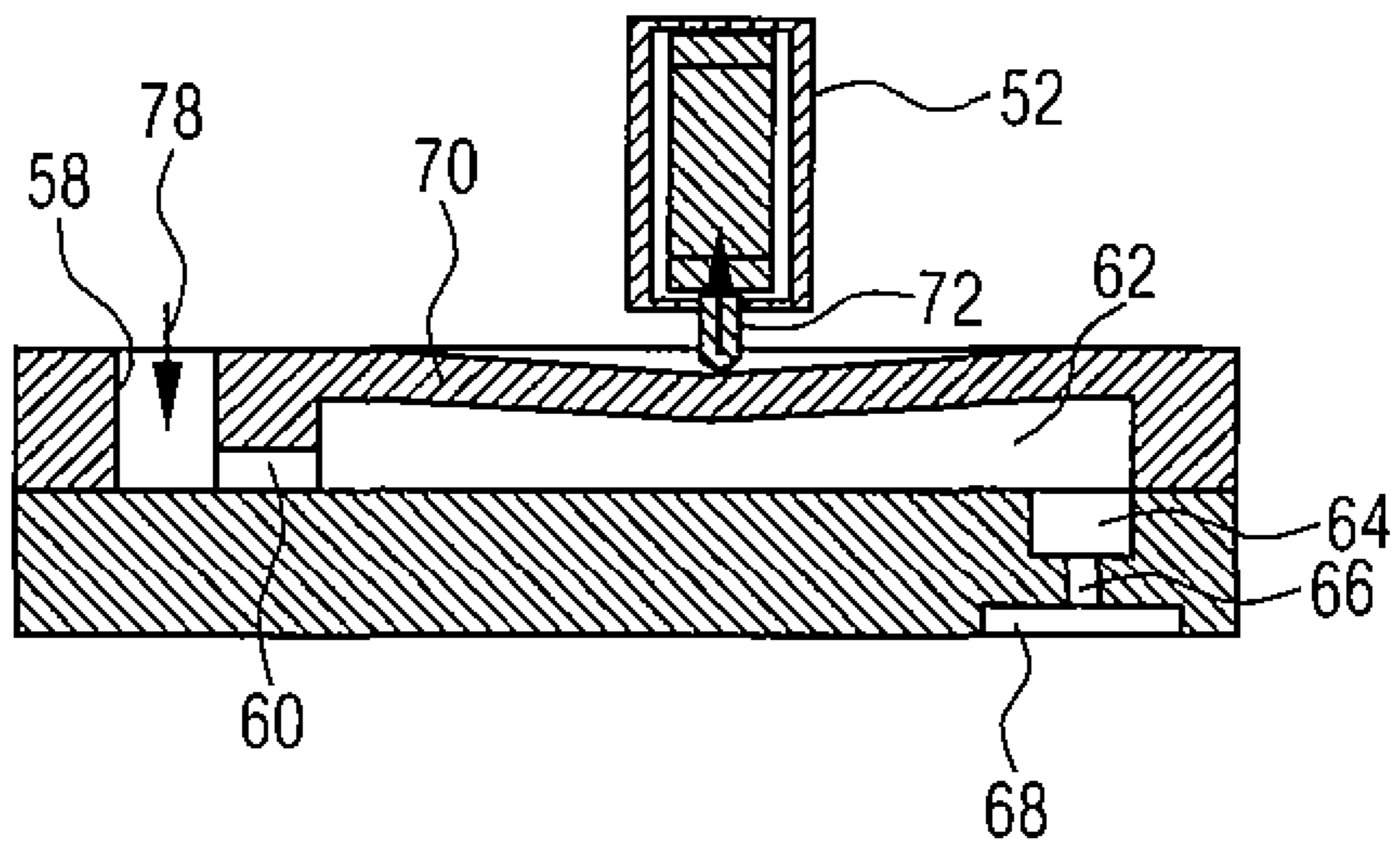
FIG. 9C PRIOR ART
