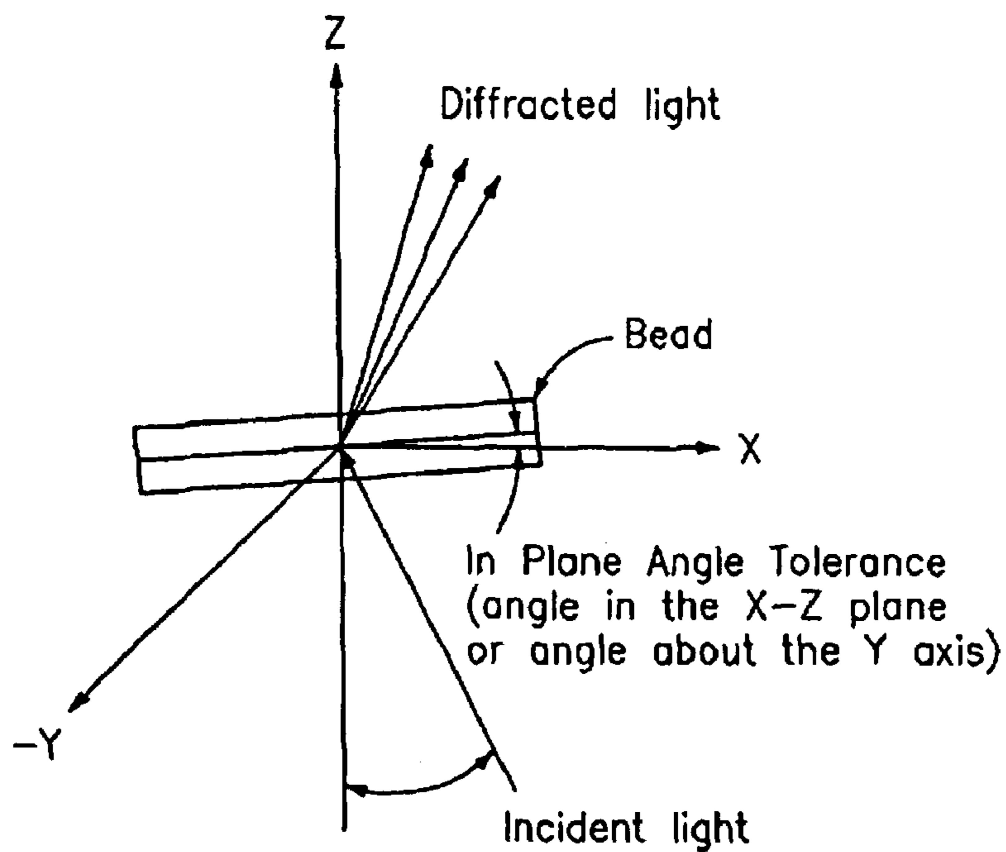
Beam-Bead Alignment, In-Plane Error
