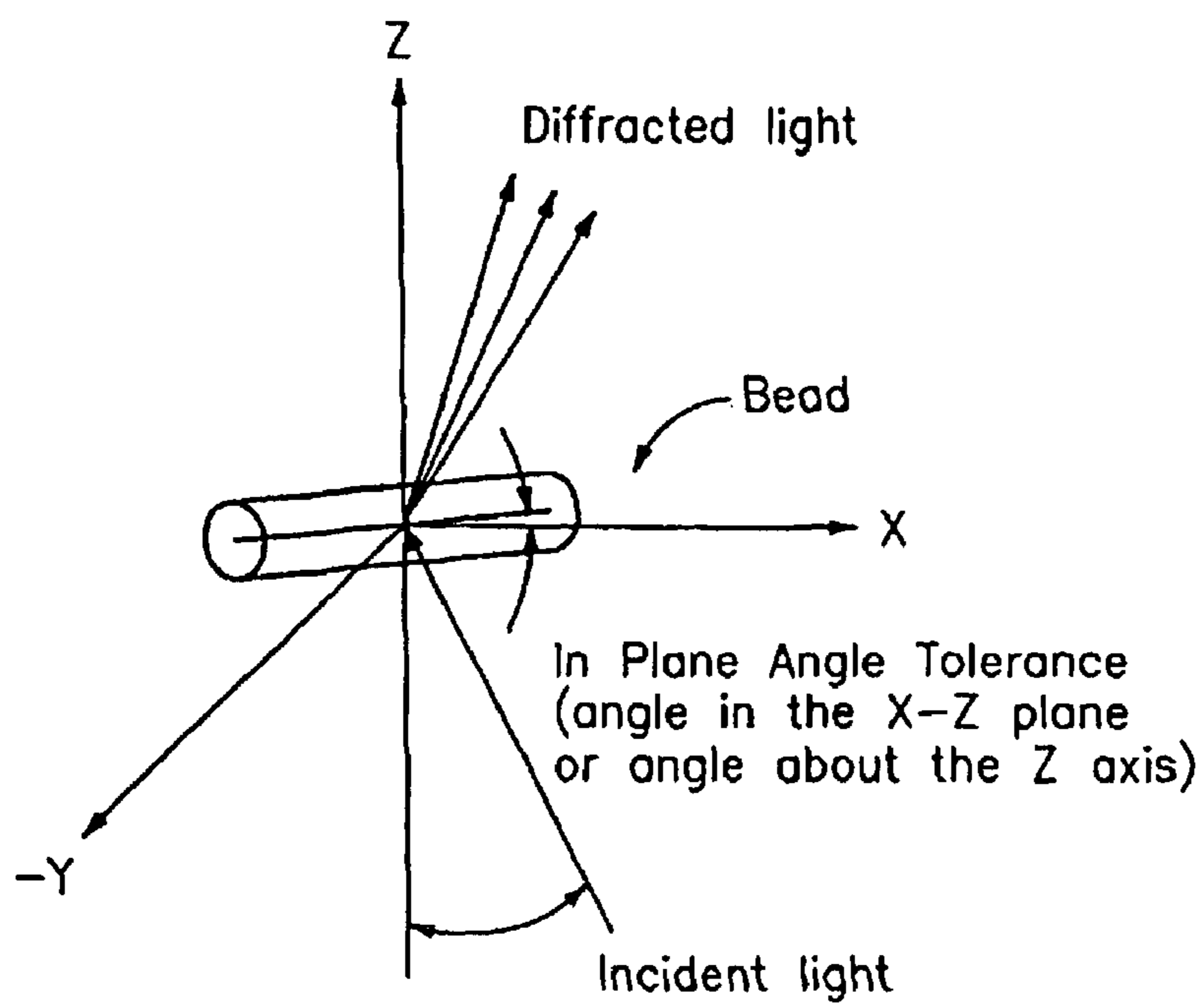
Beam-Bead Alignment, Out-of-Plane Error
