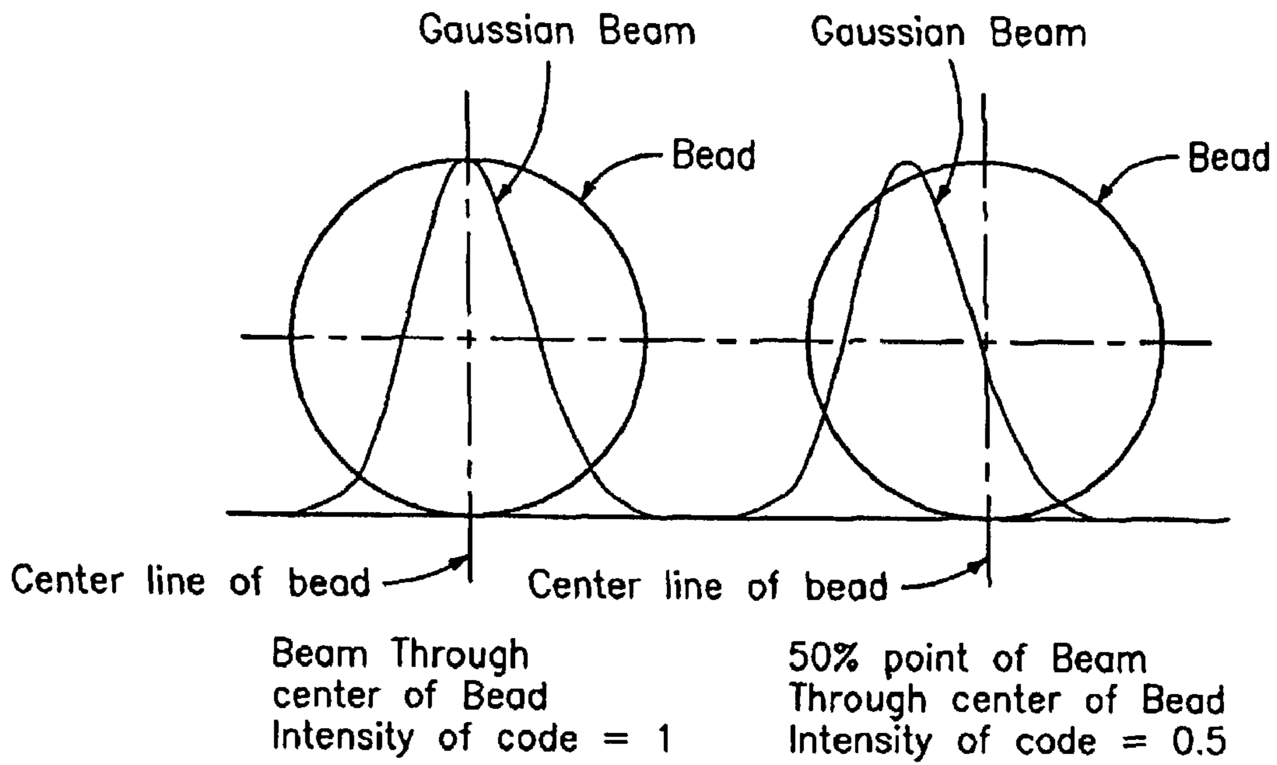
Bead to Beam Position Offset
