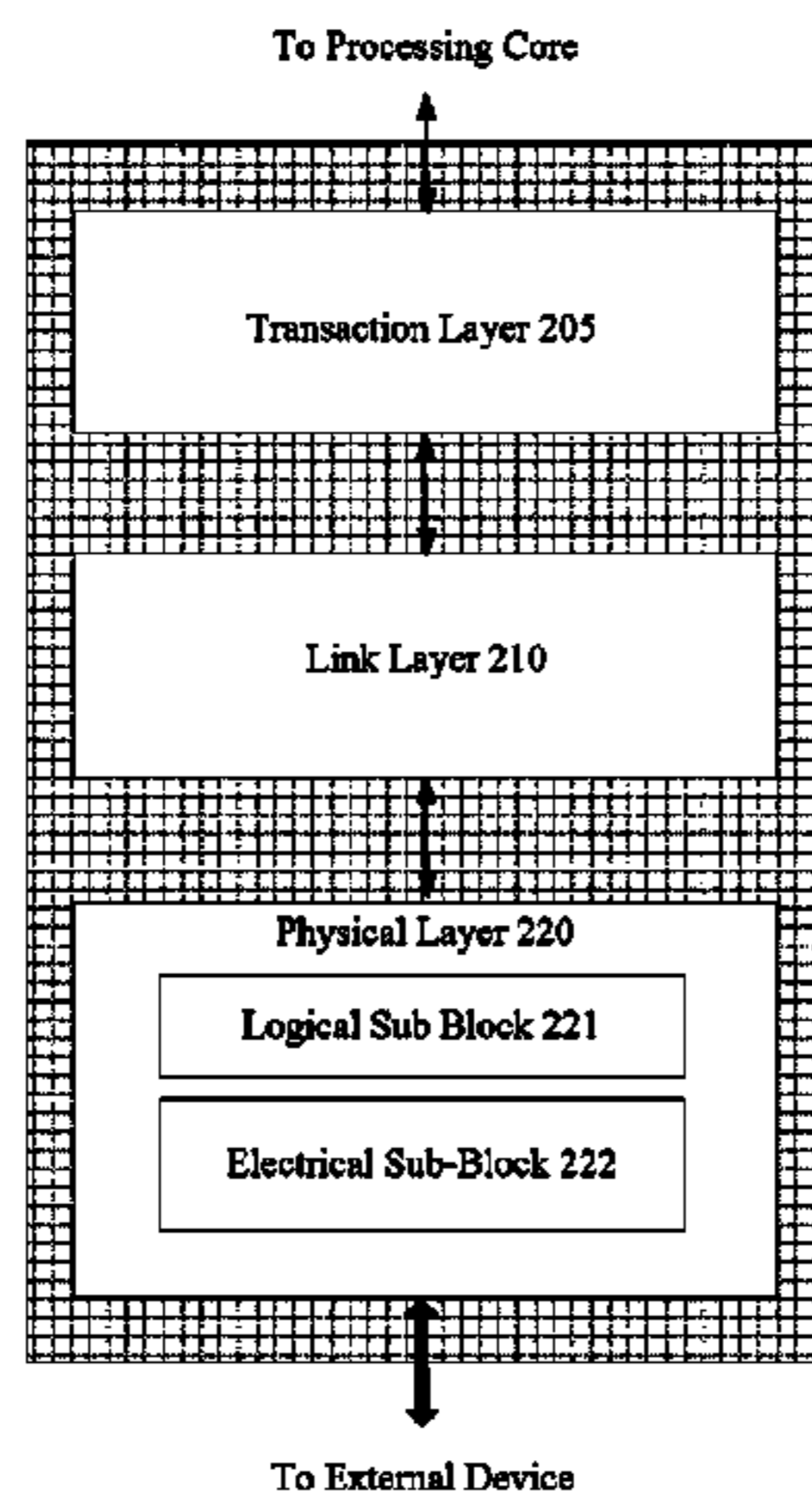
Layered Protocol Stack 200
