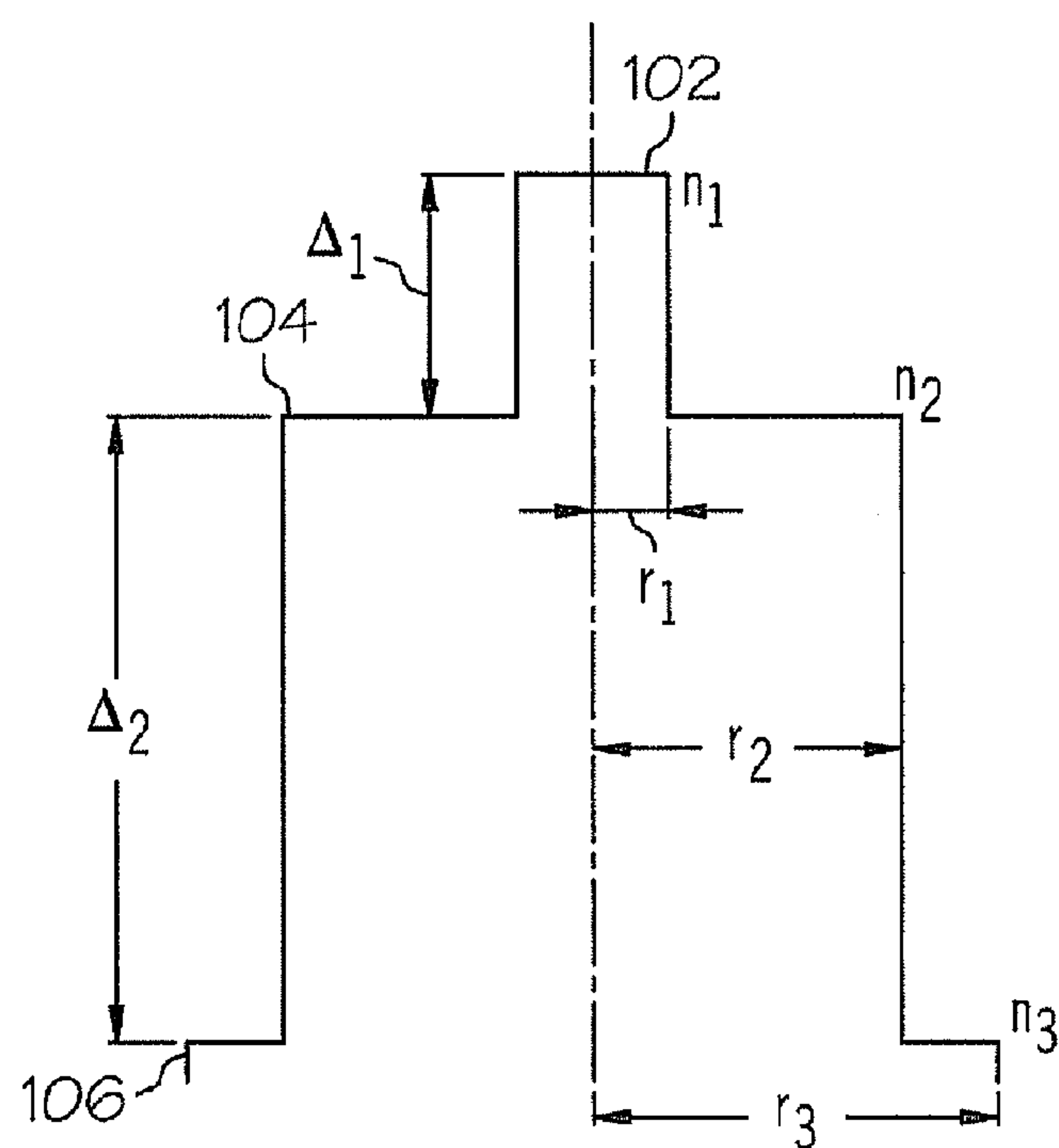
INDEX OF REFRACTION PROFILE
