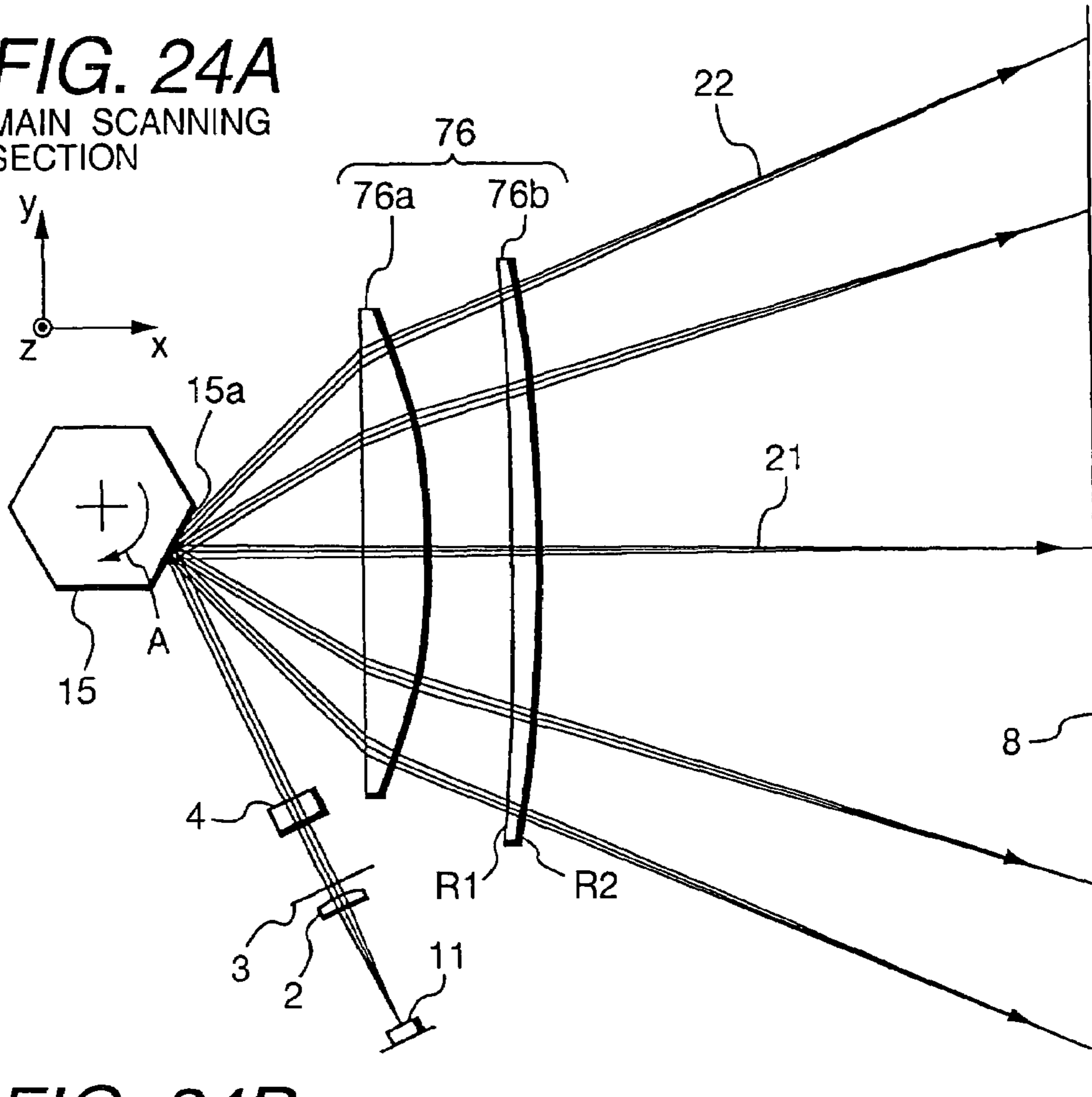
FIG. 24B SUB SCANNING SECTION
