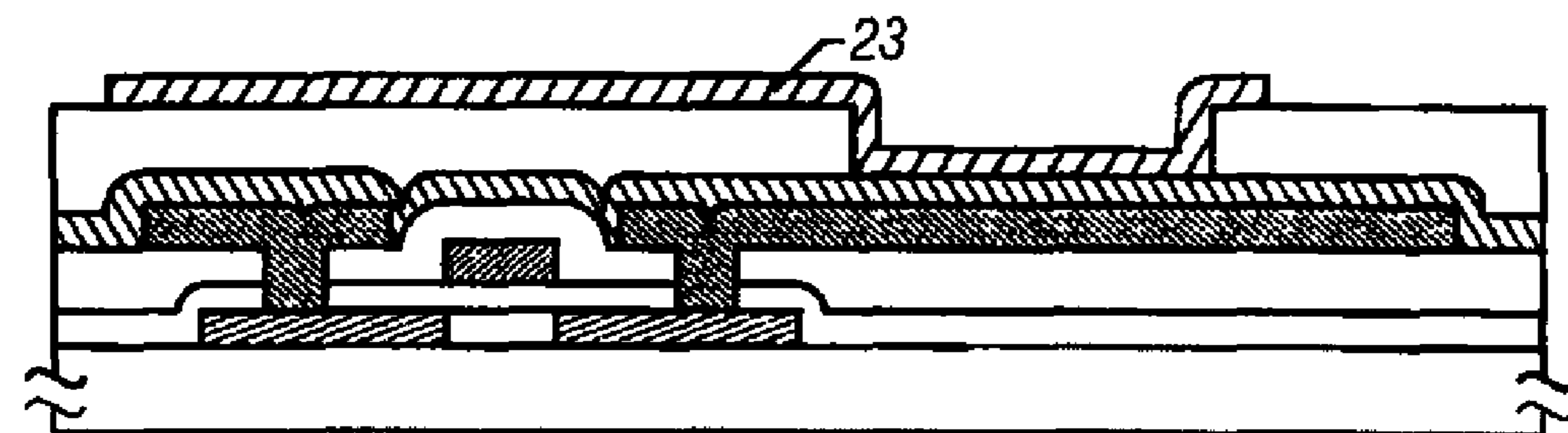
FIG. 3D
