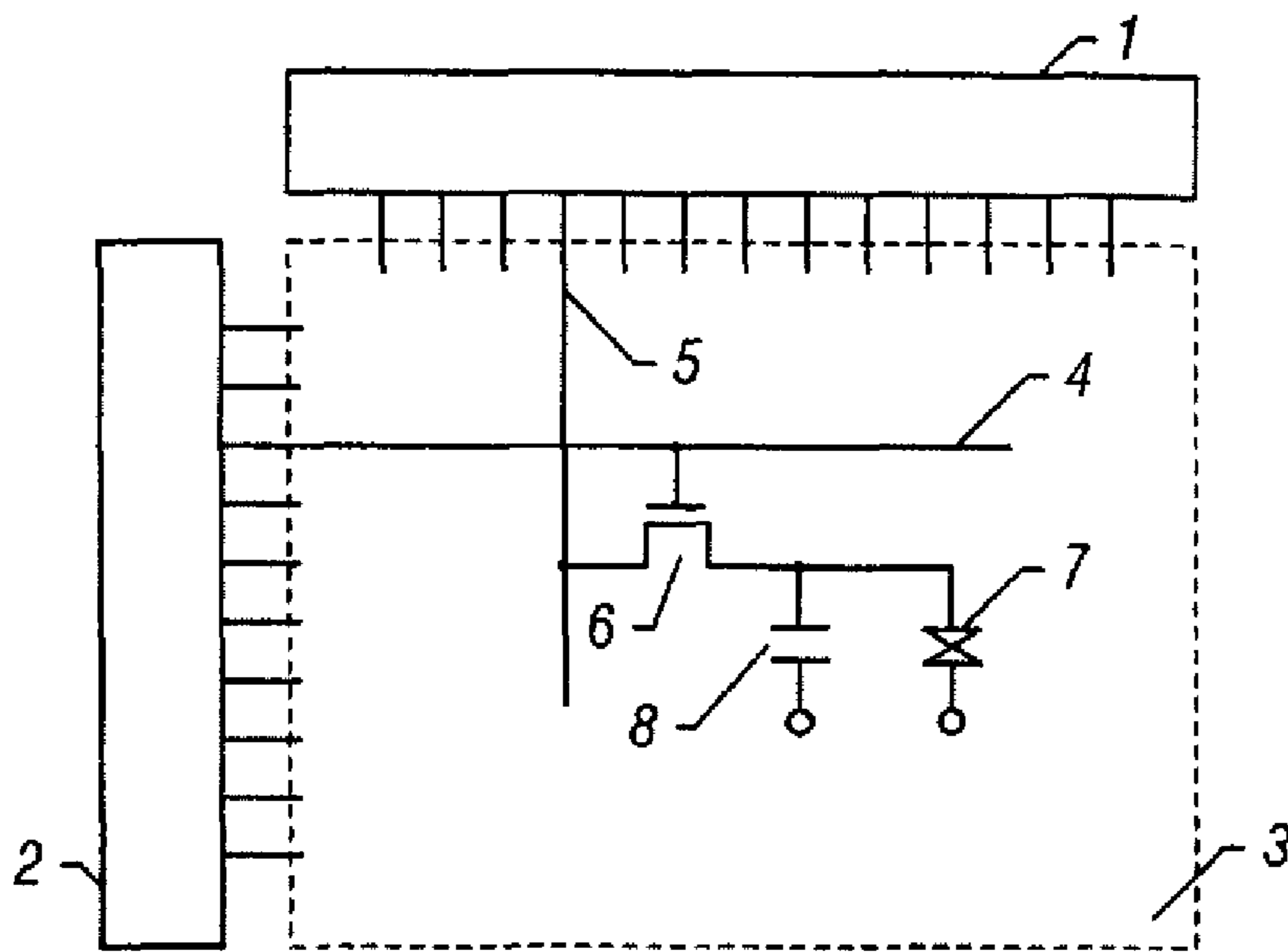
FIG. 1 (Prior Art)
