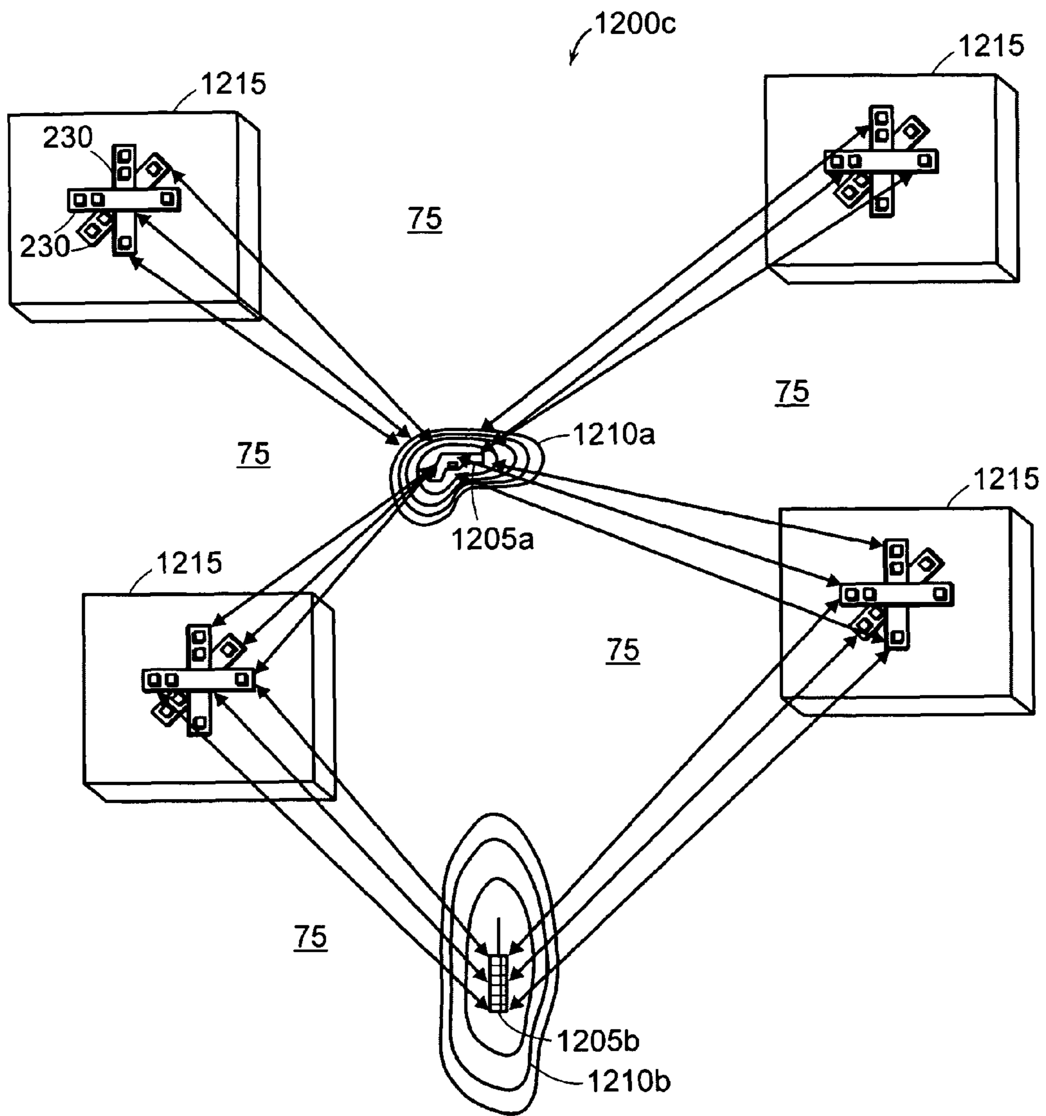
(Top View) FIG. 12C
