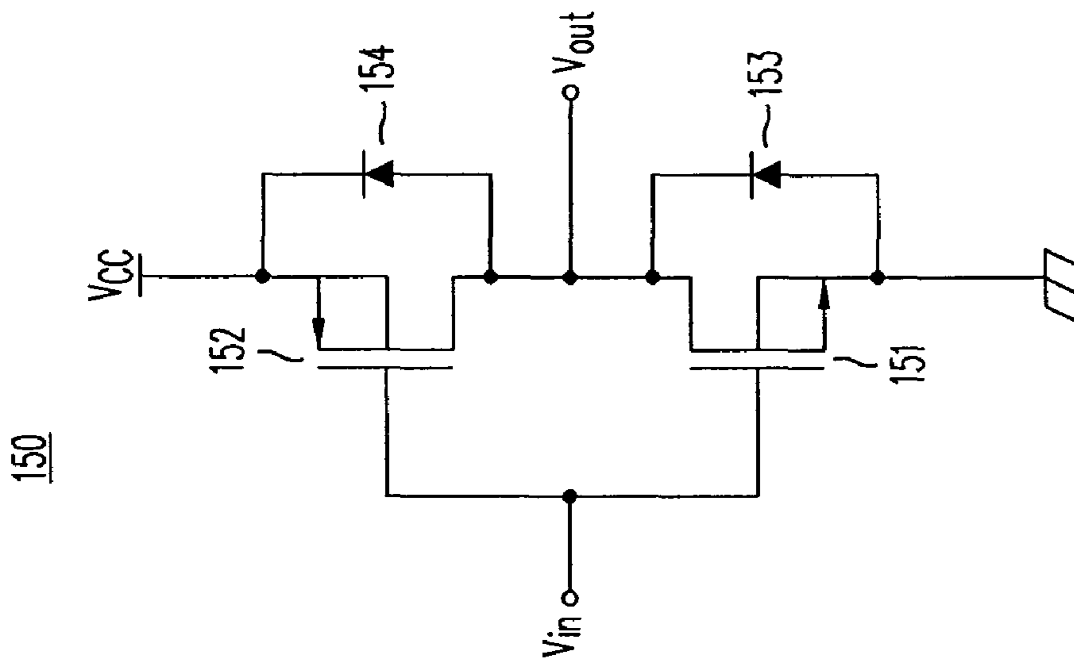
FIG. 3C (Prior Art)
