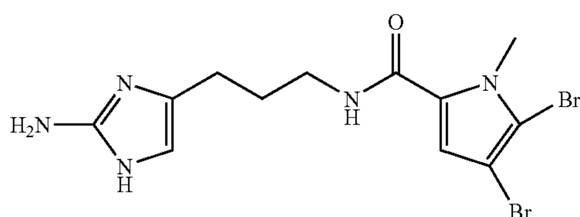
Dihydrosventrin (DHS)
