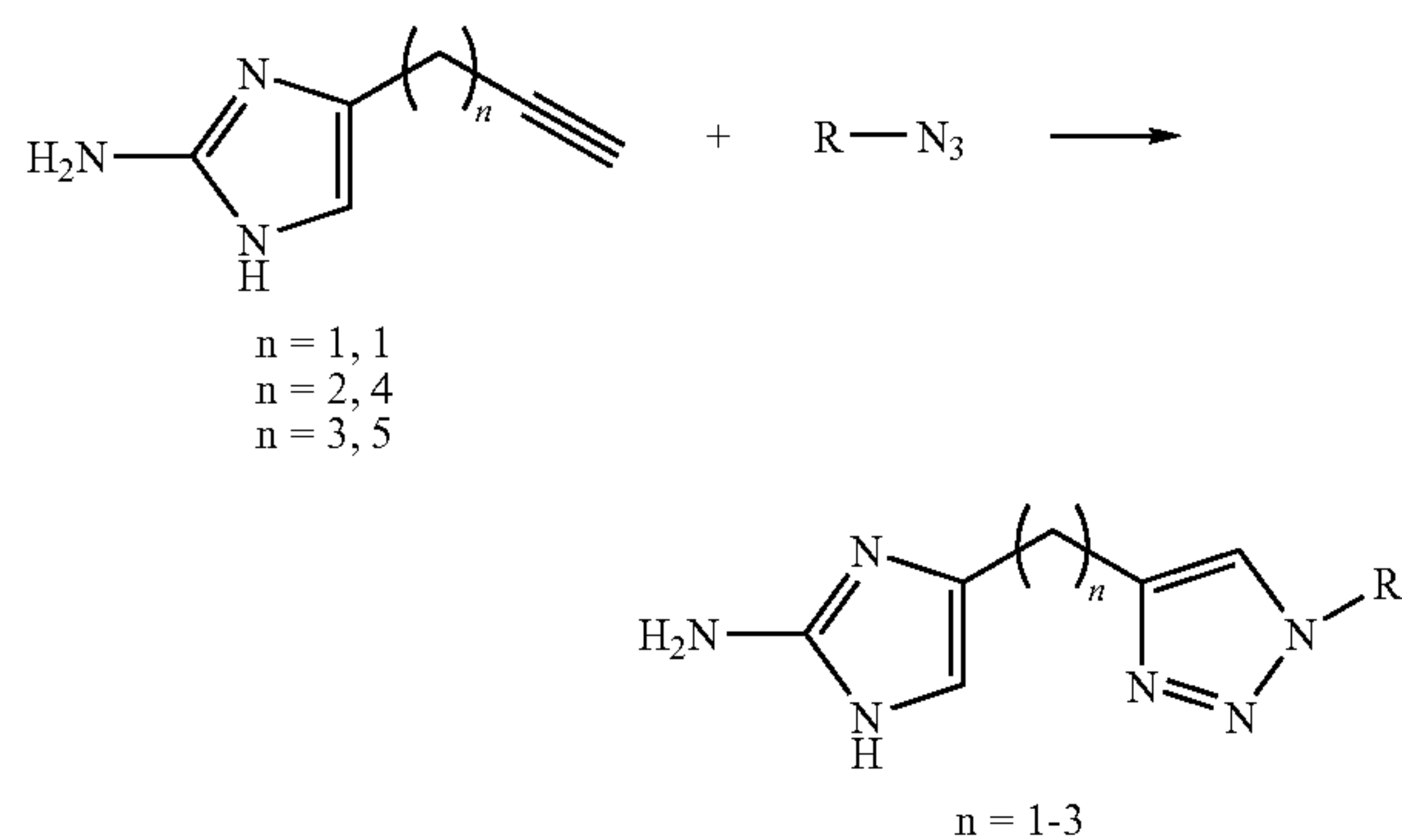
Scheme 1. Construction of the initial 2-AIT library.
