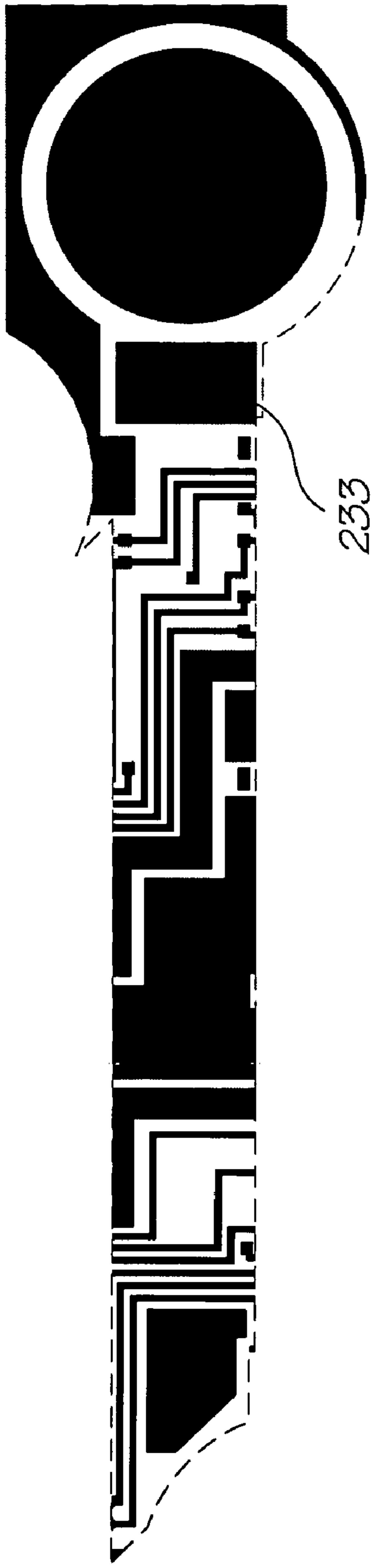
Metal 2 mask
