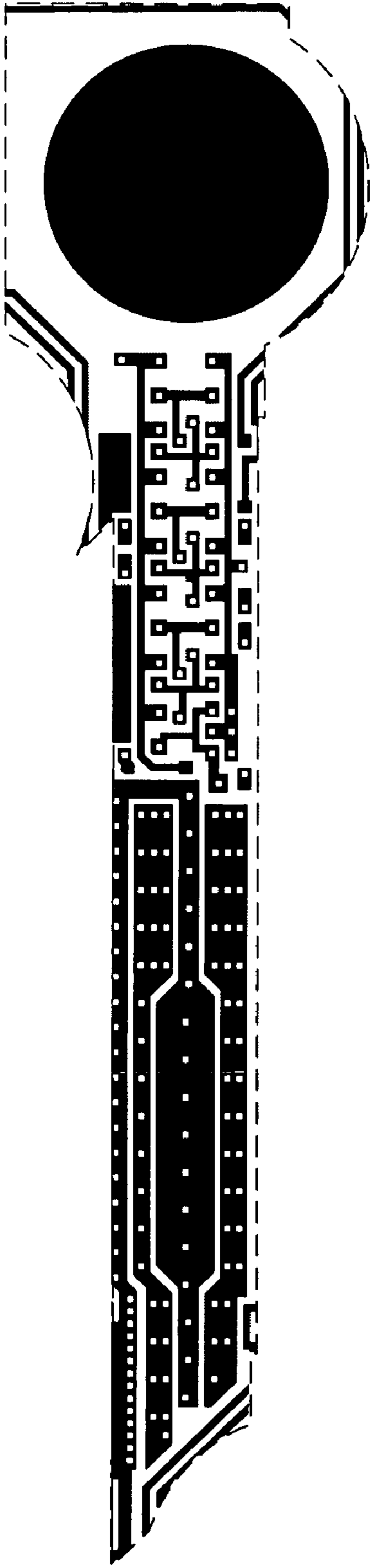
Metal 1 mask
