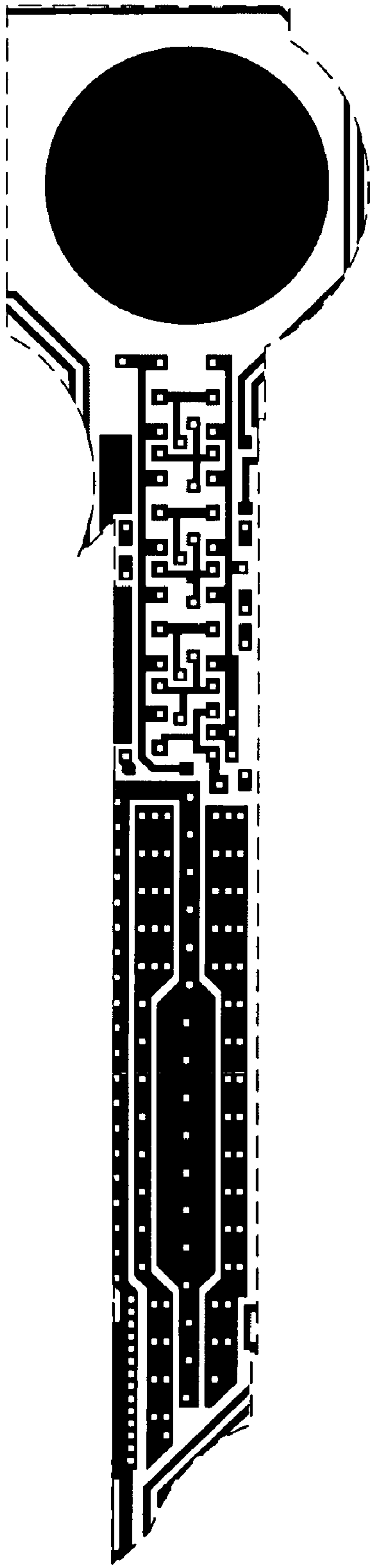
Metal 1 mask
