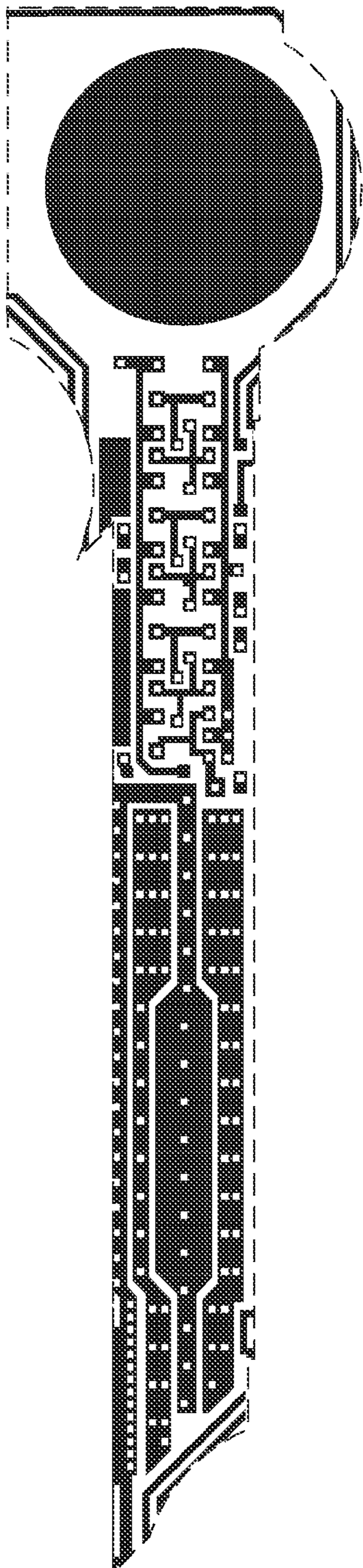
Metal 1 mask
