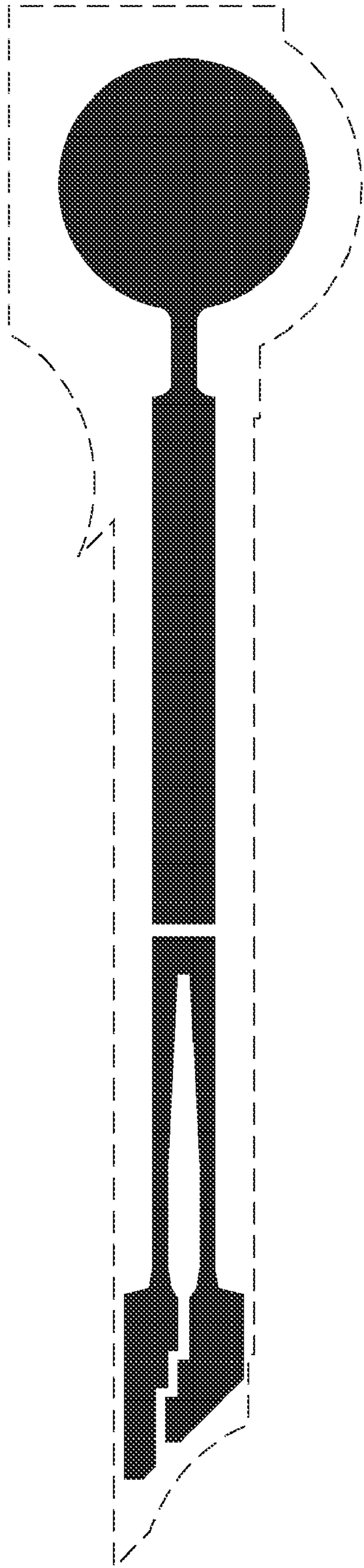
Heater mask
