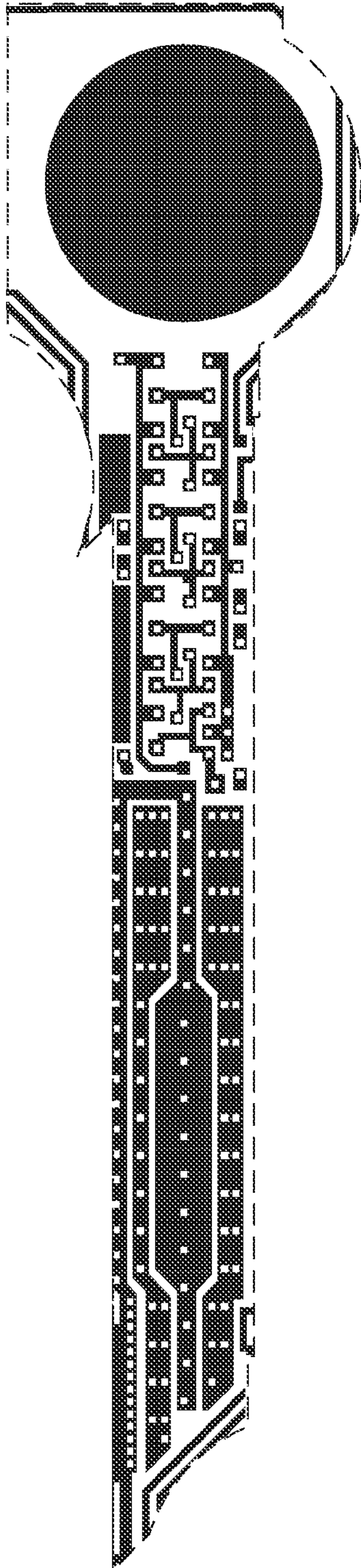
Metal 1 mask
