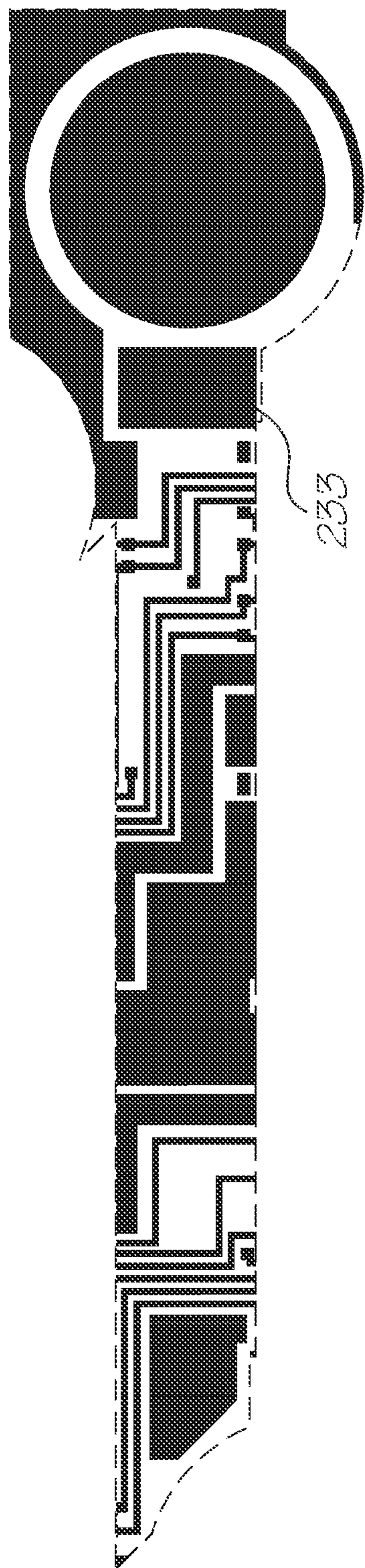
Metal 2 mask
