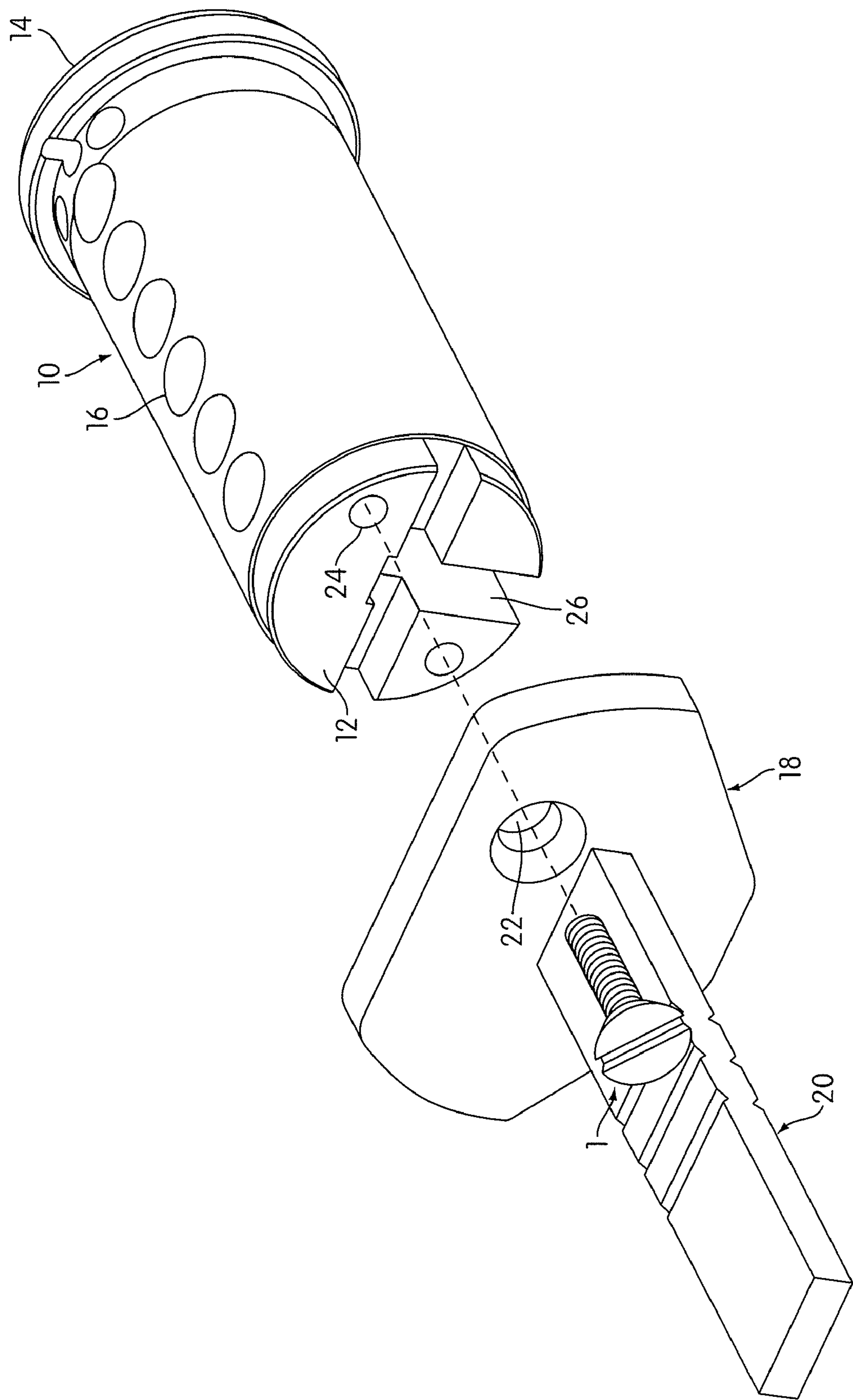
FIG. 1 PRIOR ART
