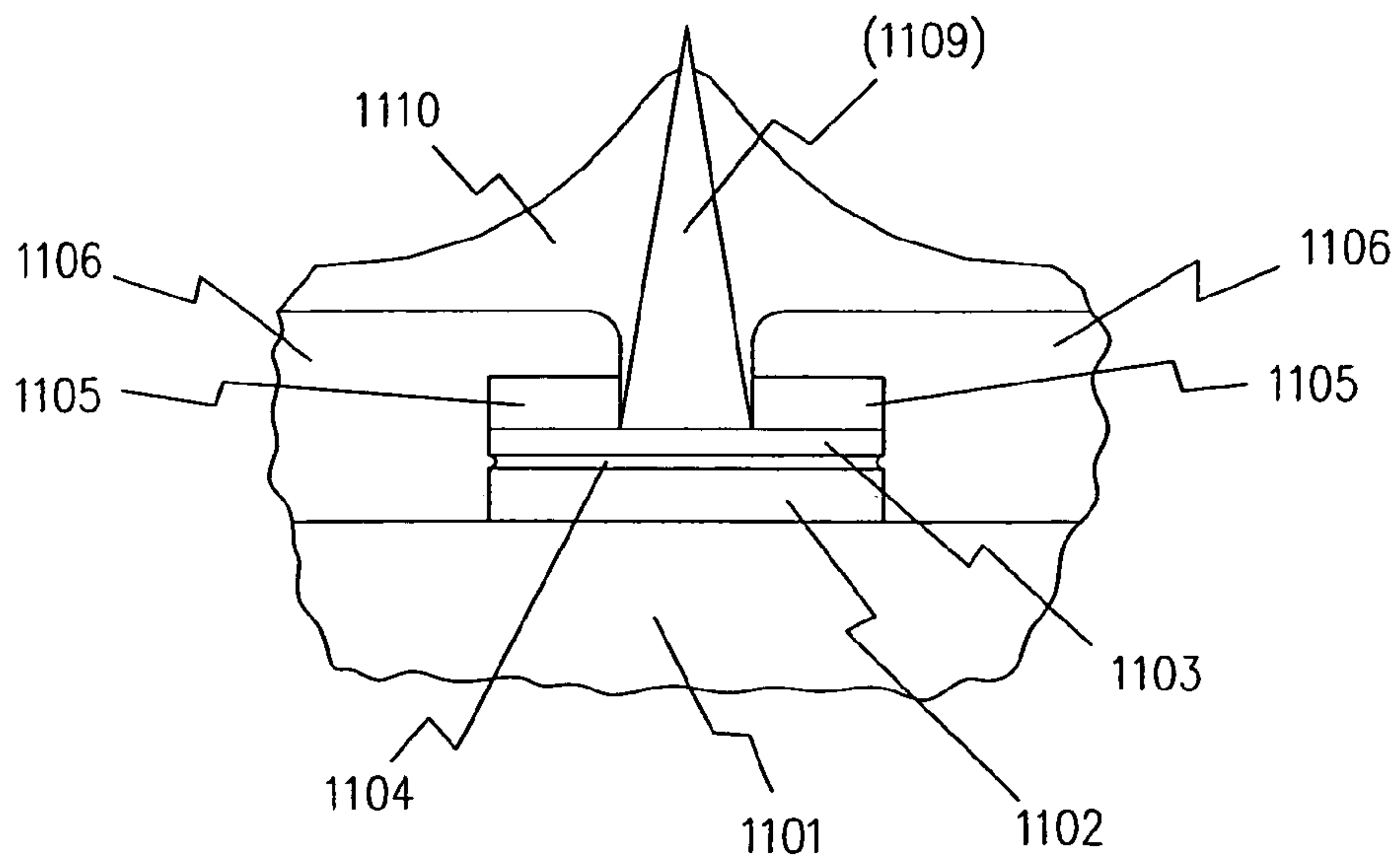
FIGURE 11b ELECTRODES
