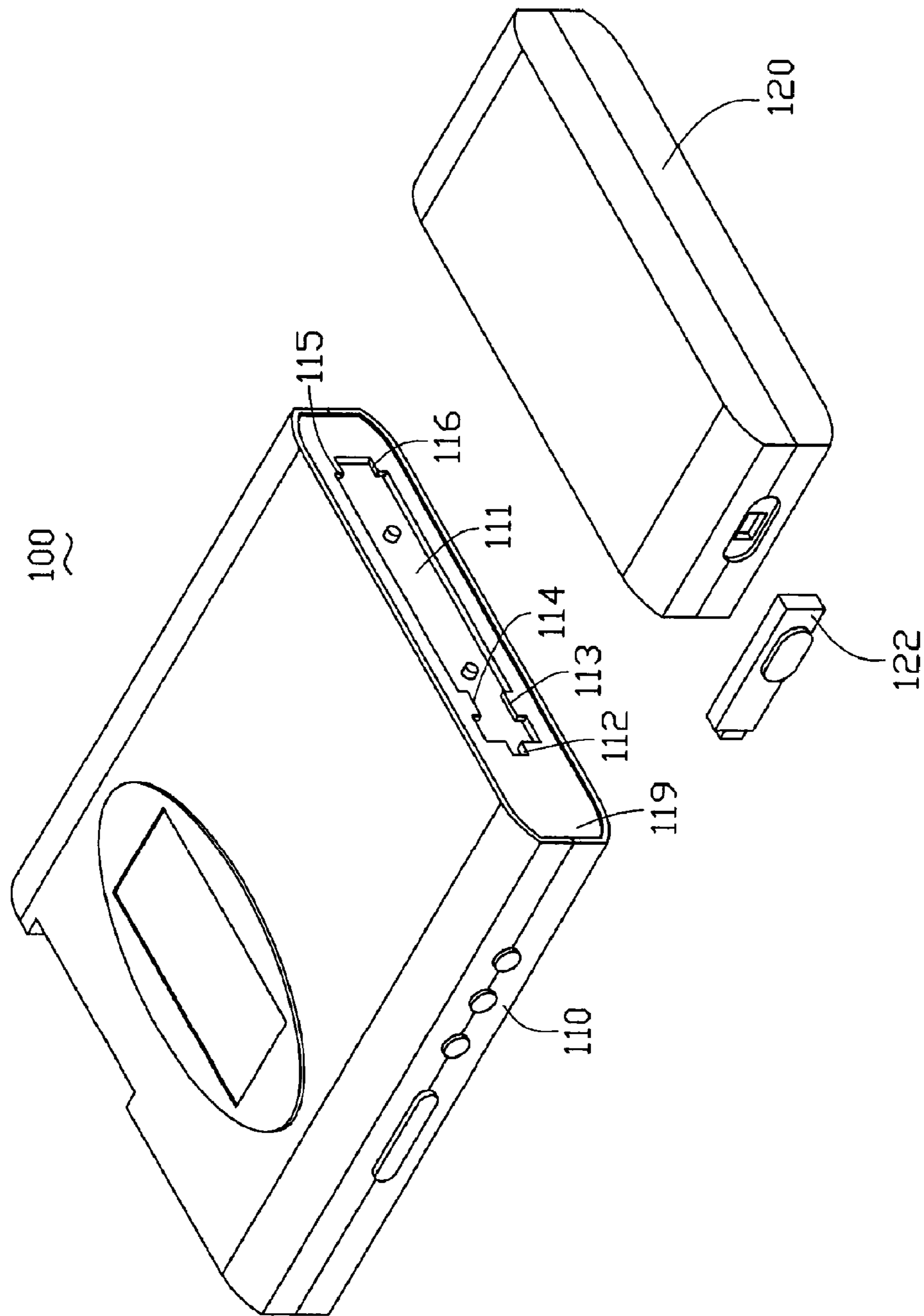
FIG. 6 (RELATED ART)
