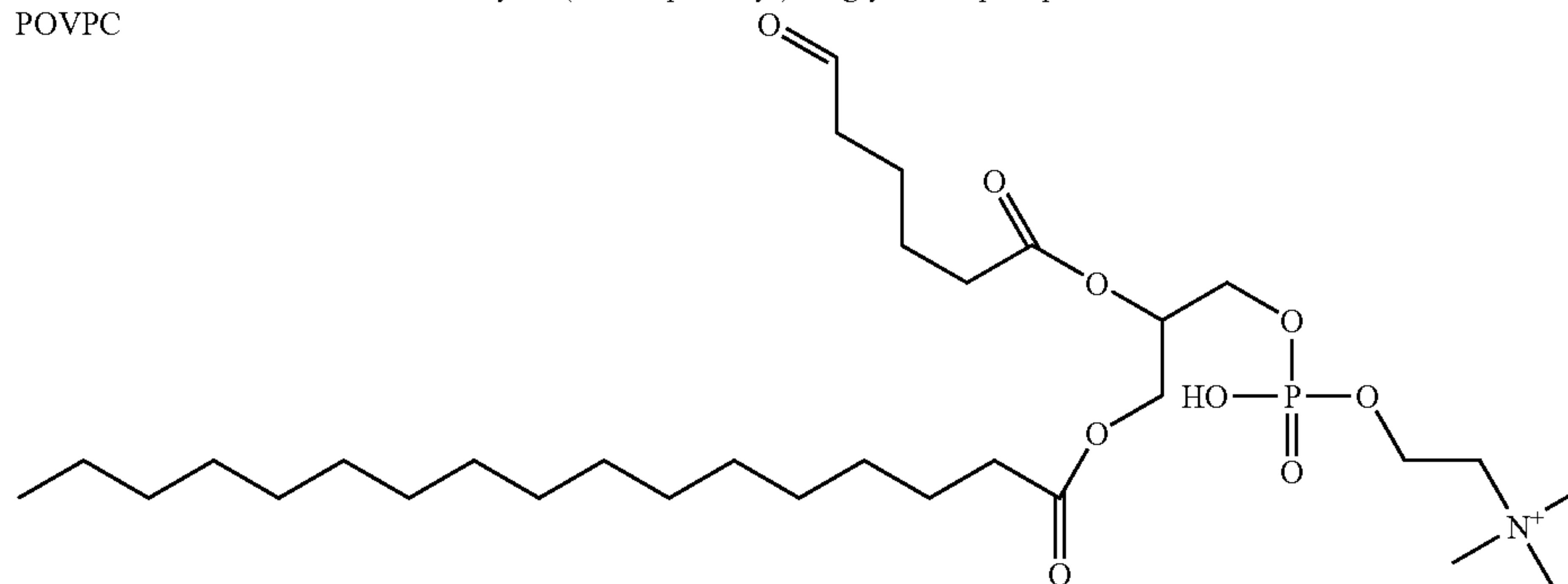
1-hexadecanoyl-2-(5'-oxo-pentanoyl)-sn-3-phosphocholine
