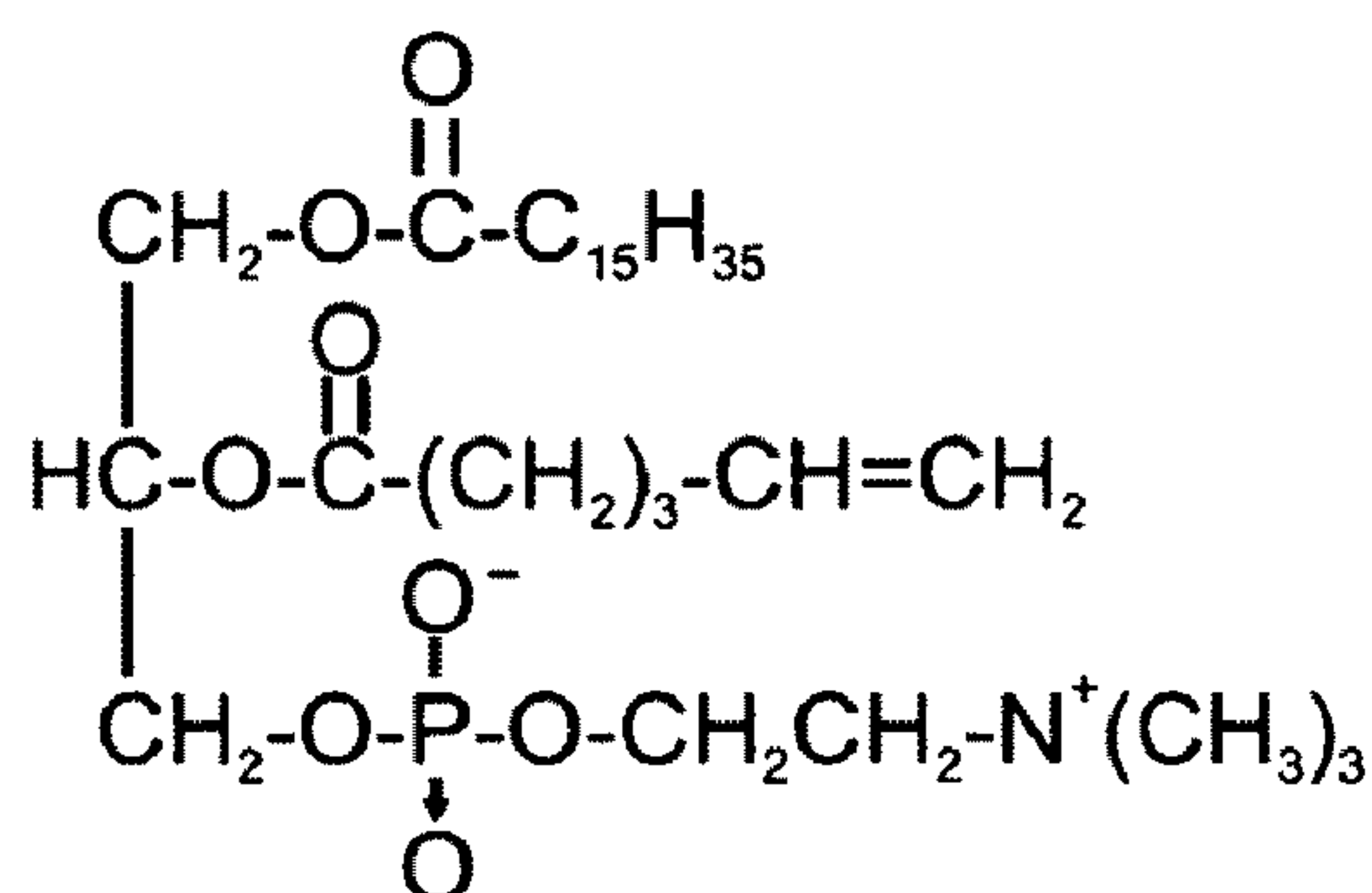
1-Hexadecanoyl-2-(5'-hexenoyl) sn-3-glycerophosphocholine
