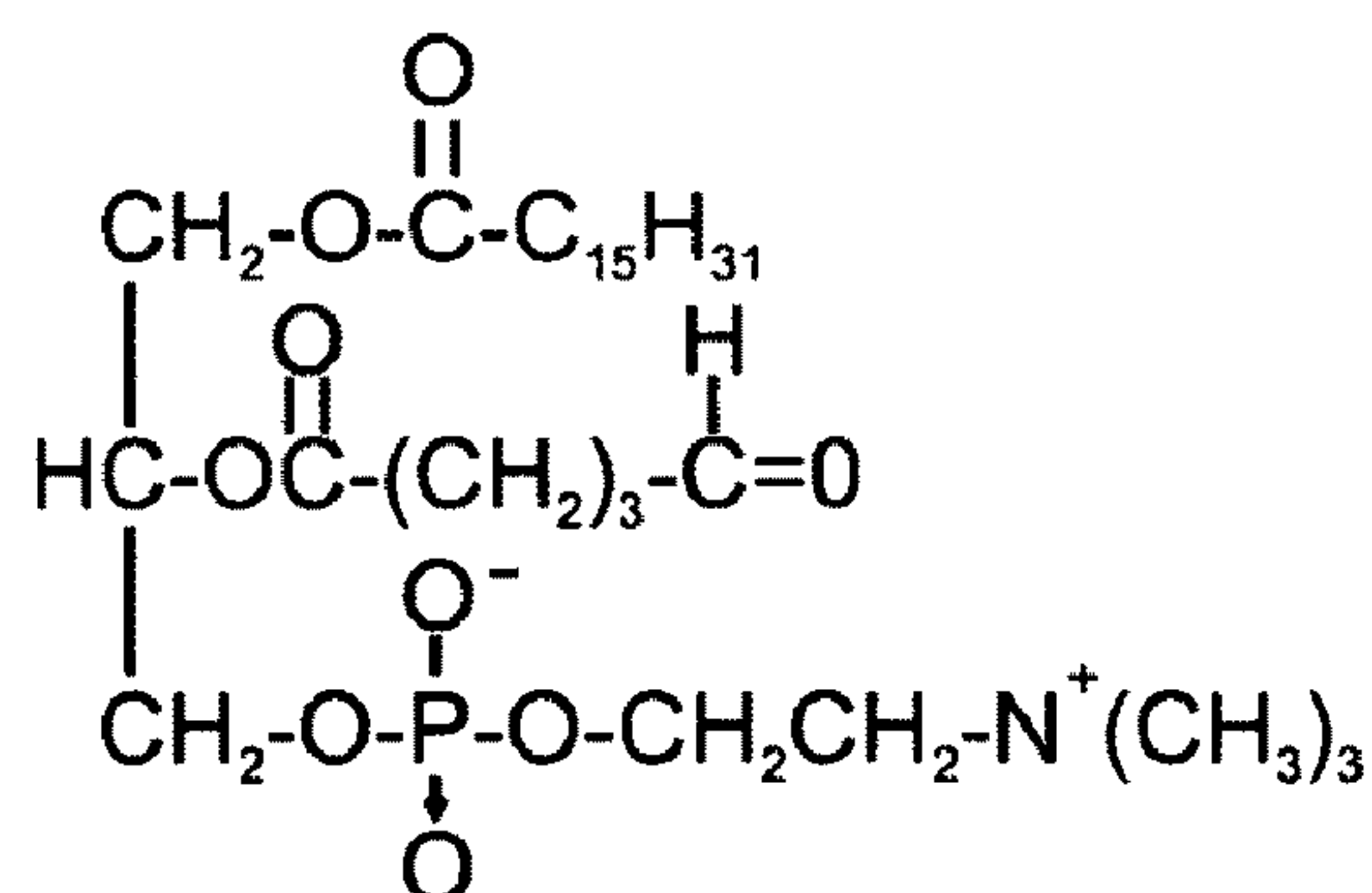
POVPC 1-Hexadecanoyl-2-(5'-oxopentanoyl)- sn-3-glycerophosphocholine
