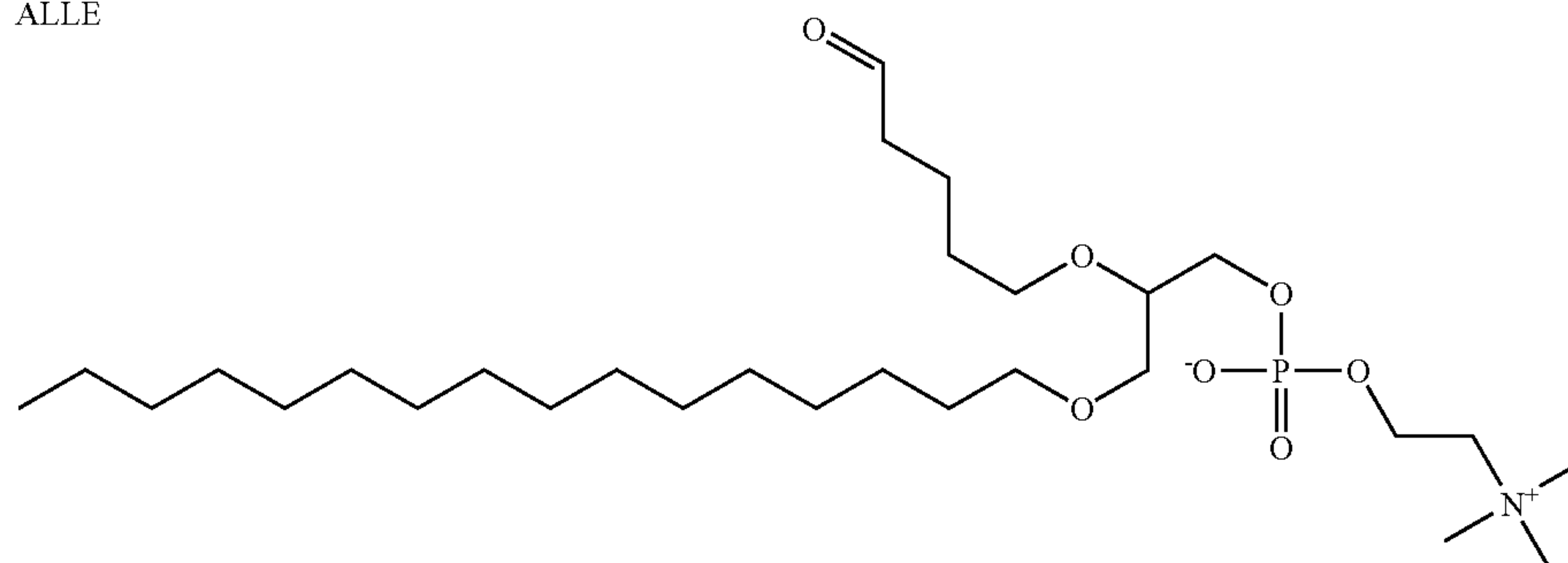
1-hexadecyl-2-(5'-oxo-pentanyl)-sn-glycero-3-phosphocholine
