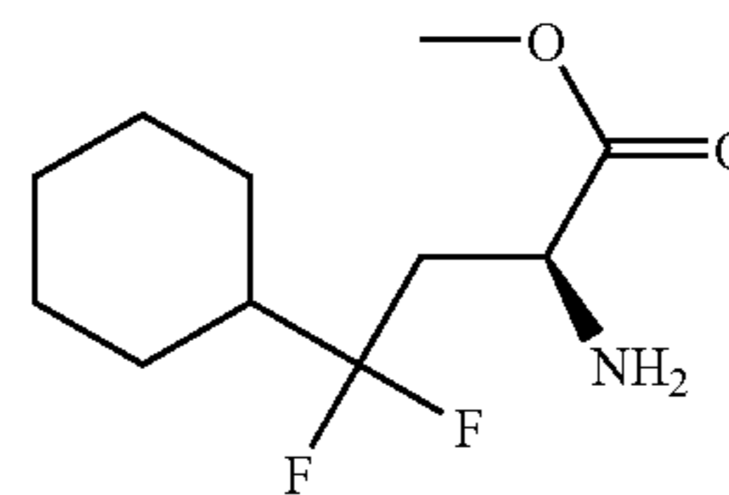
(S)-methyl 2-amino-4-cyclohexyl-4,4-difluorobutanoate
