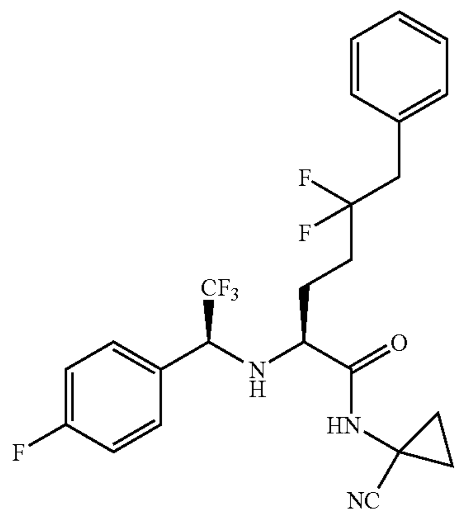
Synthesis Example 8
