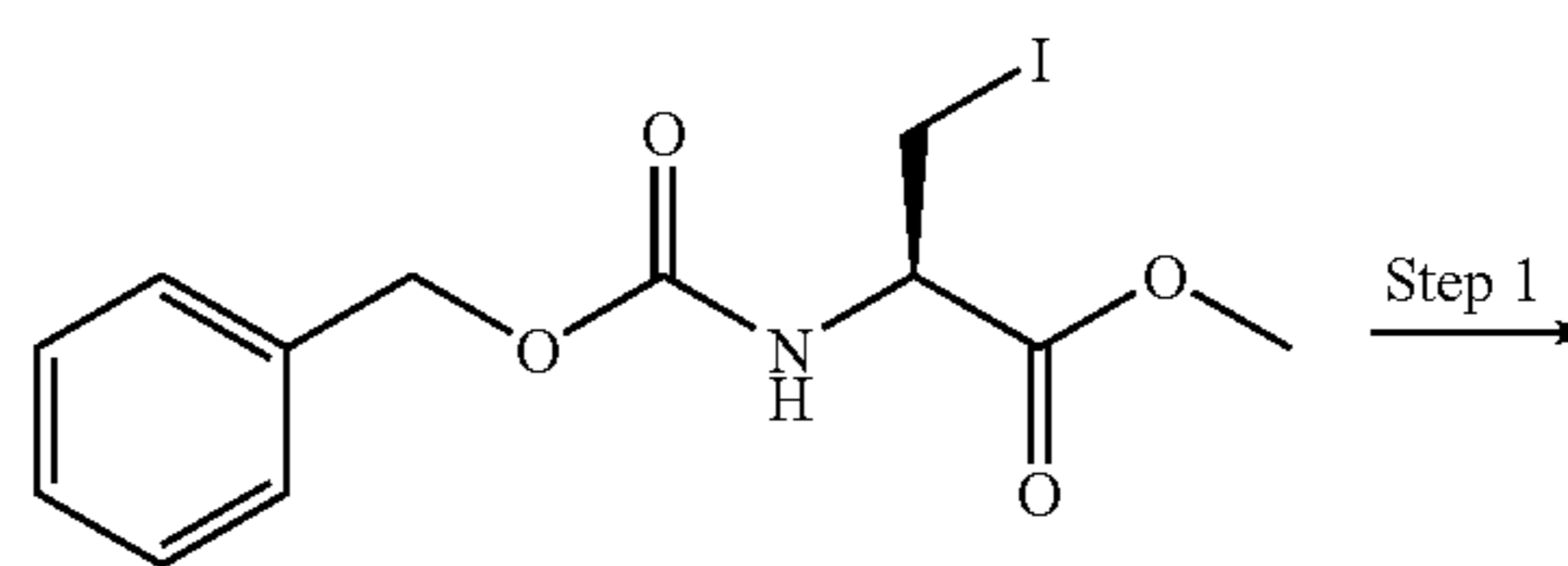
Scheme 3
