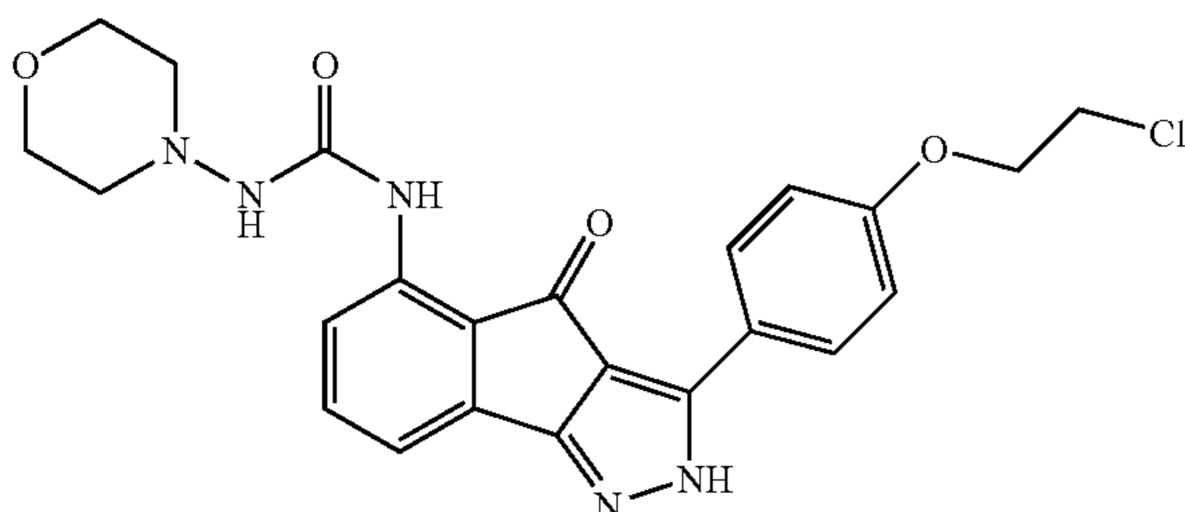
Synthesis of 1-(3-[4-(2-chloroethoxy)phenyl]-4-oxo-2,4-dihydroindeno[1,2-c]pyrazol-5-yl)-3-morpholin-4-yl urea
