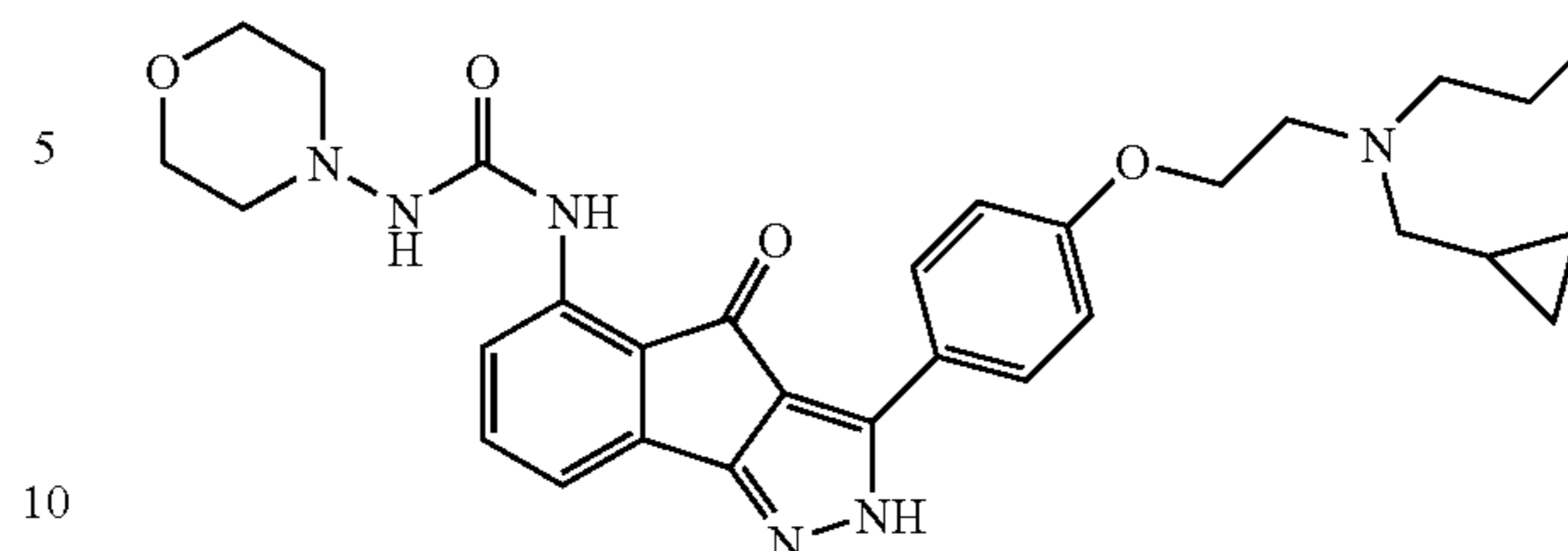
Synthesis of 1-(3-{4-[2-(cyclopropylmethyl-propylamino)ethoxy]phenyl}-4-oxo-2,4-dihydroindeno[1,2-c]pyrazol-5-yl)-3-morpholin-4-yl urea
