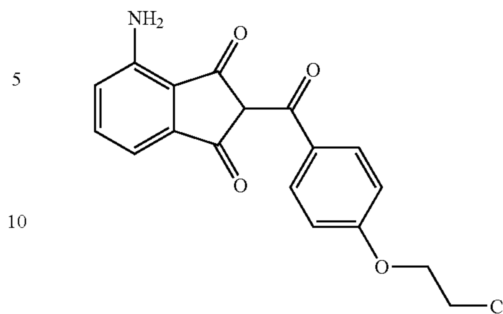
Synthesis of 4-Amino-2-[4-(2-chloroethoxy)benzoyl]indan-1,3-dione
