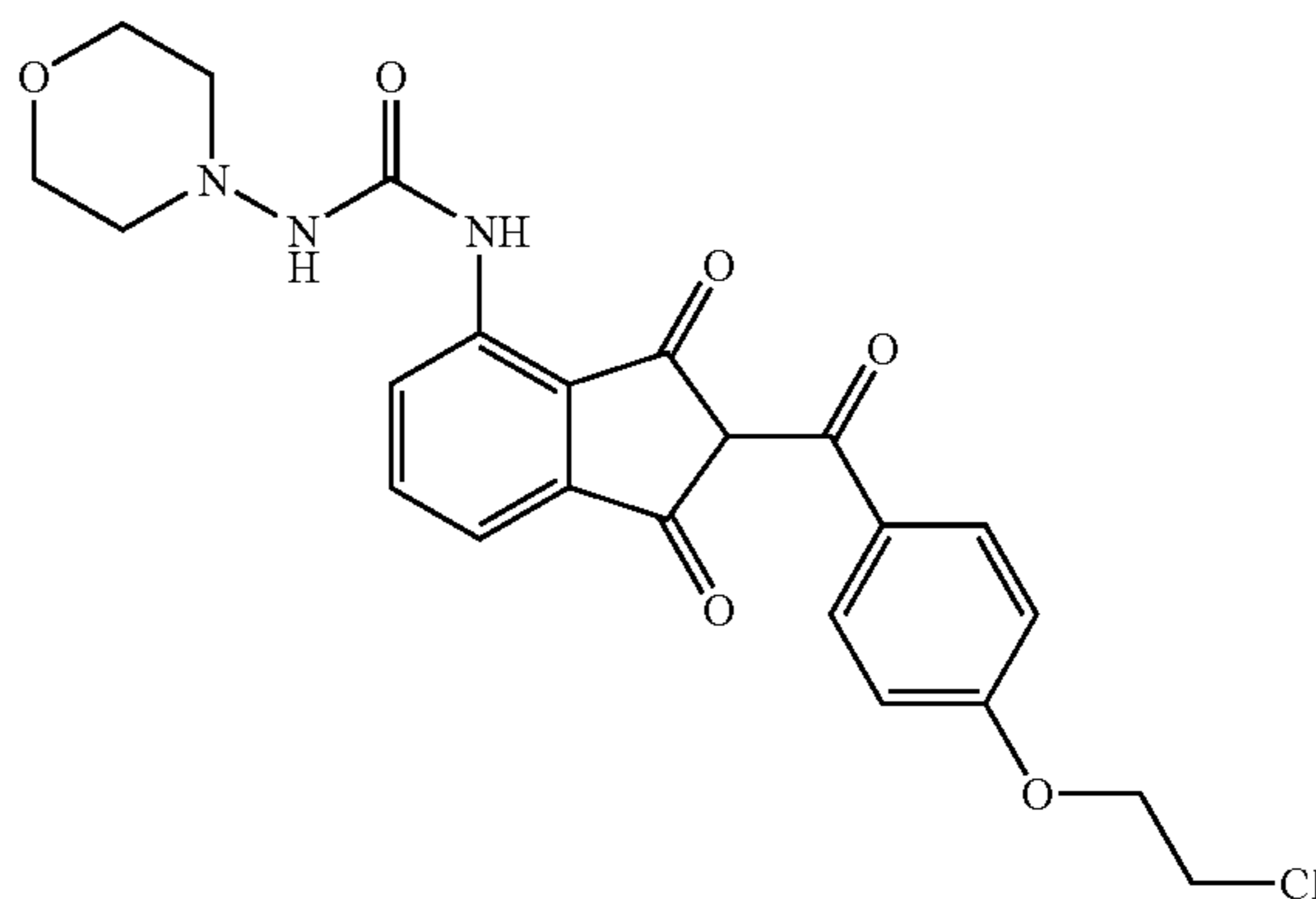
Synthesis of 1-{2-[4-(2-chloroethoxy)benzoyl]-1,3-dioxo-indan-4-yl}-3-morpholin-4-yl-urea
