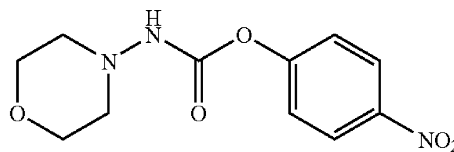
Synthesis of morpholin-4-ylcarbamic acid 4-nitrophenyl ester
