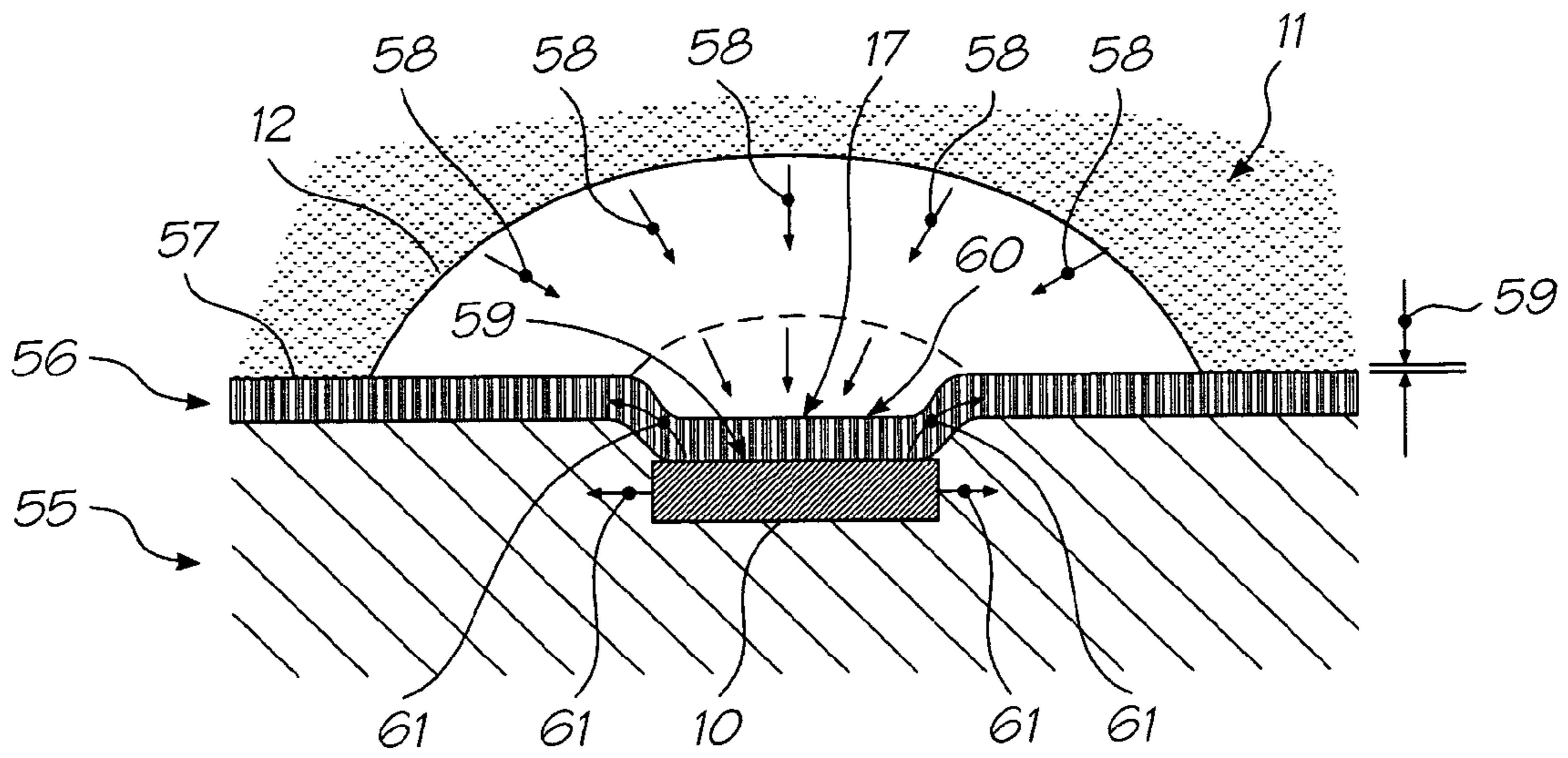
FIG. 47 (PRIOR ART)
