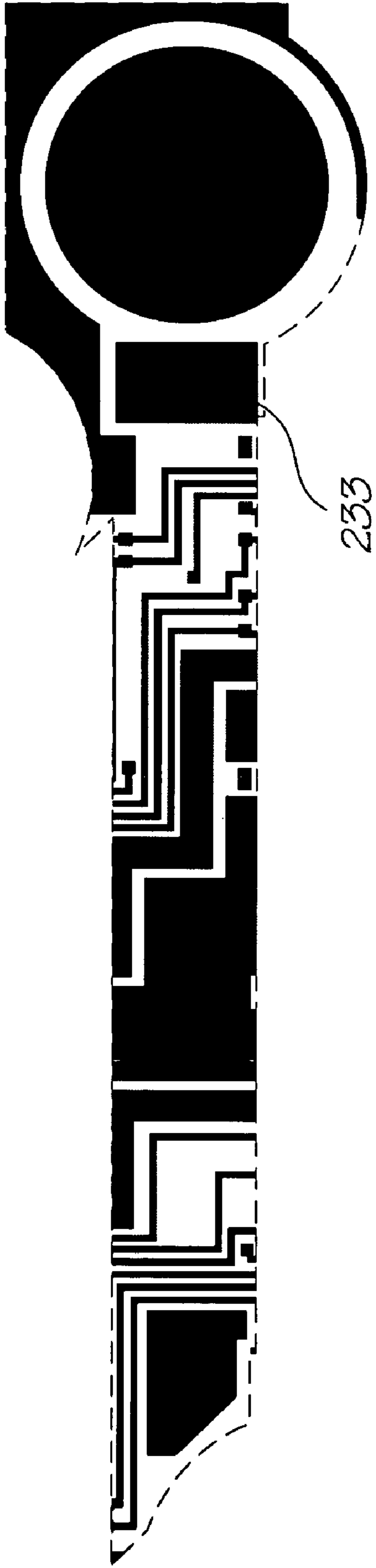
Metal 2 mask
