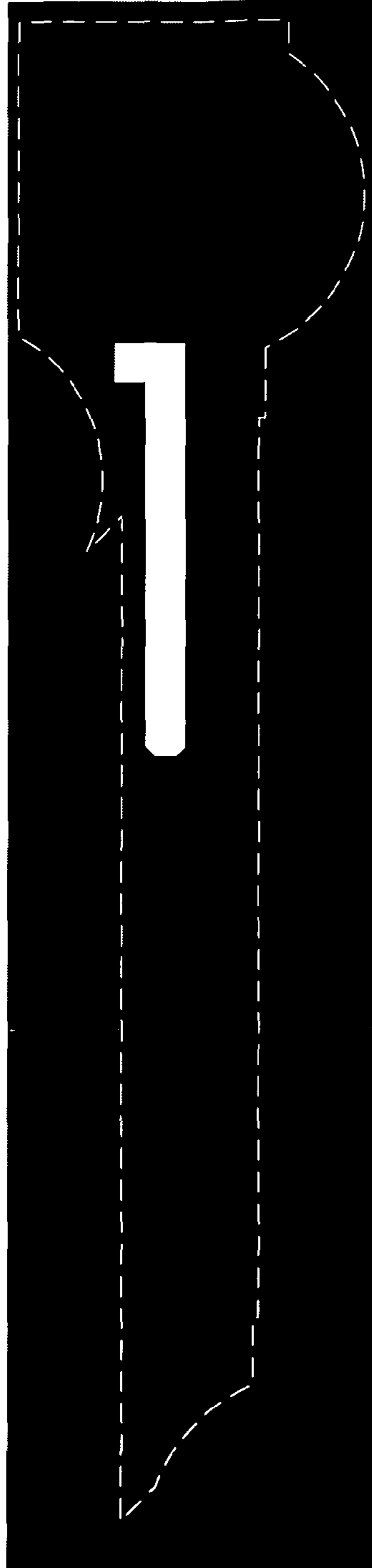
N-Well mask
