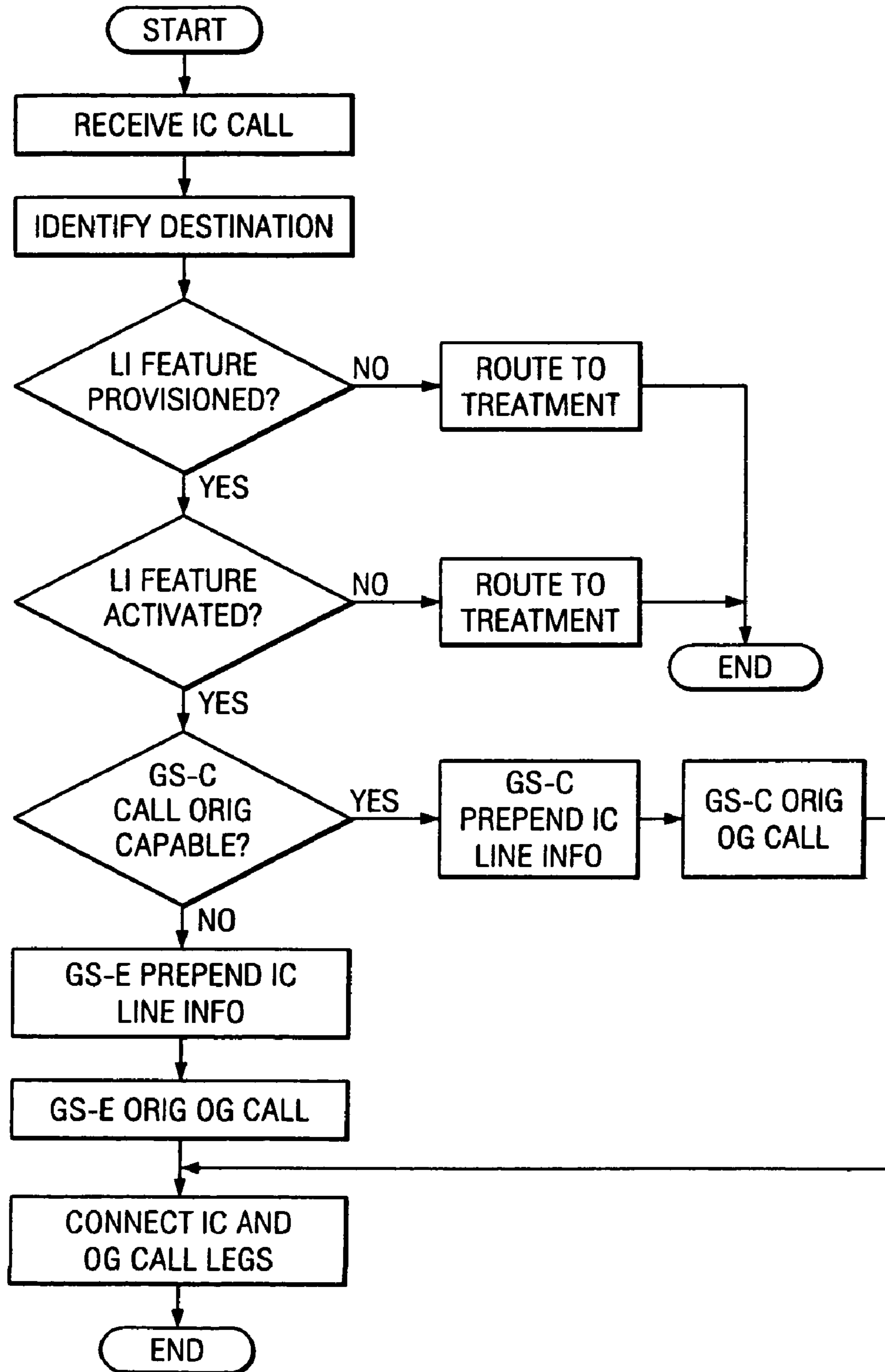
INCOMING CALL HANDLING FLOW CHART
