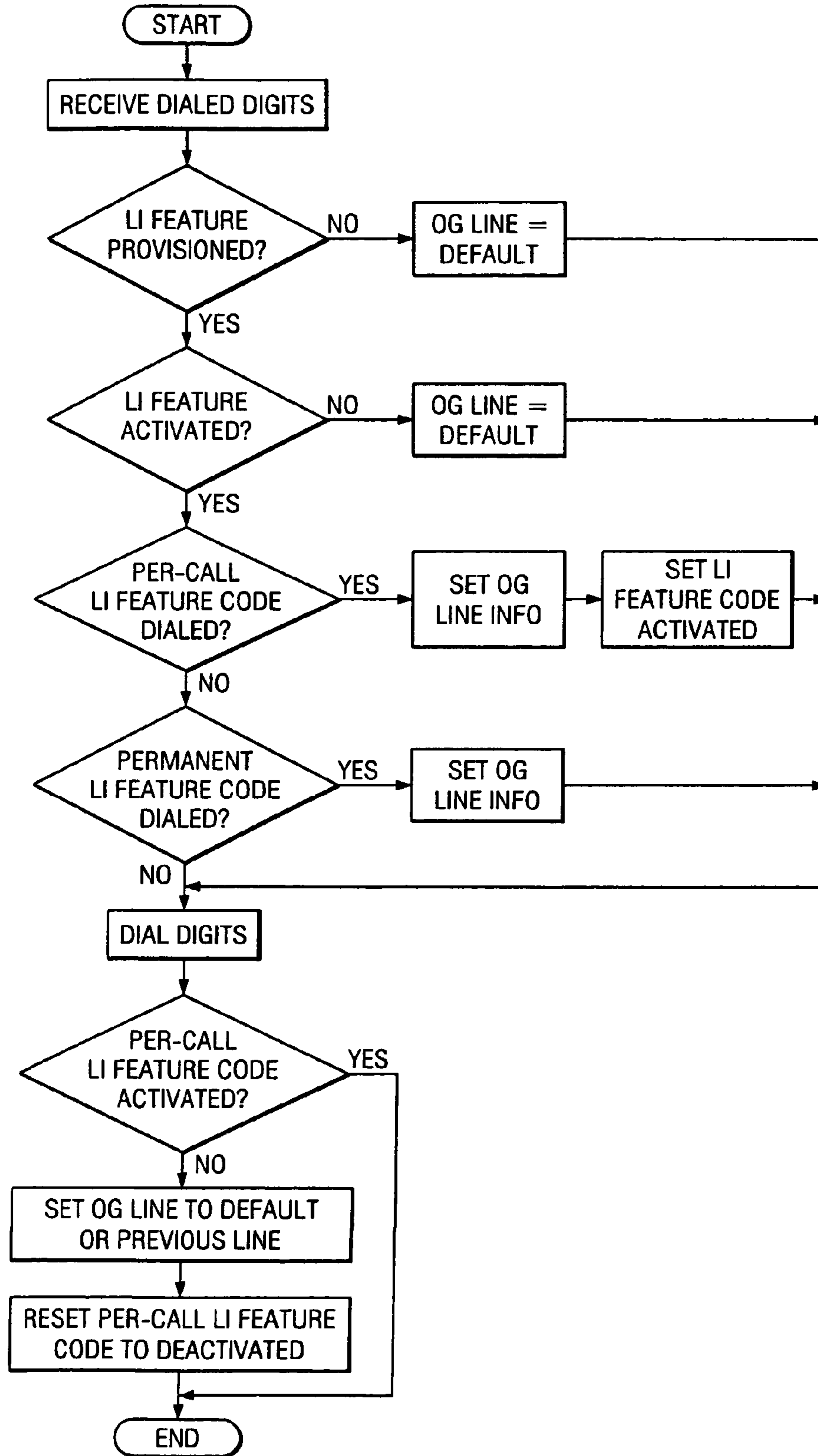
FIG. 18 OUTGOING CALL HANDLING FLOW CHART
