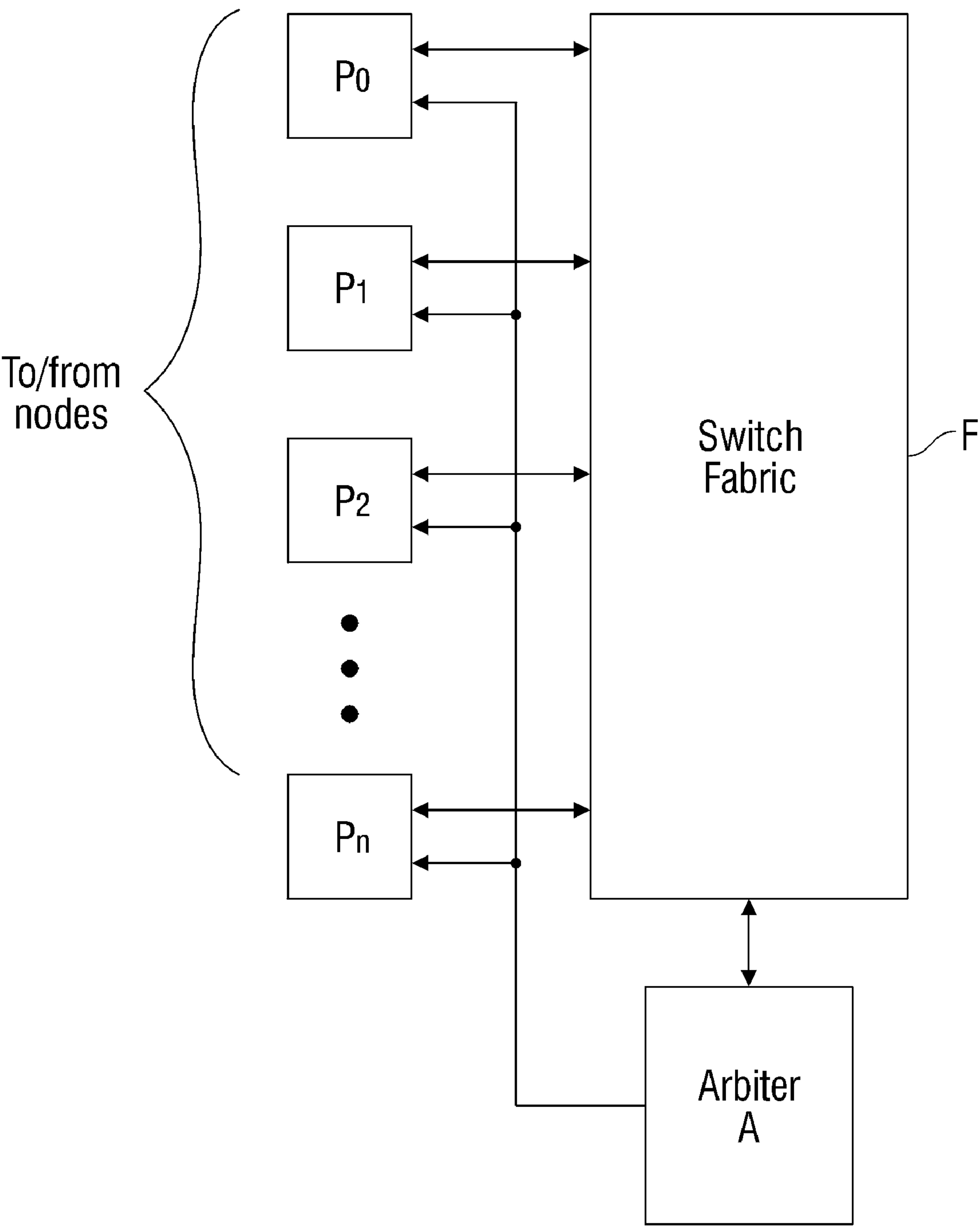
FIG. 1 (Prior Art)
