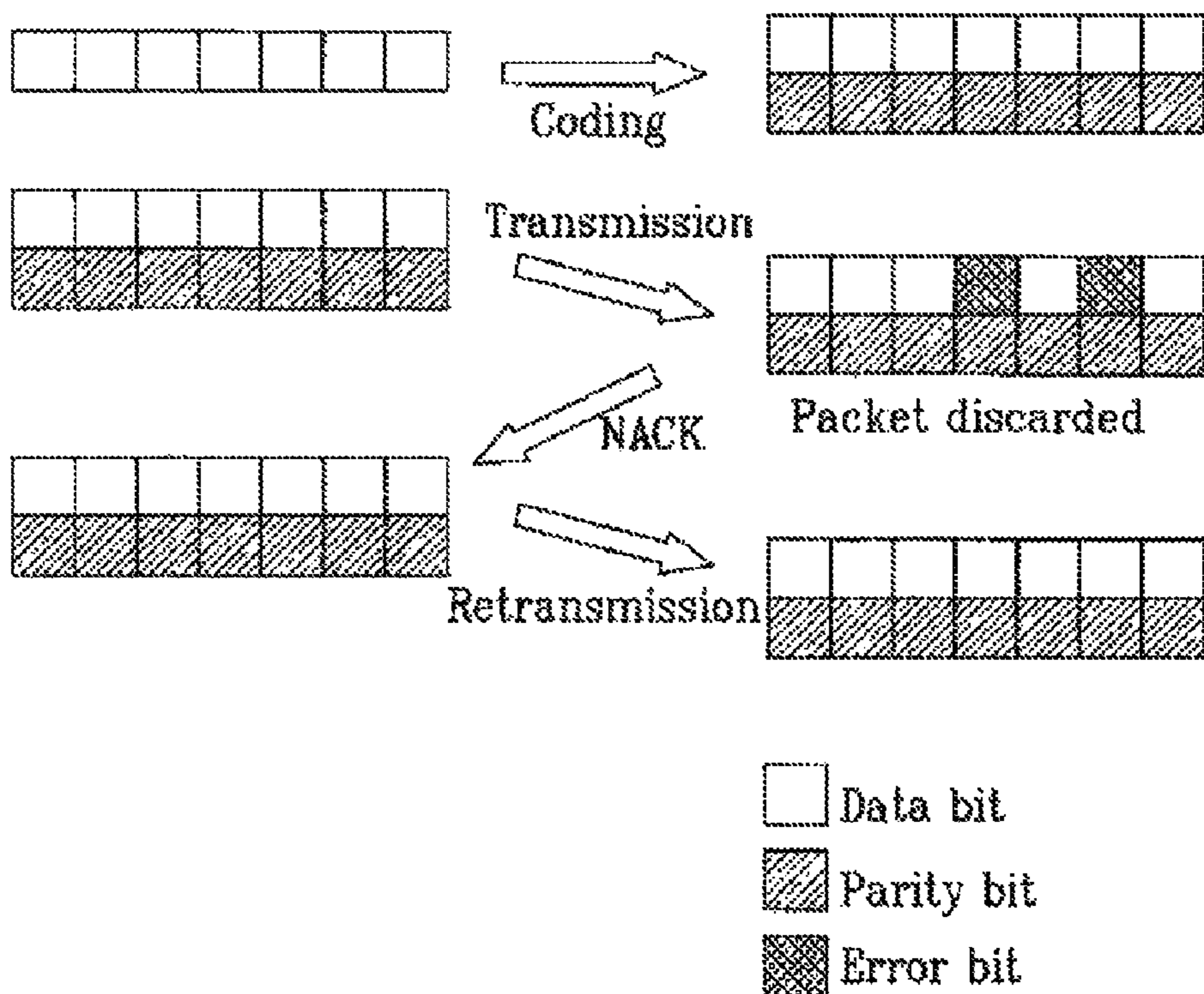
FIG. 2 Prior Art
