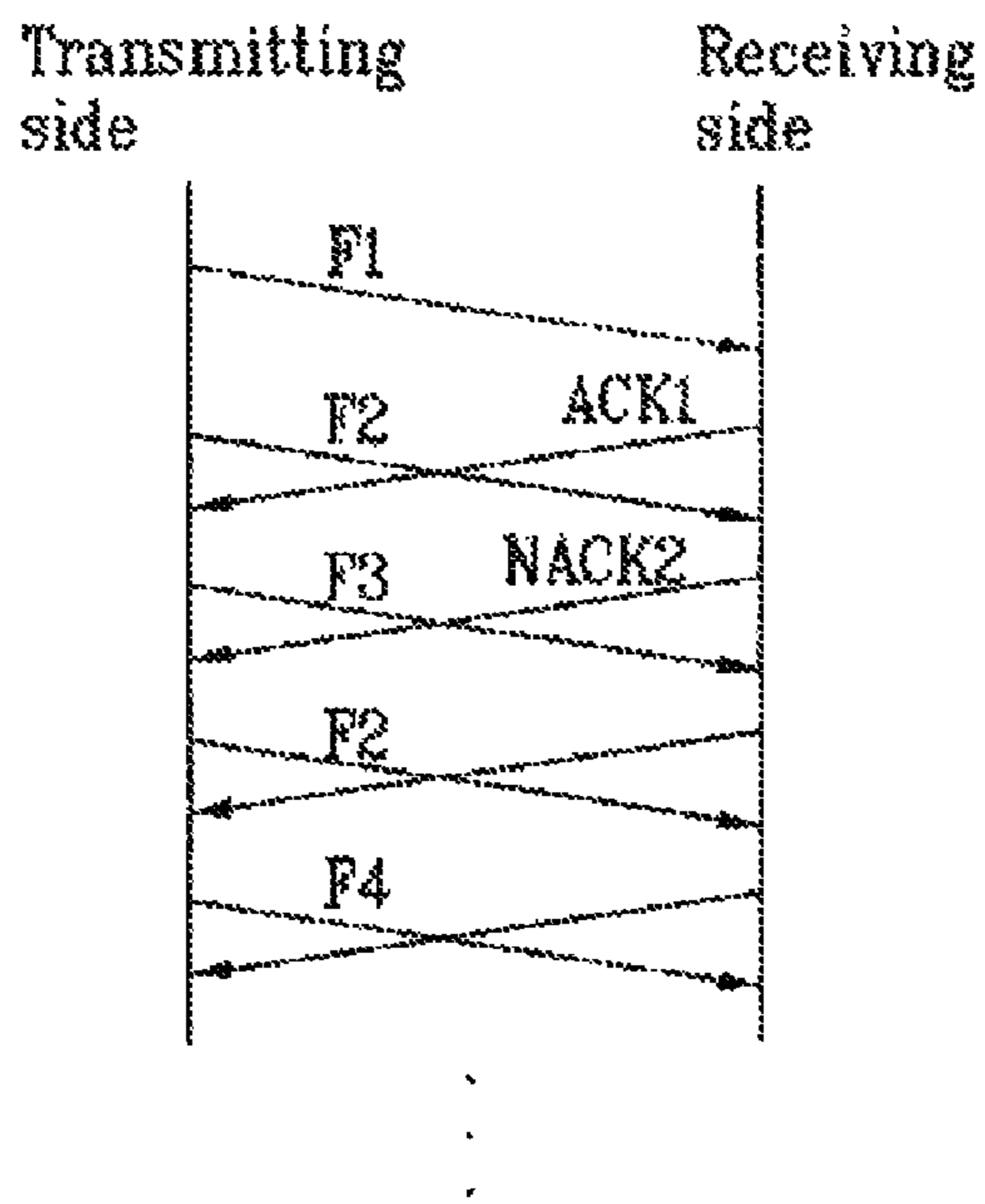
FIG. 2 Prior Art
