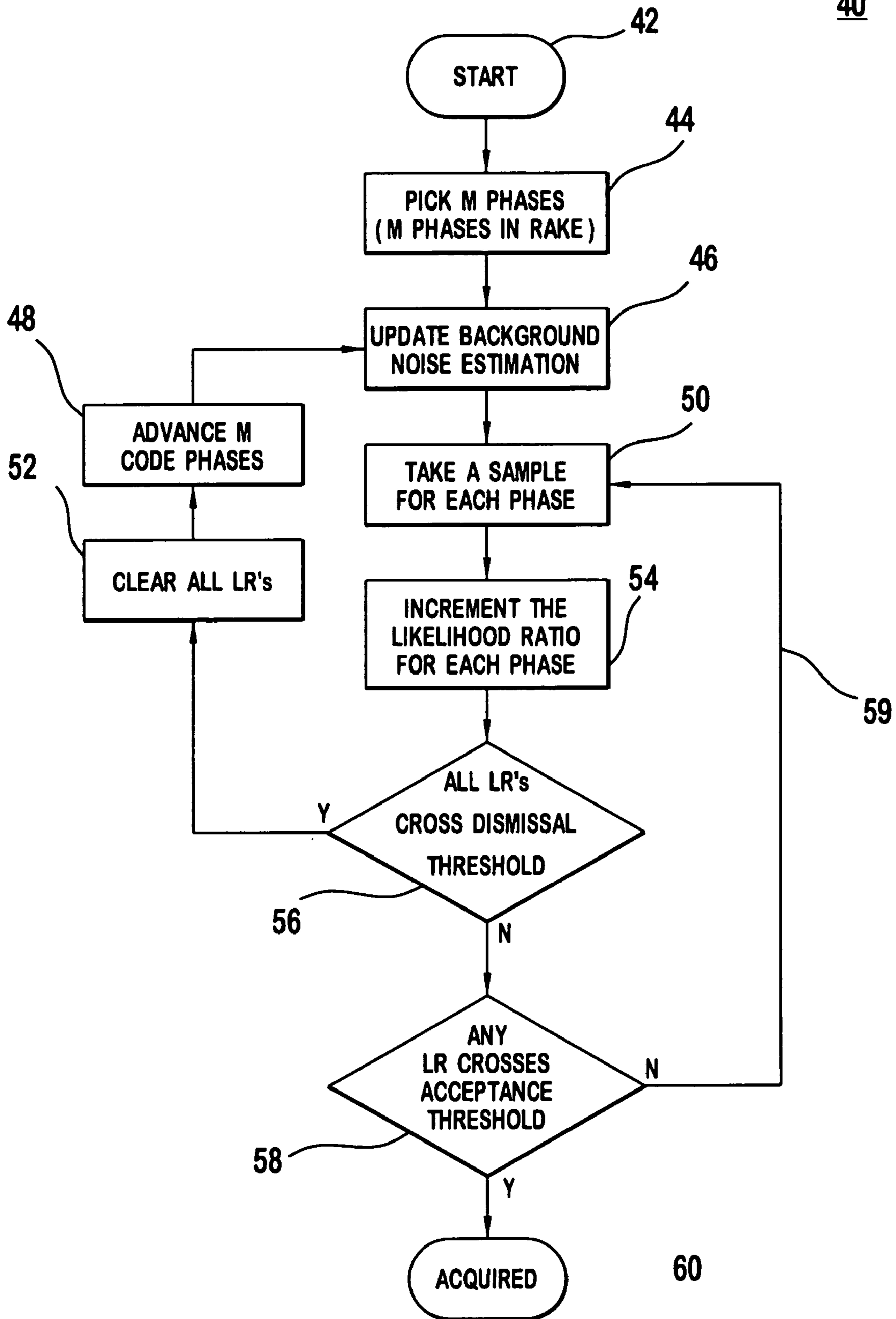
FIG. 2 (PRIOR ART)
