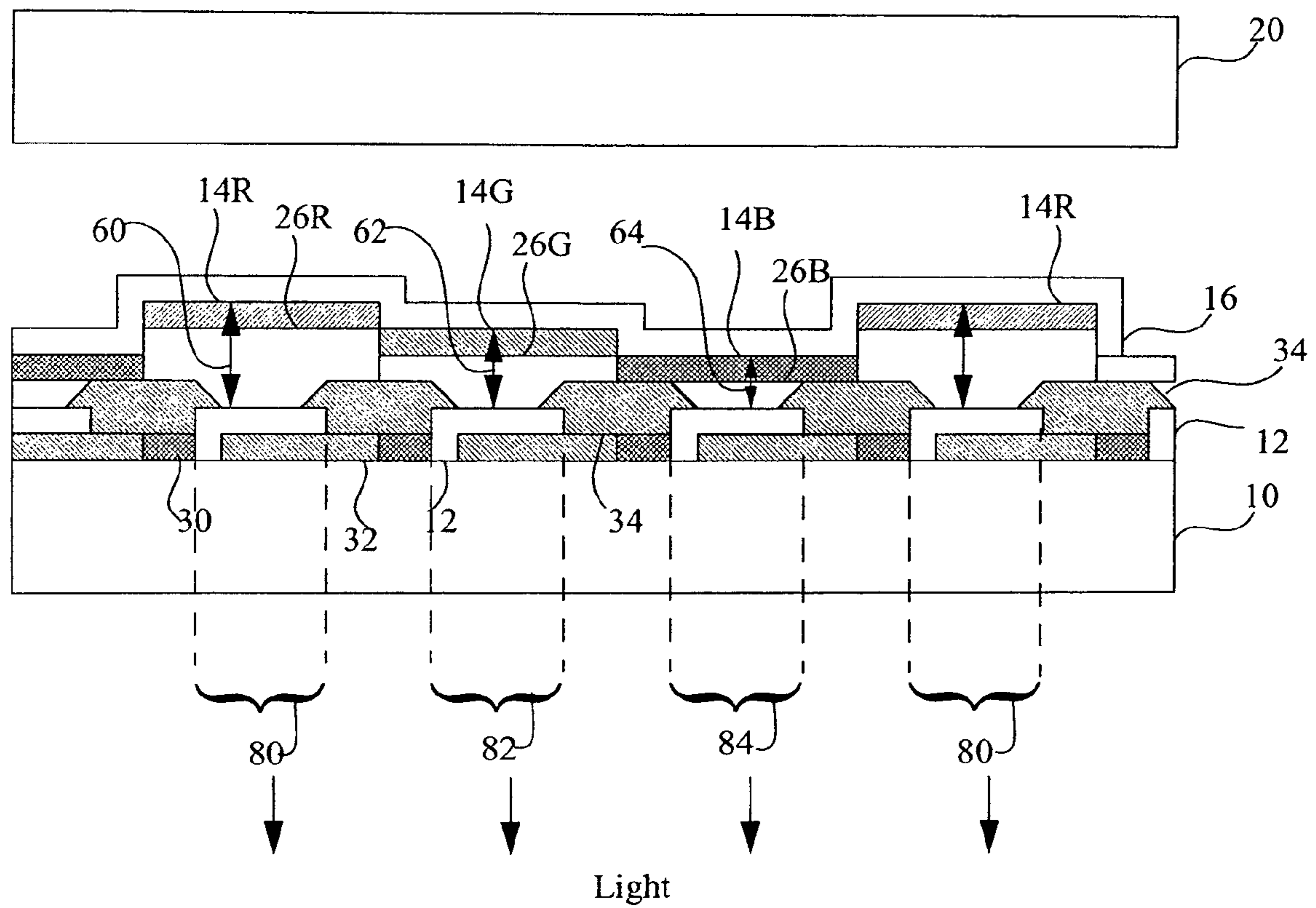
Fig. 7 - Prior Art
