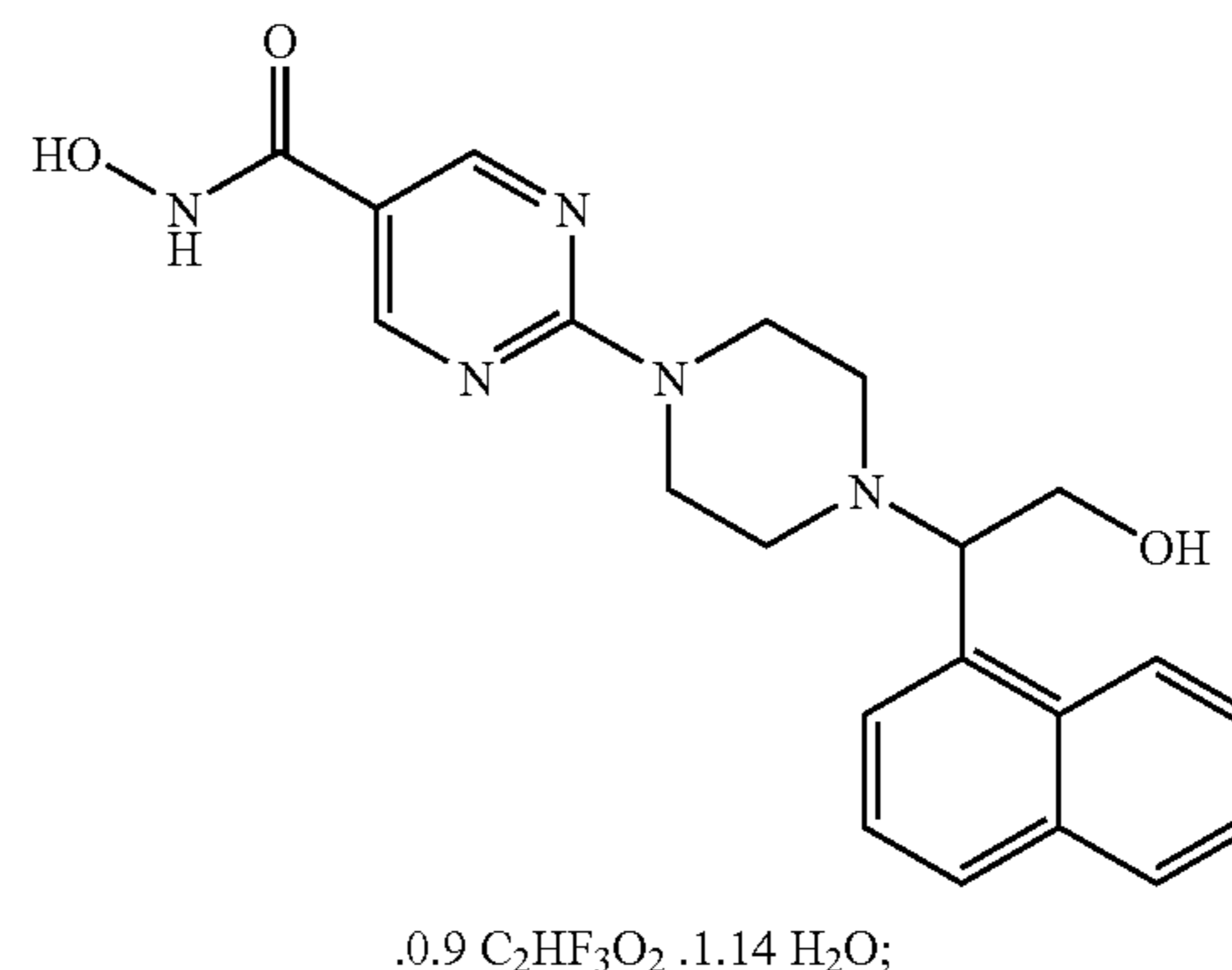
Compound No. 1
