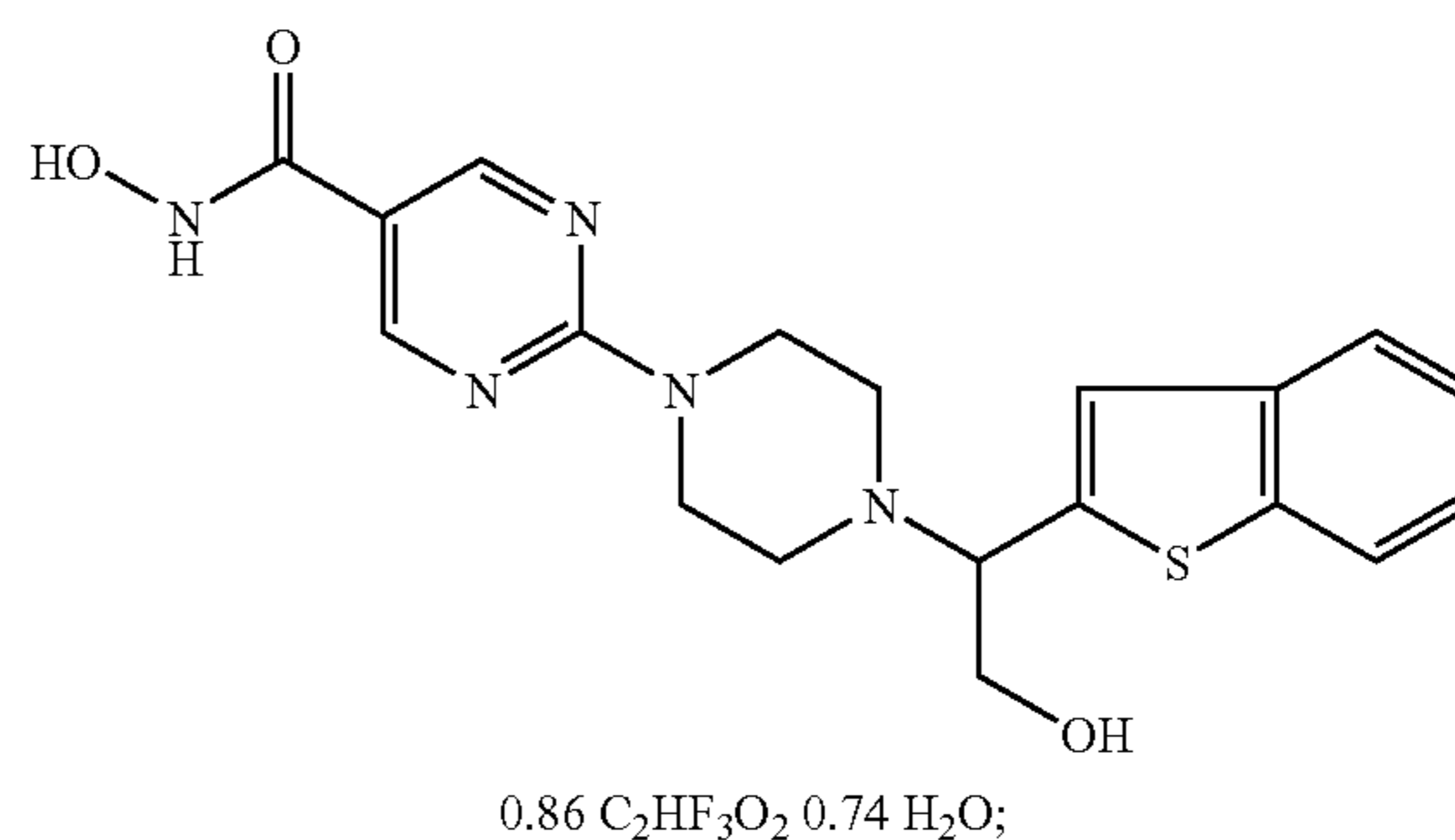
Compound No. 2
