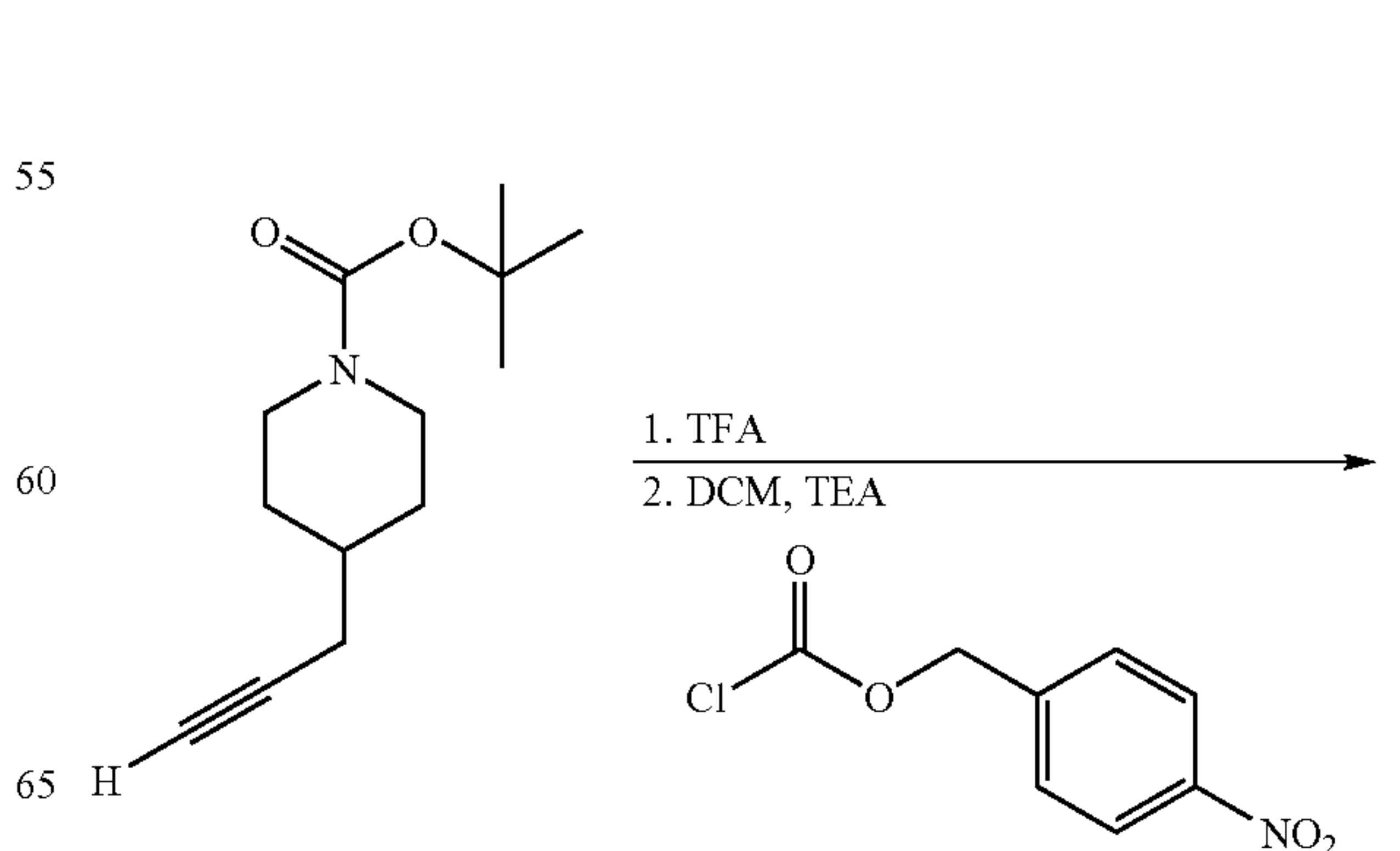
Intermediate 11
