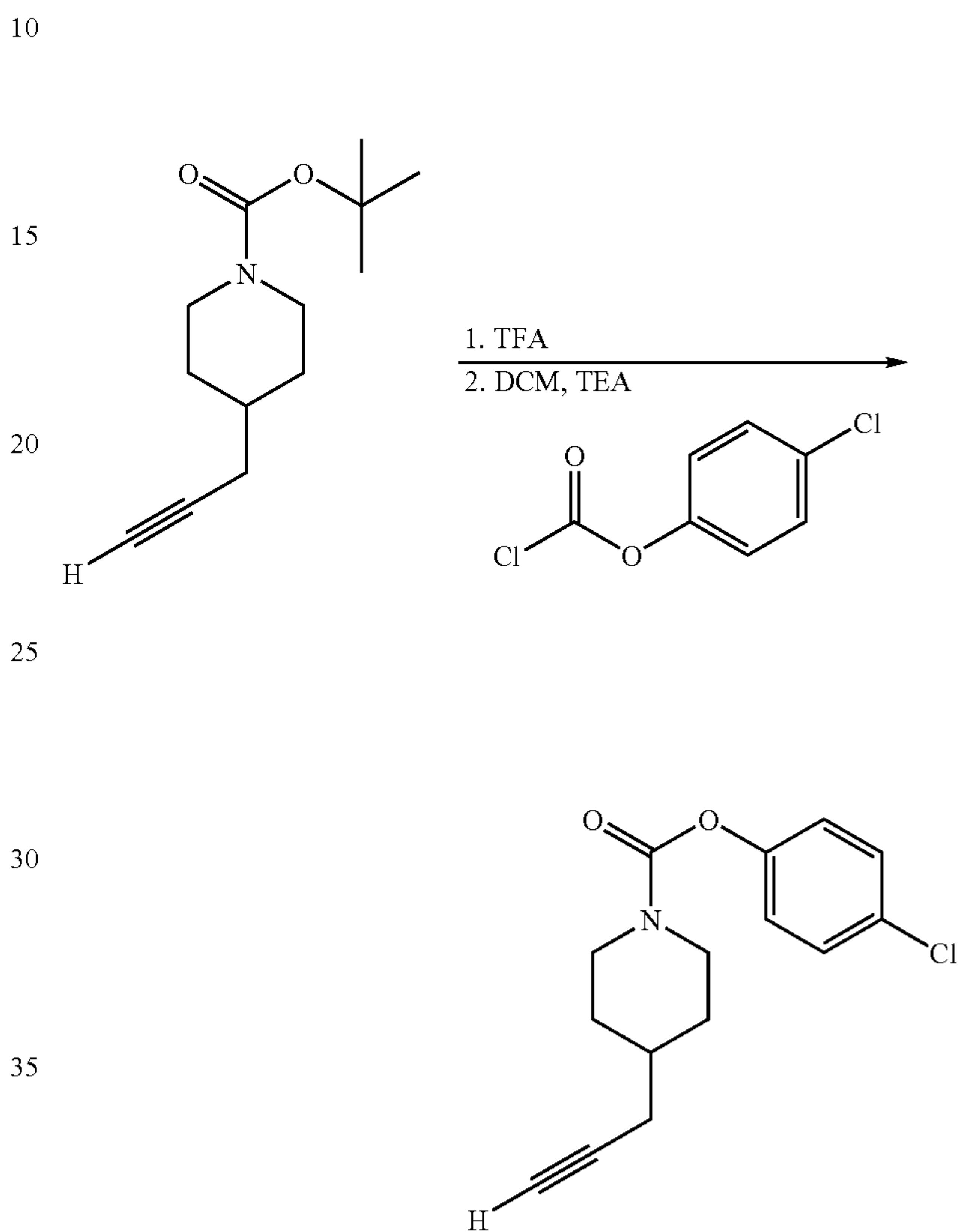
Intermediate 10
