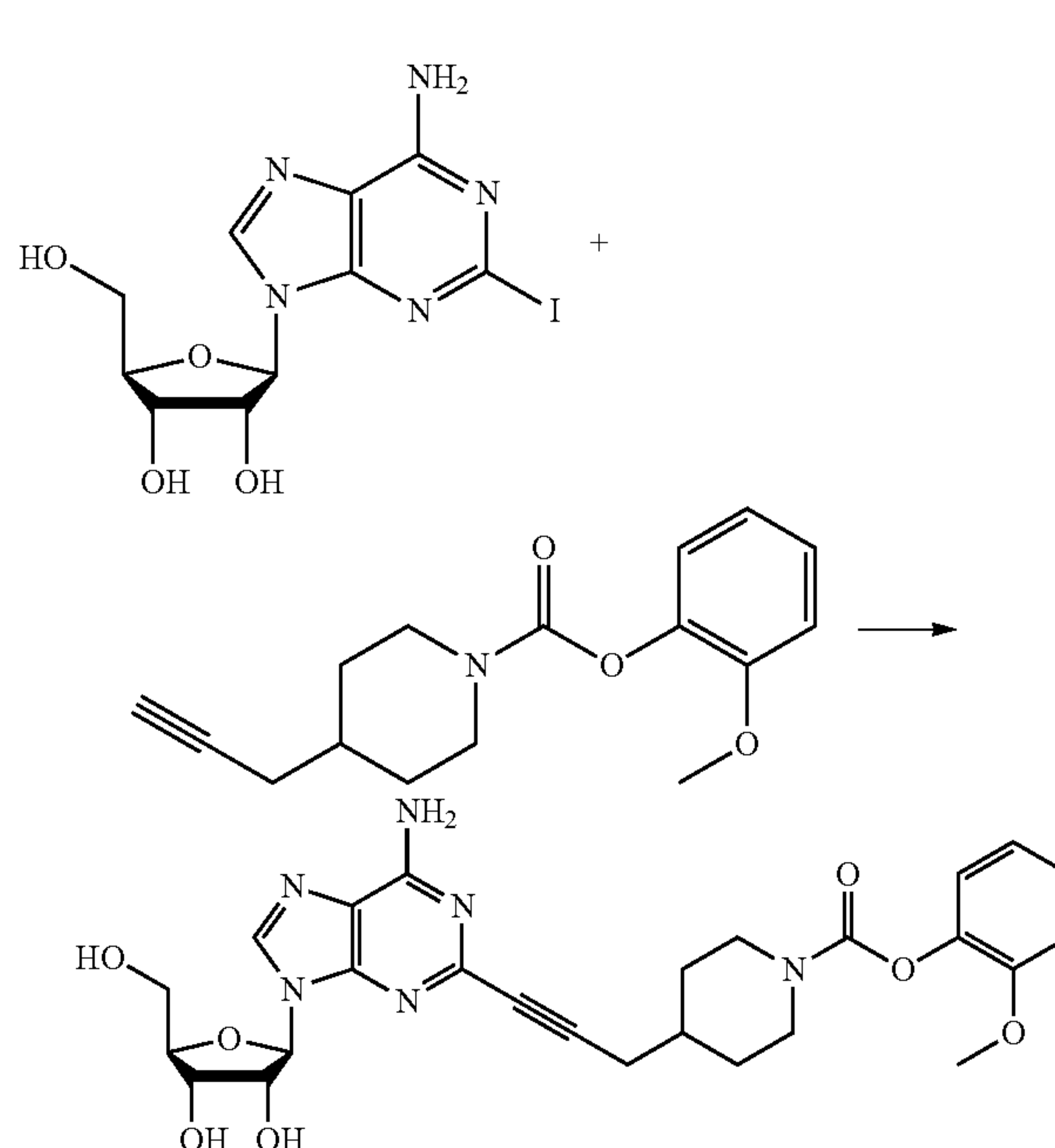
Compound 36
