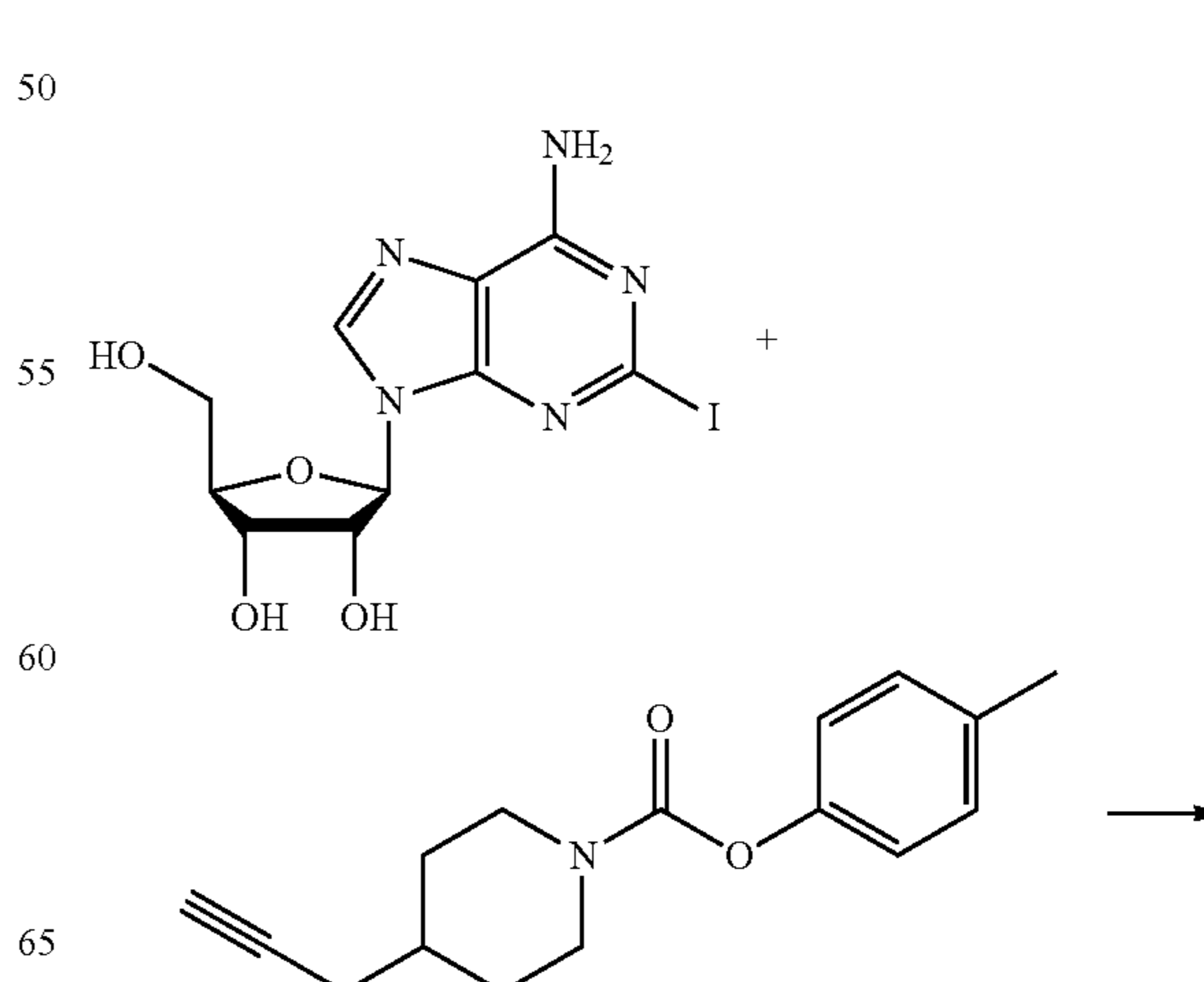
Compound 29
