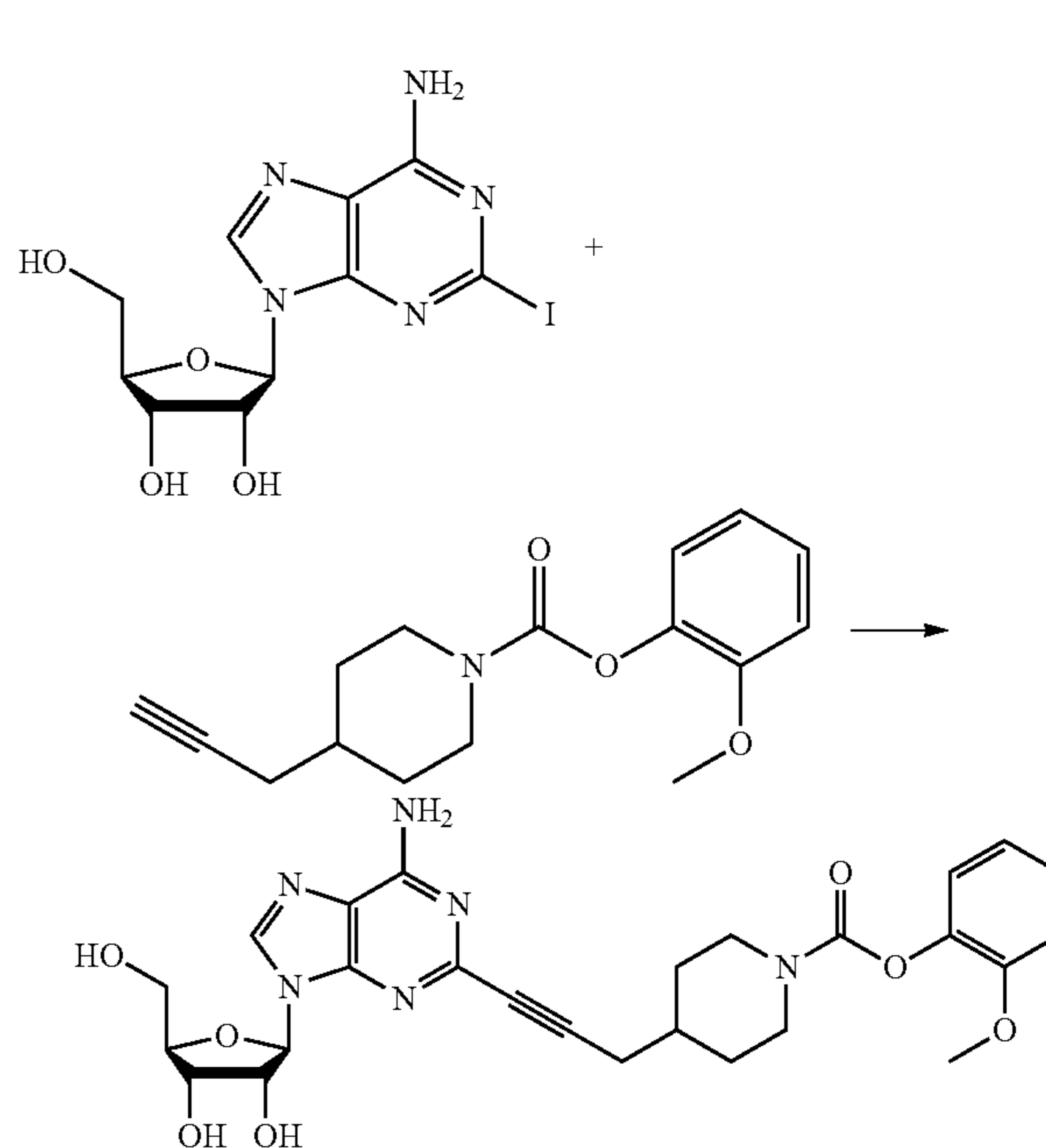
Compound 36
