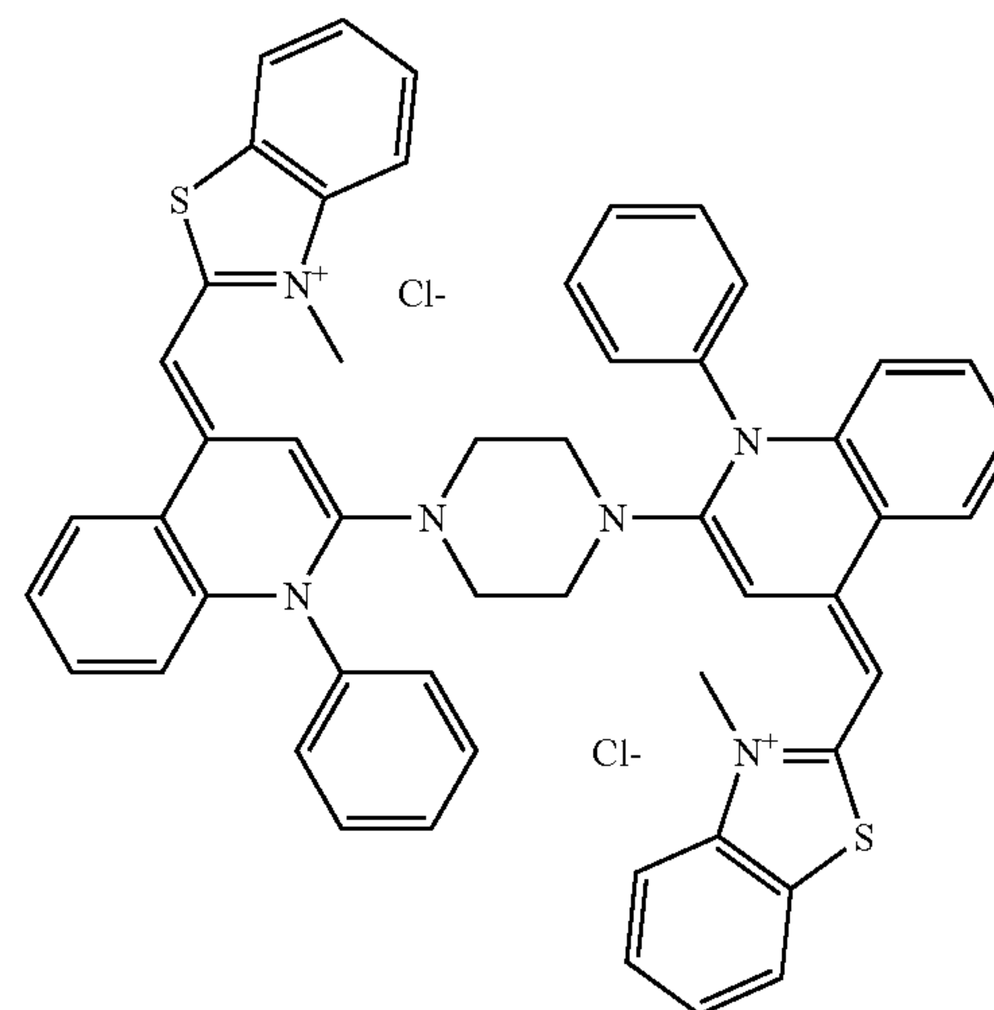
Compound 6
