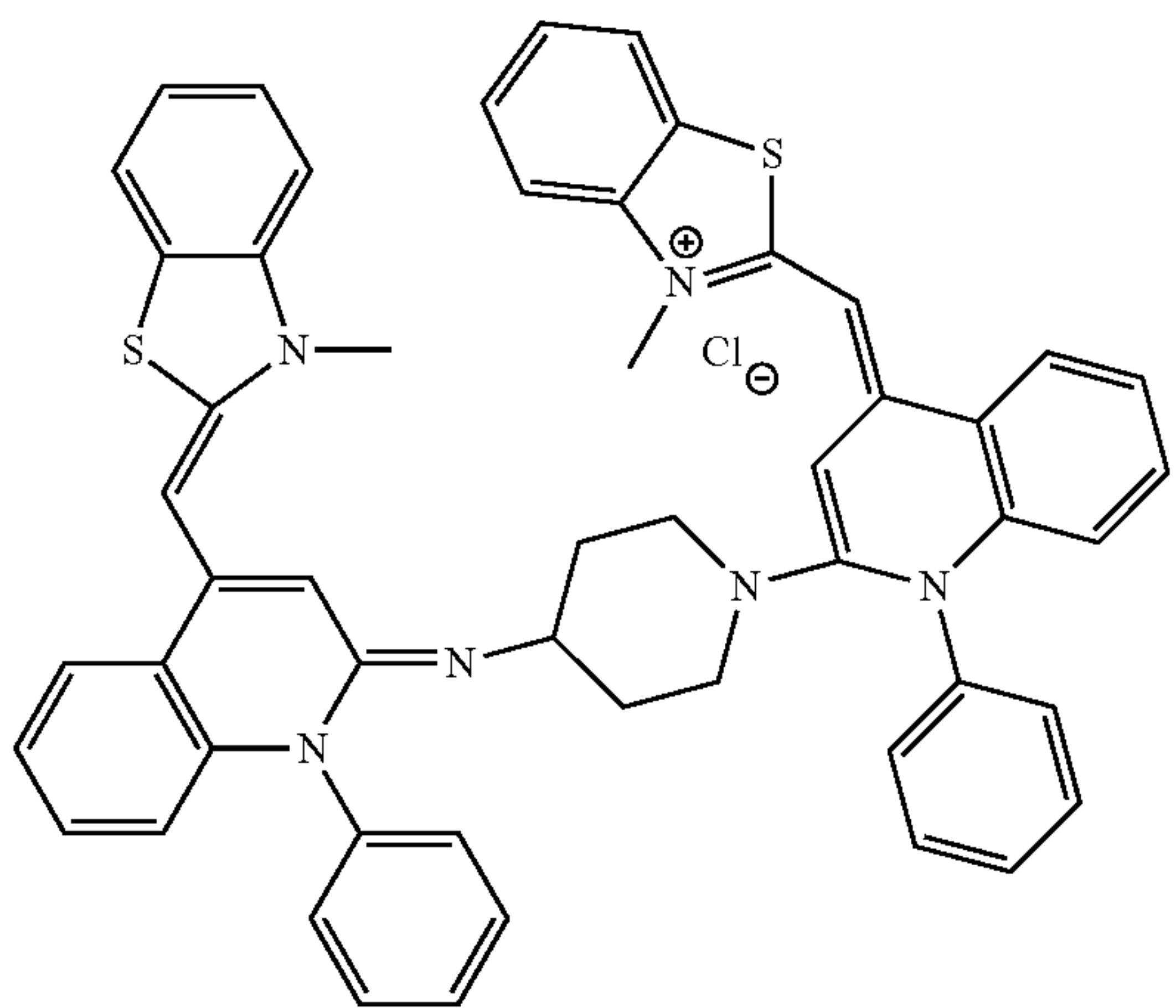
(Compound 30)
