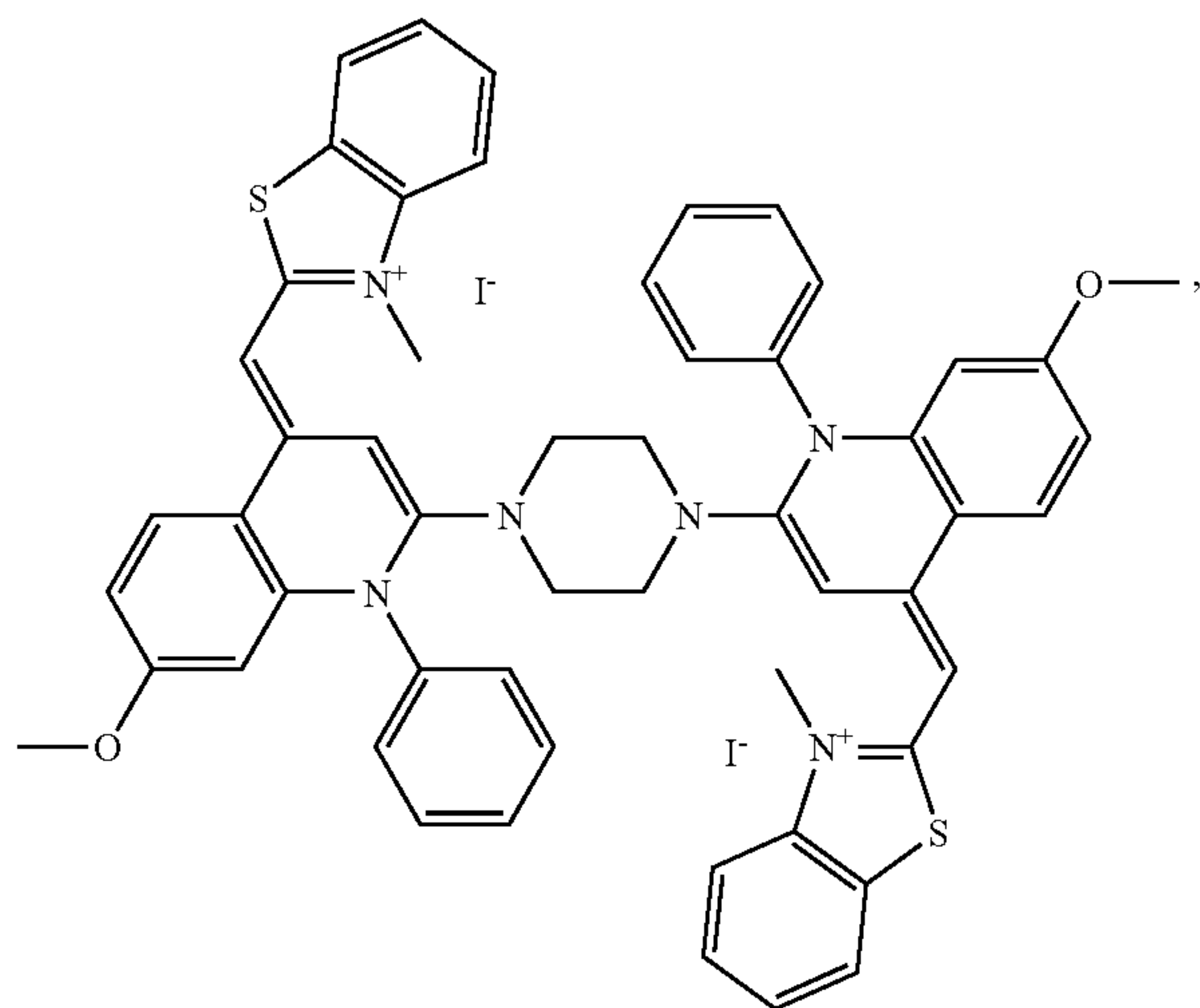
(Compound 19)
