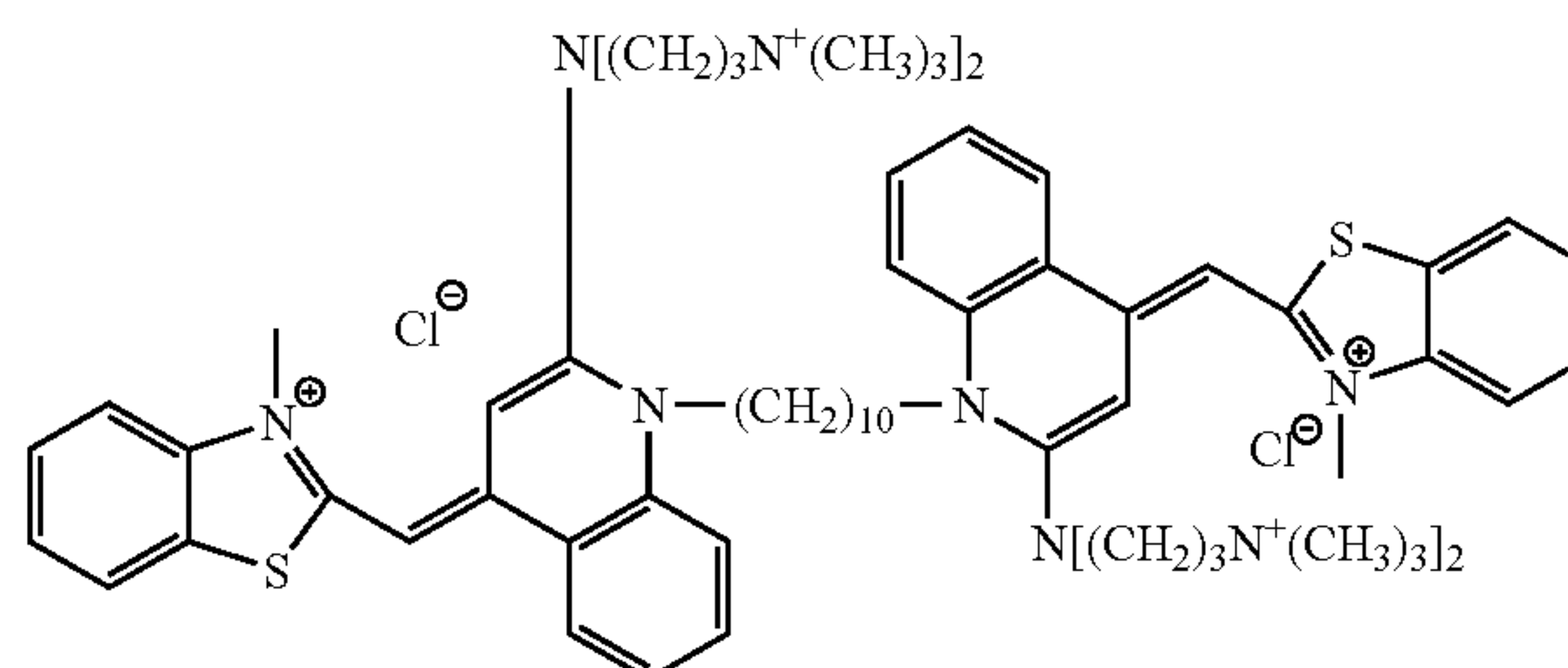
Compound 13
