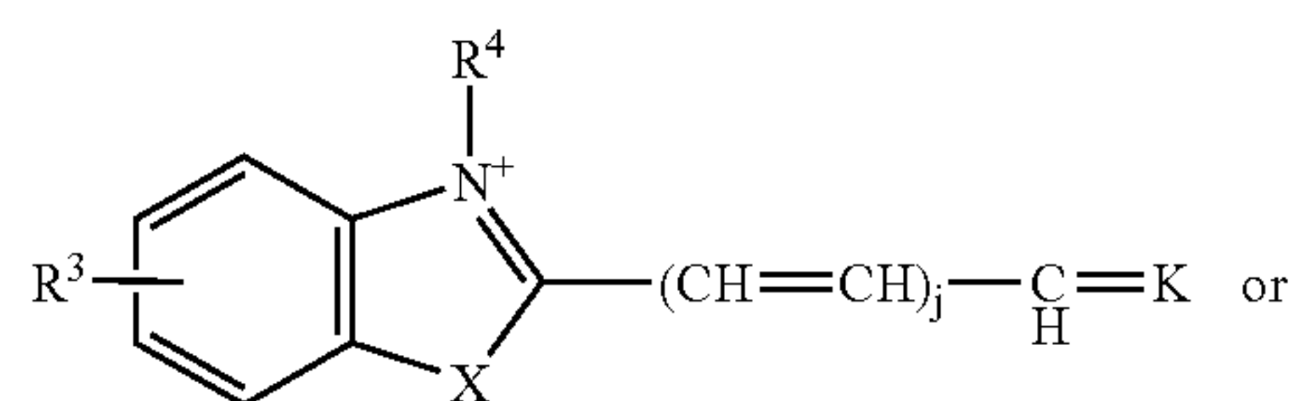
Formula (III)(y)
