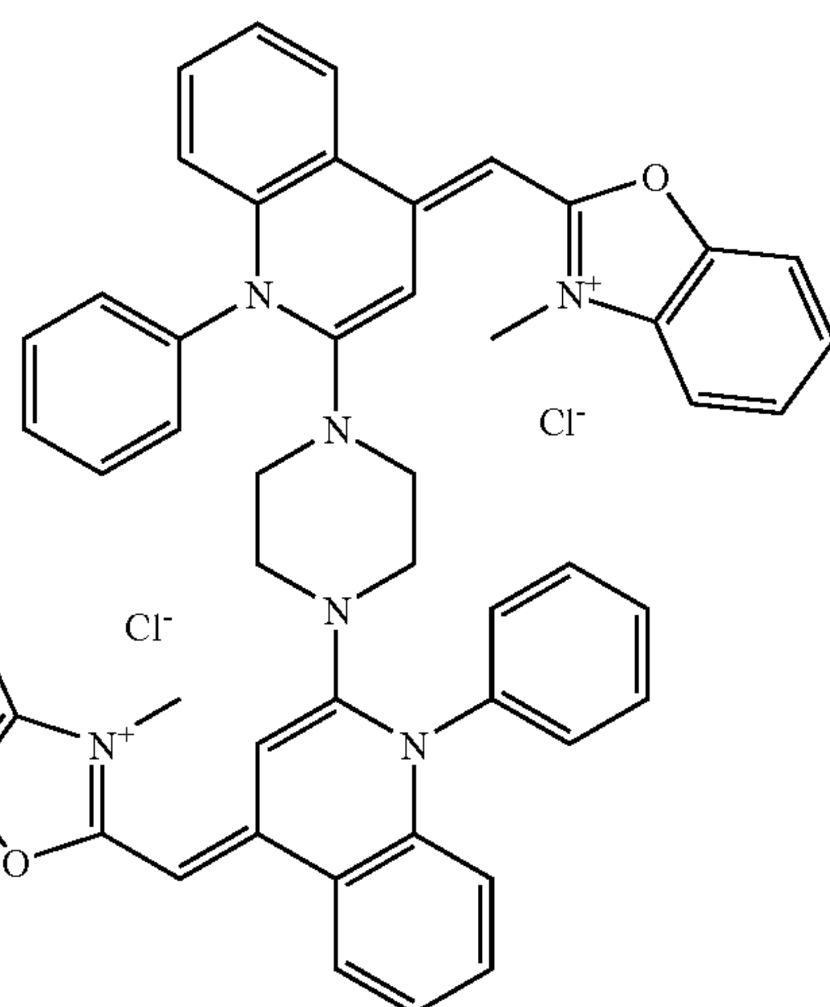
Compound 20
