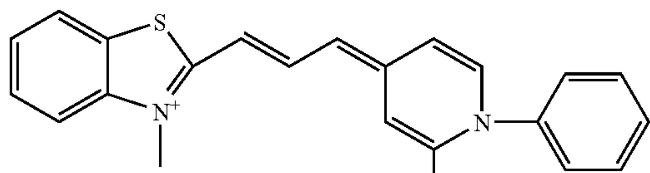
Compound 18
