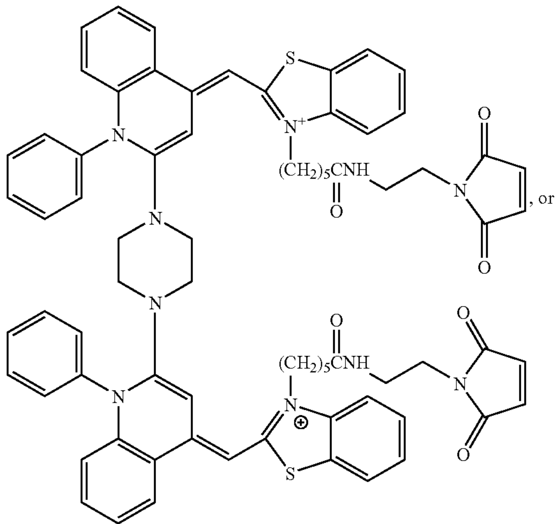
(Compound 33)
