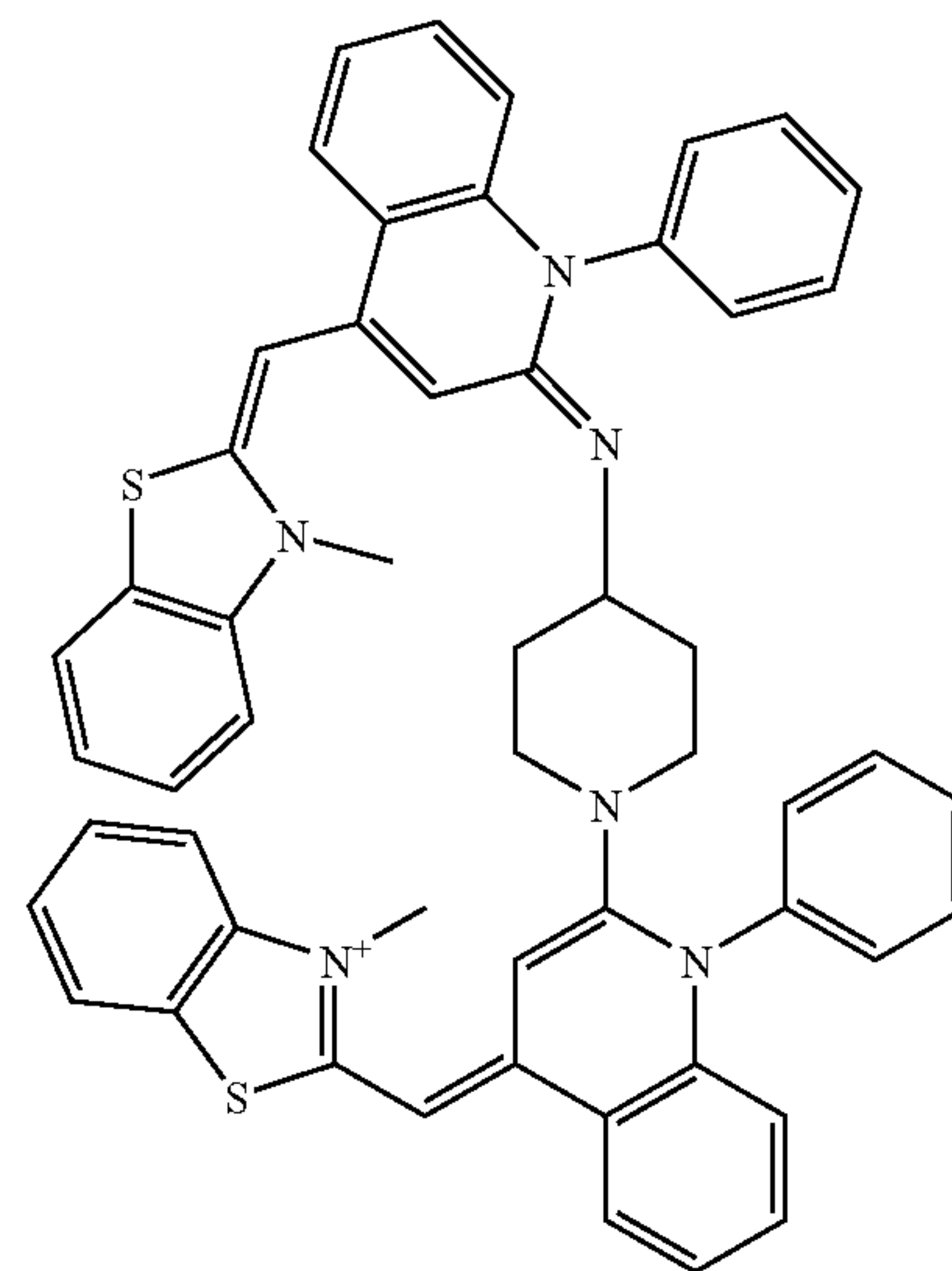
Example 22
