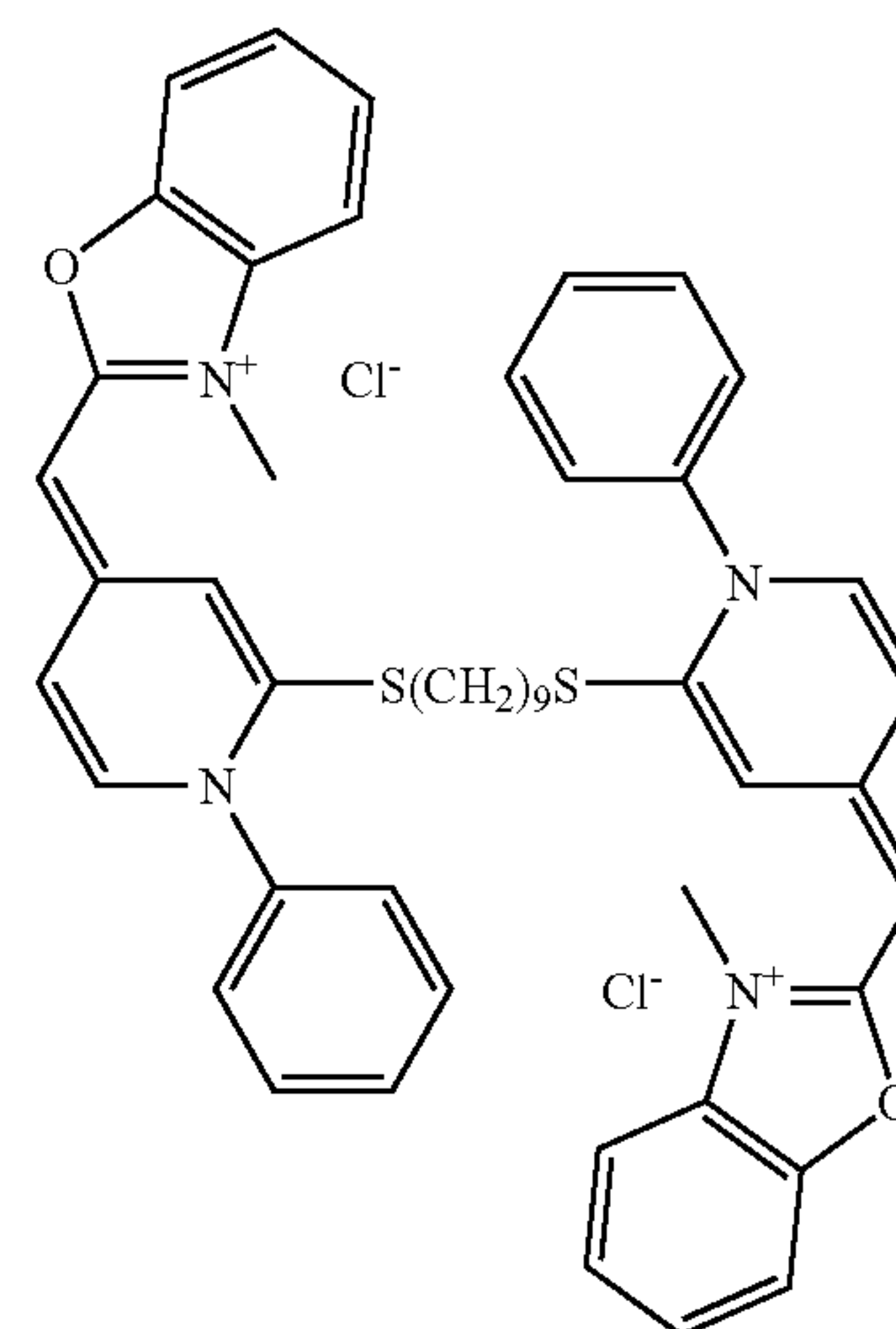
Example 23
