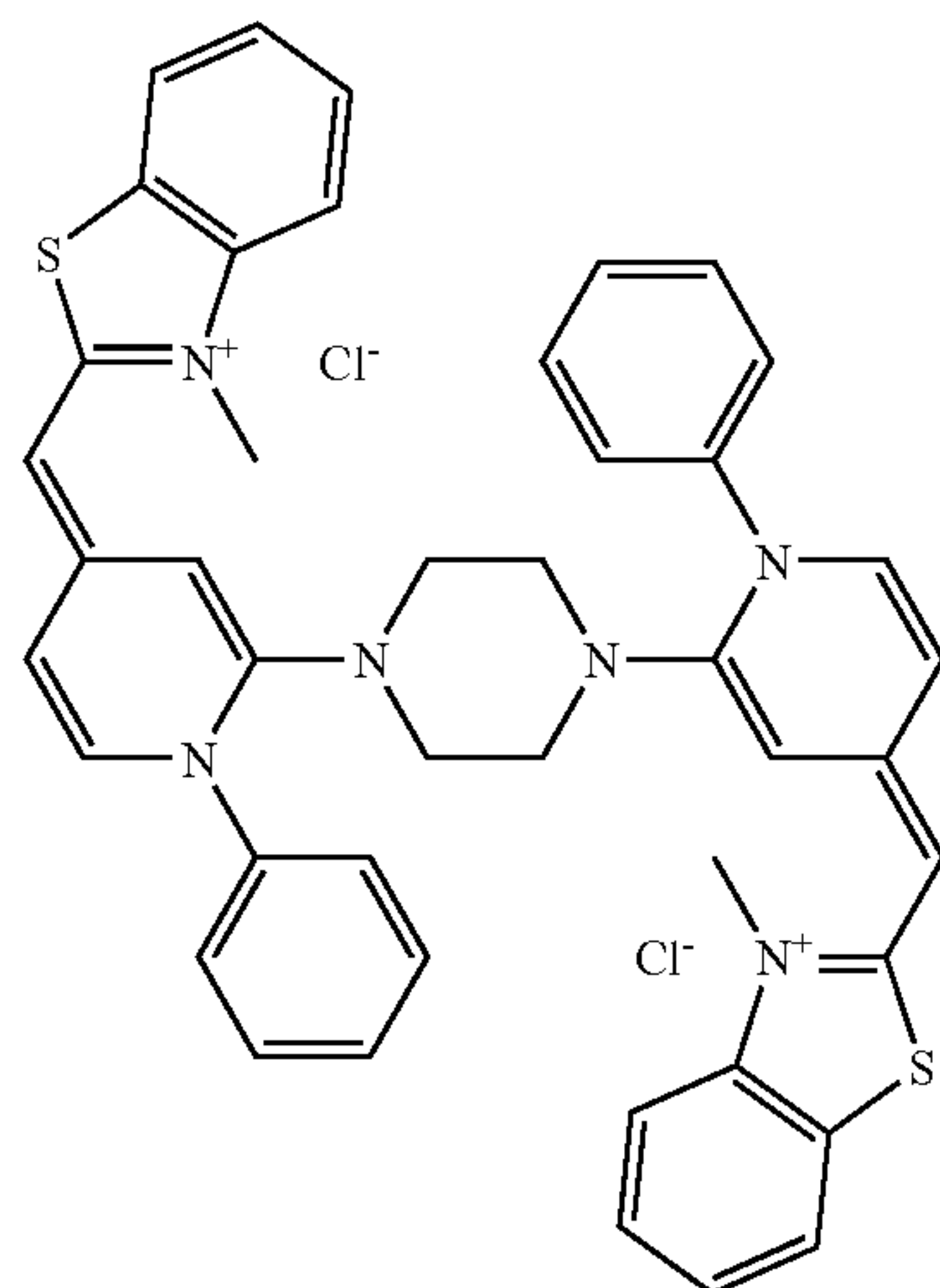
Example 24
