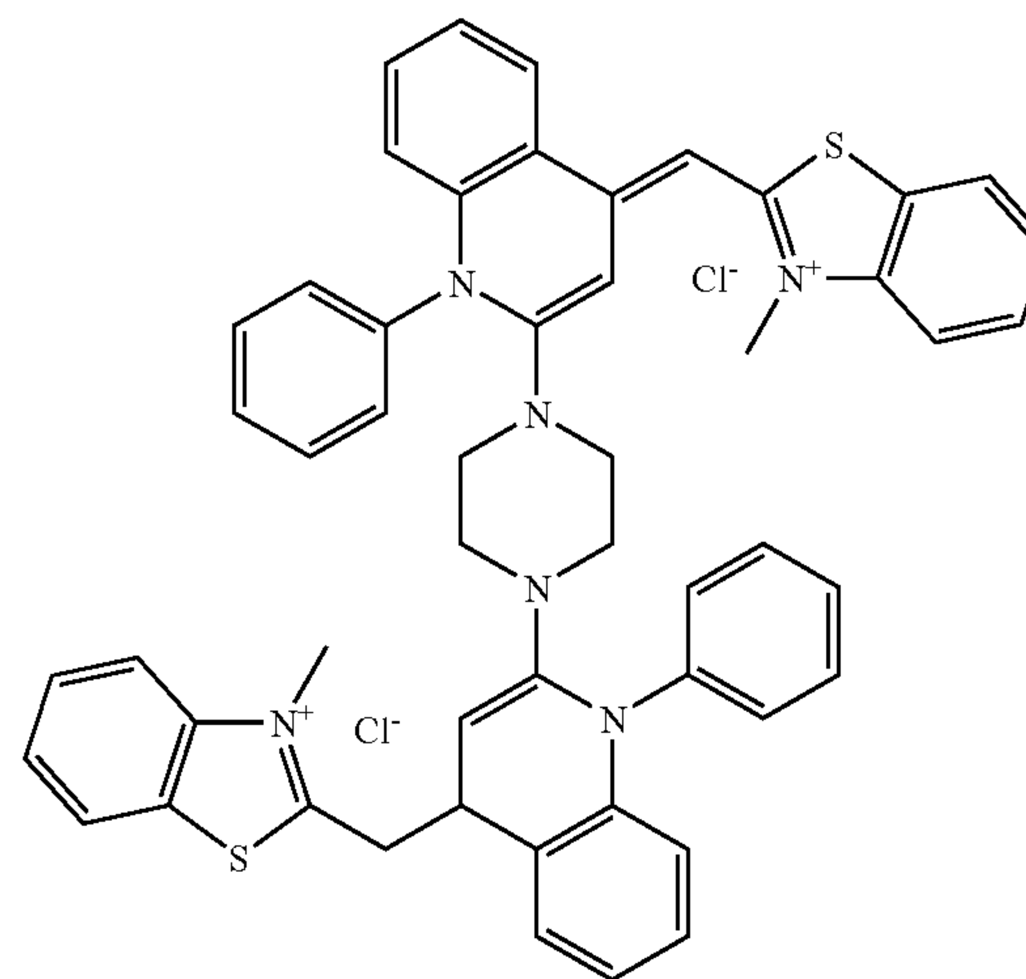
Compound 6
