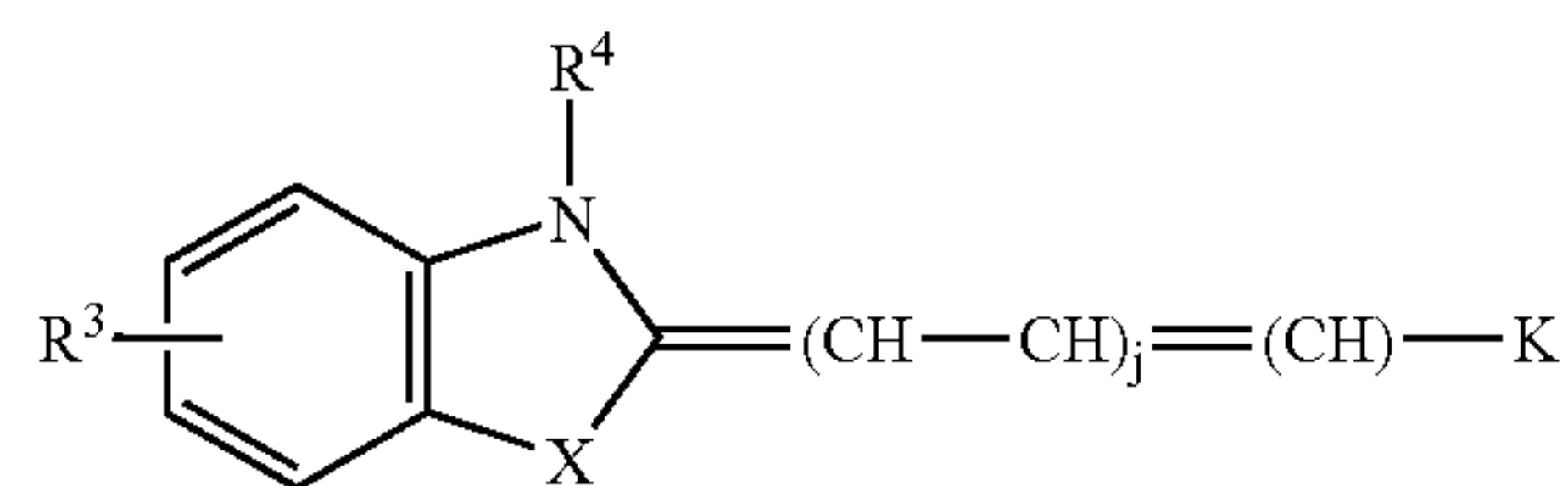
Formula (III)(y)
