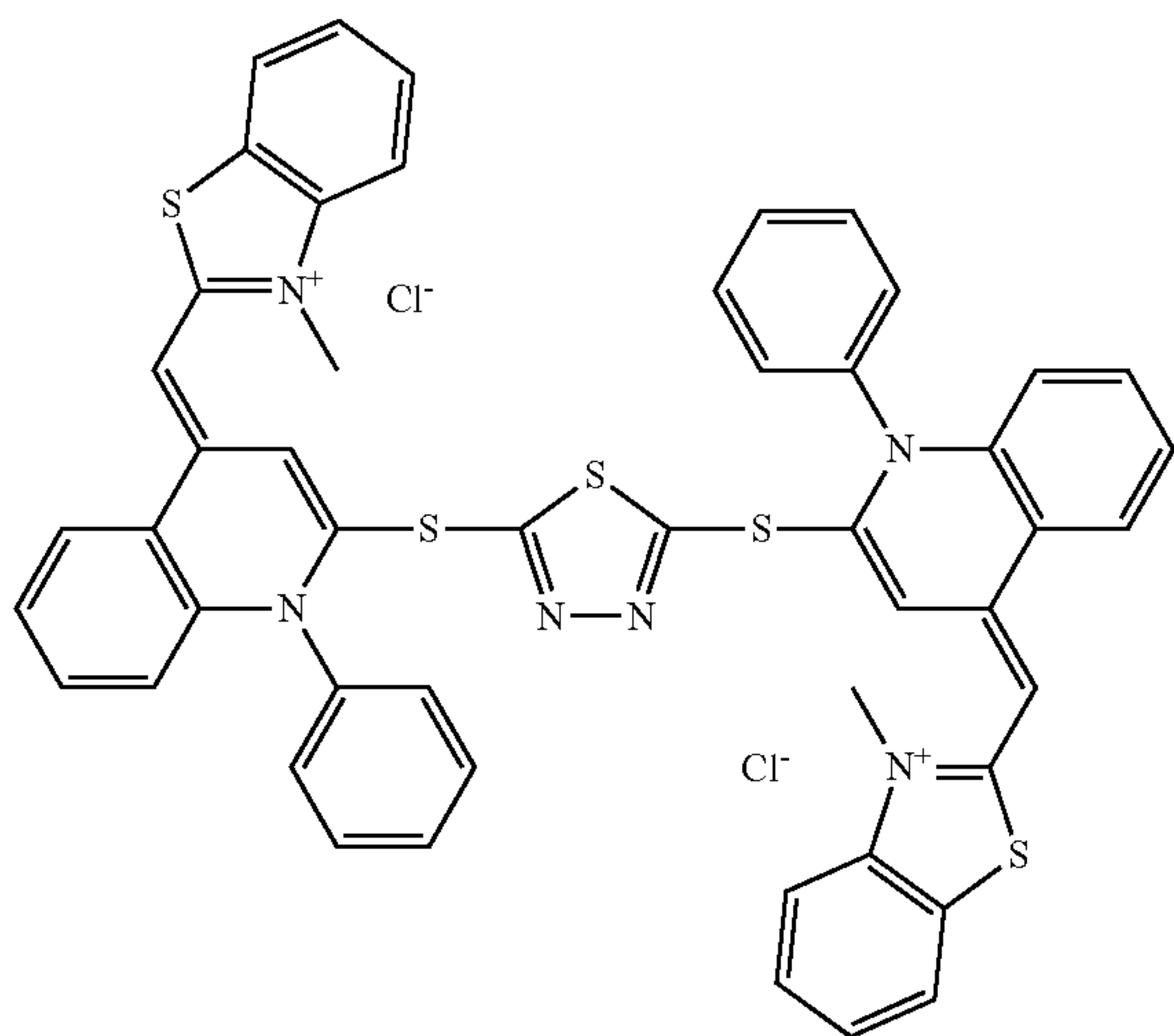
Compound 7
