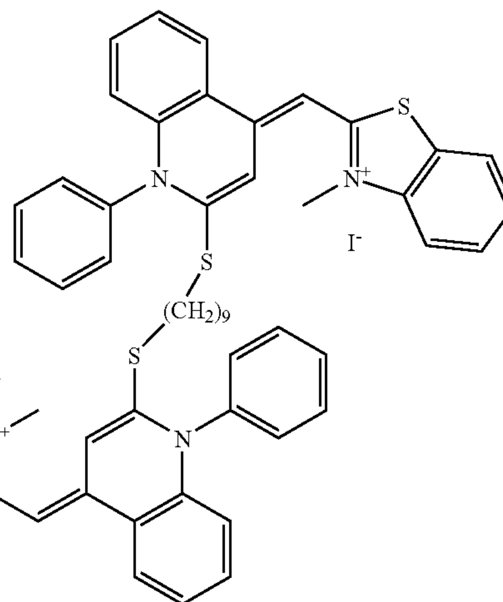
(Compound 28)
