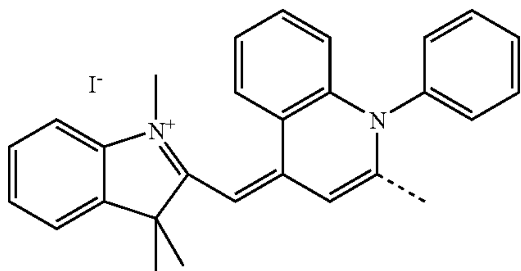
Formula (III)(h)
