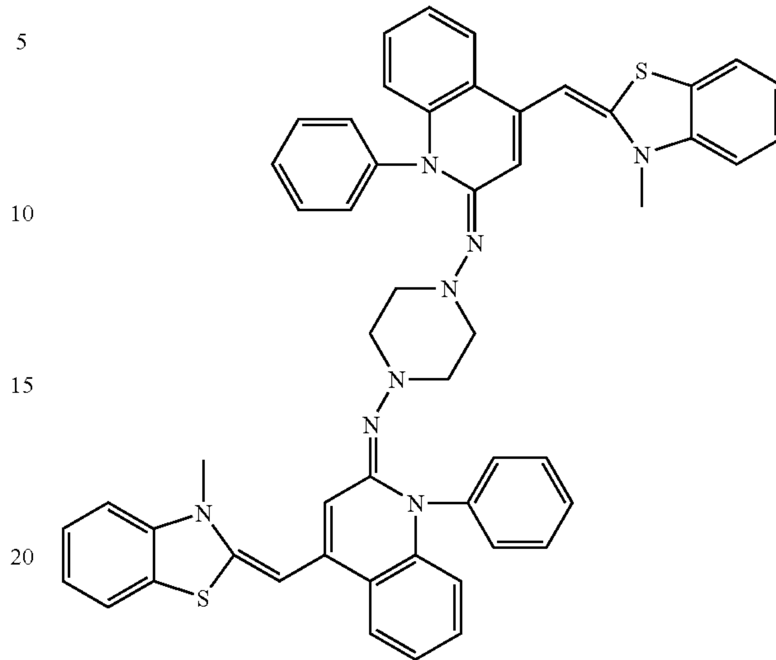
Compound 9
