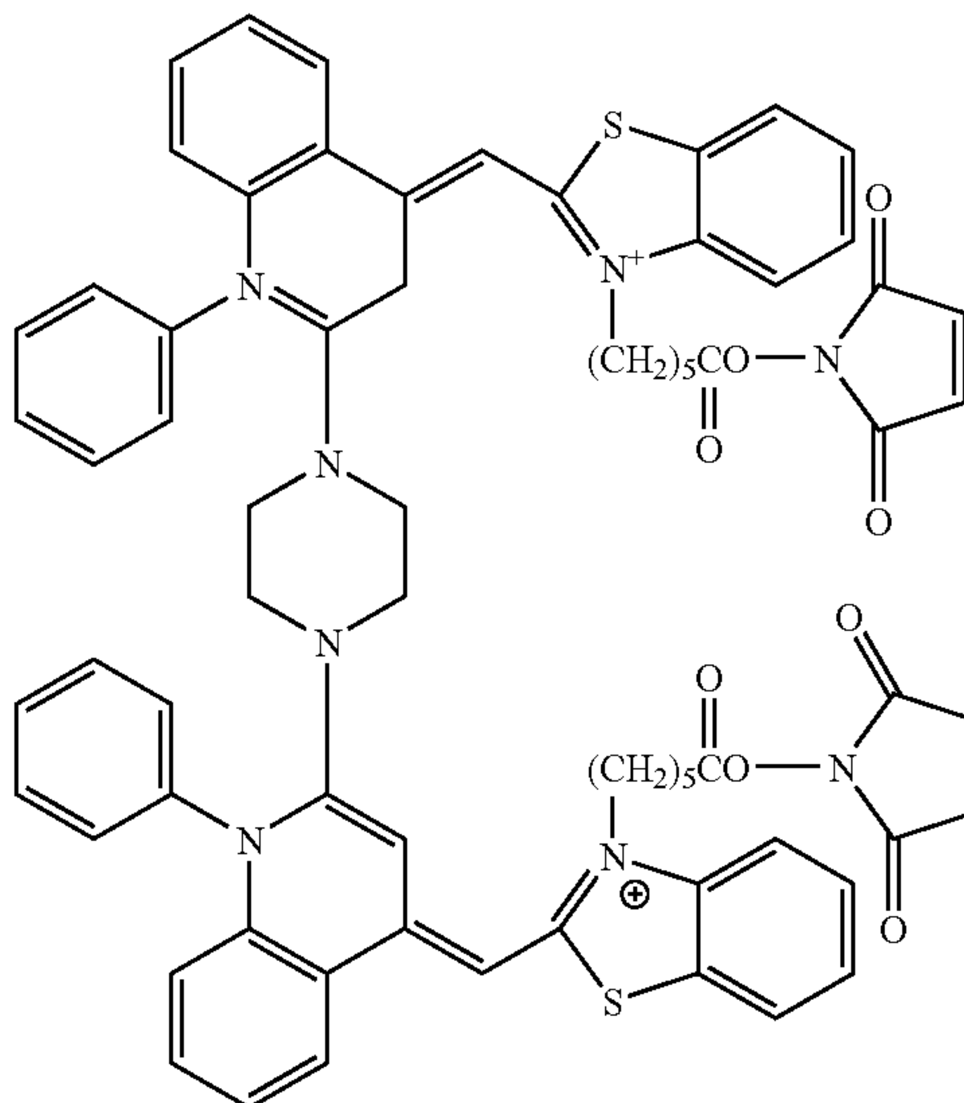
(Compound 33)
