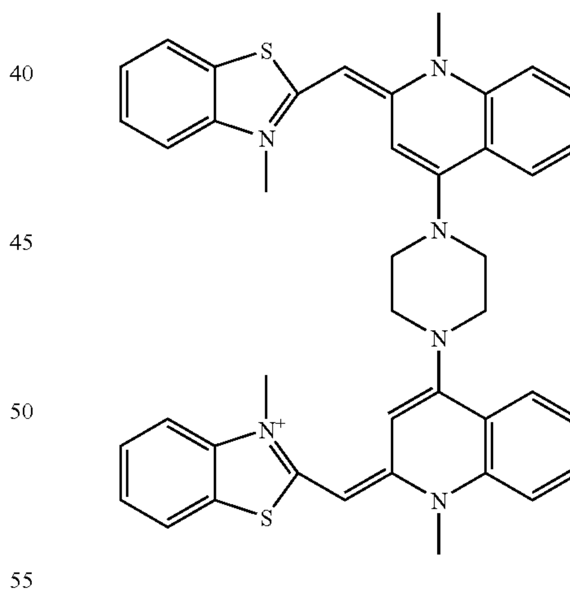
Example 11
