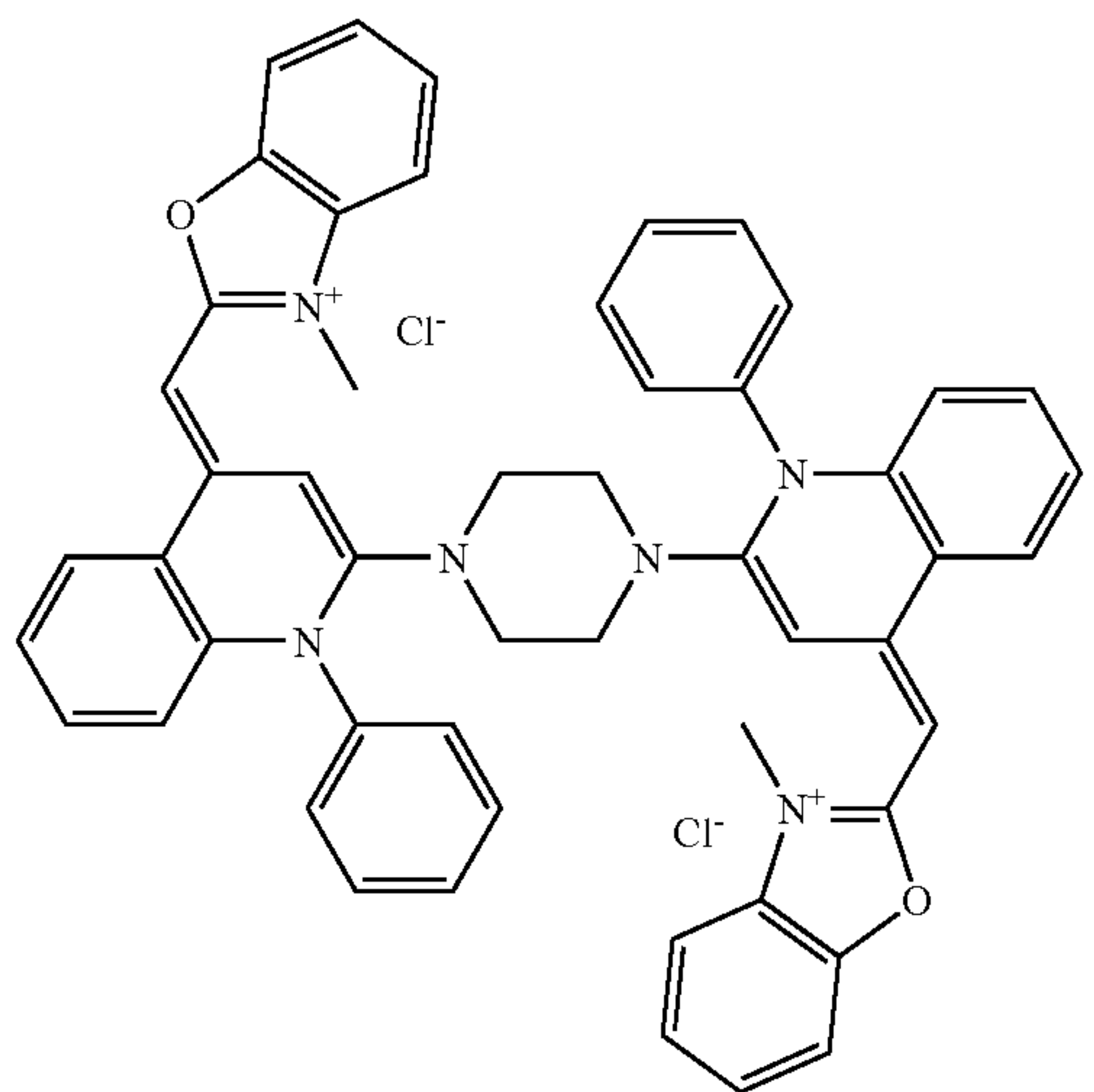
(Compound 20)
