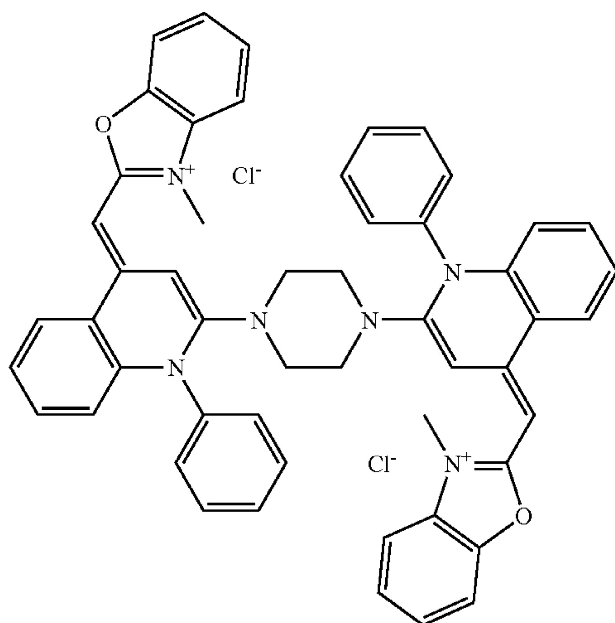
Compound 20
