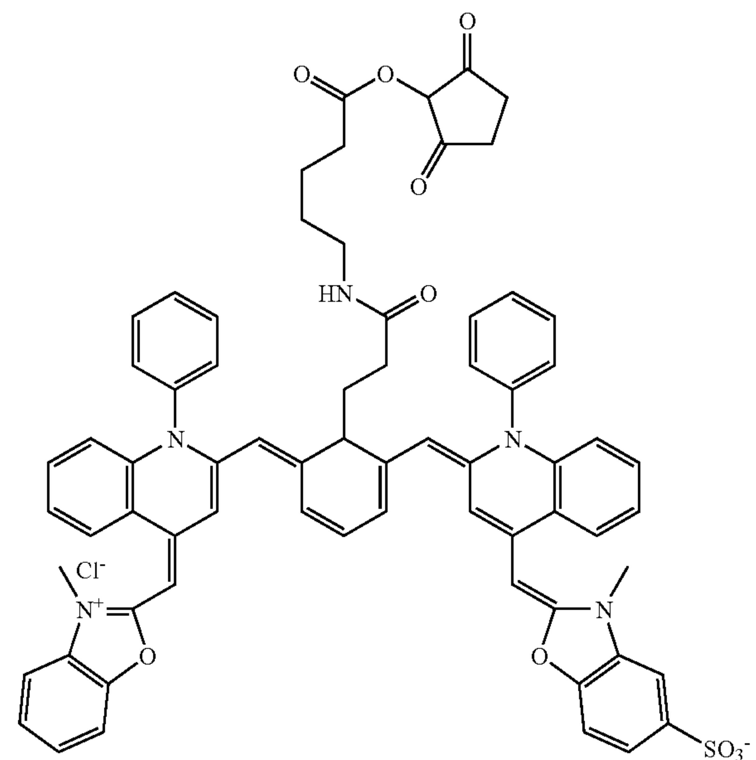
(Compound 27)
