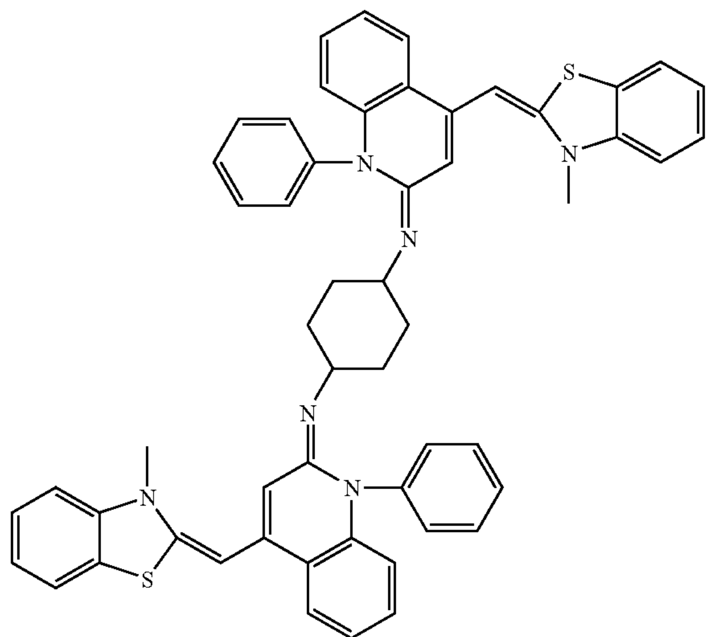
Compound 8
