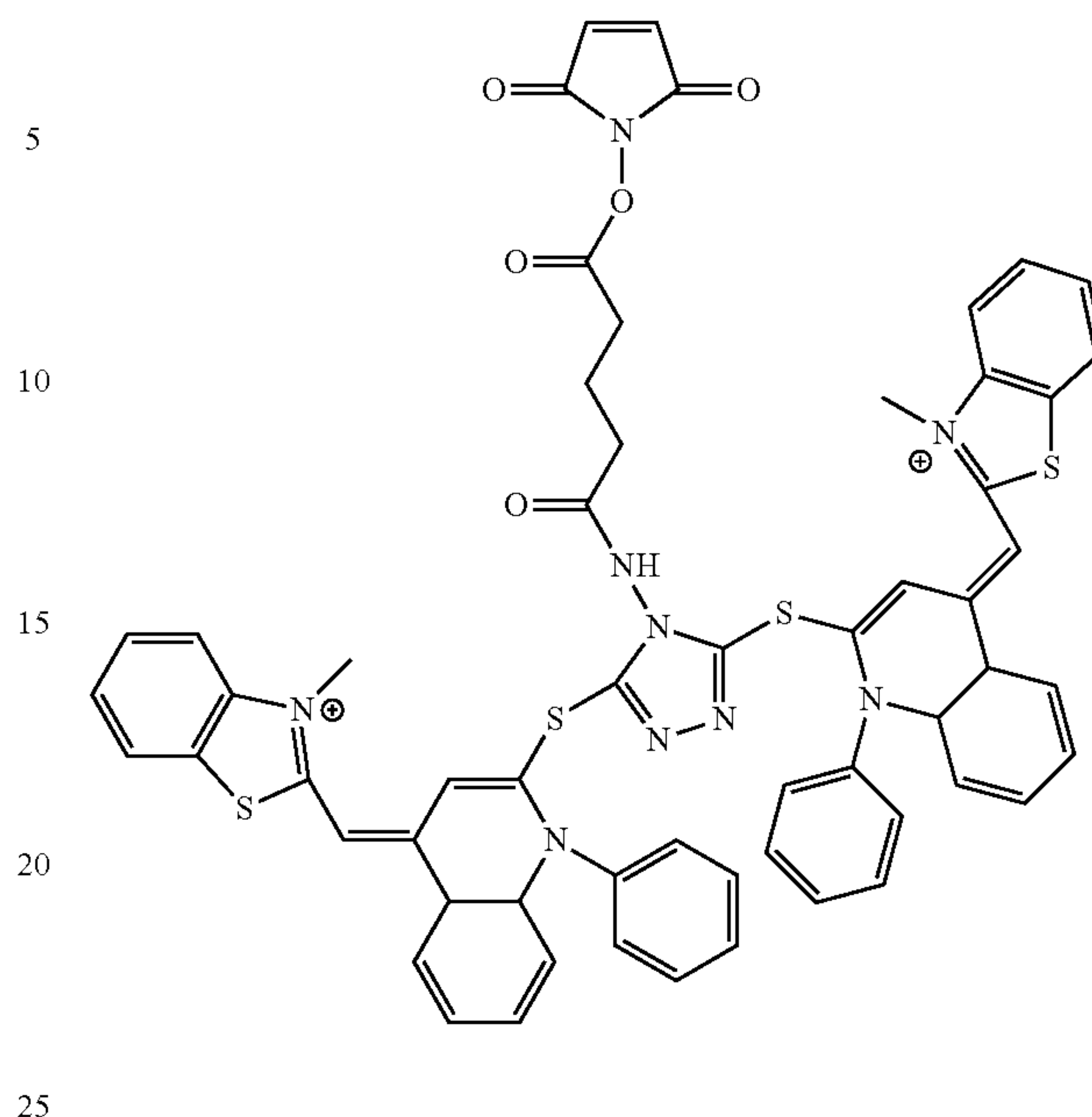
Compound 34
