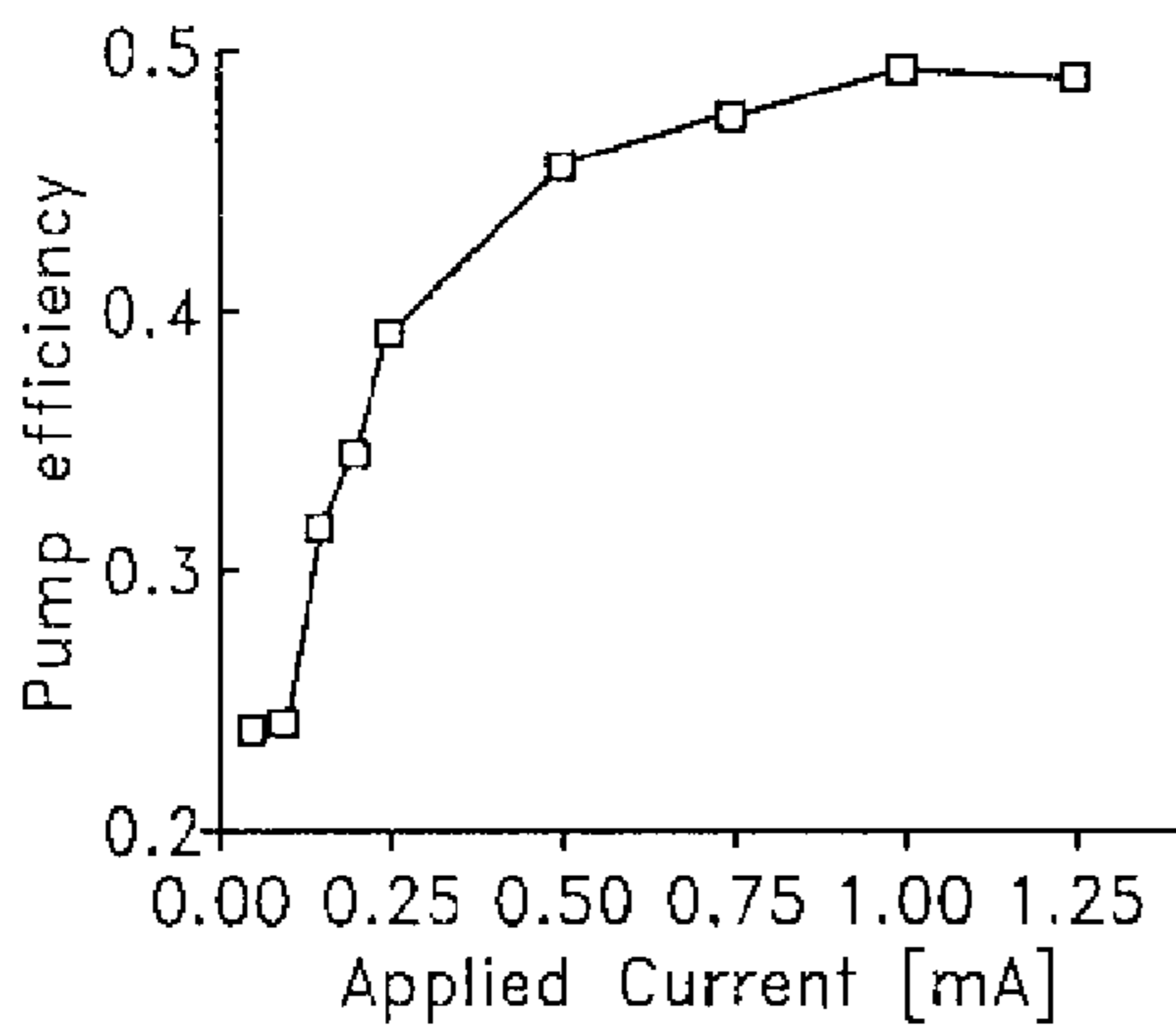
Pump efficiency
