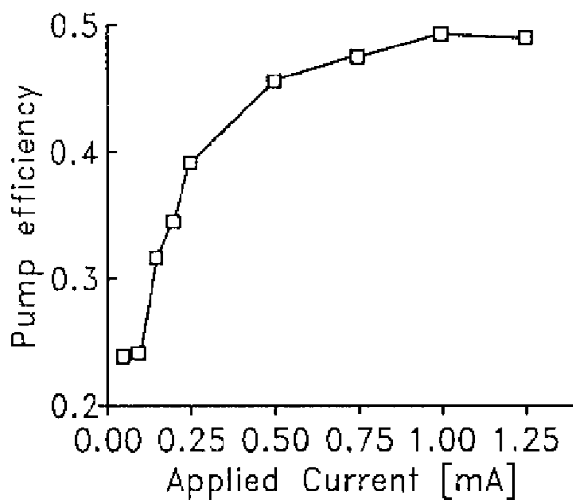
Pump efficiency
